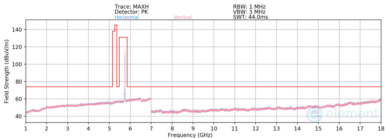
Plot 7-1023. Radiated Spurious Emissions above 1GHz CDD (802.11n – Ch. 149)
