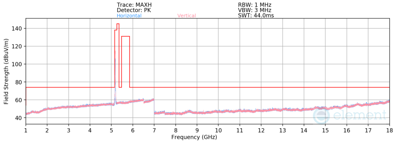
Plot 7-1011. Radiated Spurious Emissions above 1GHz CDD (802.11n – Ch. 36)
