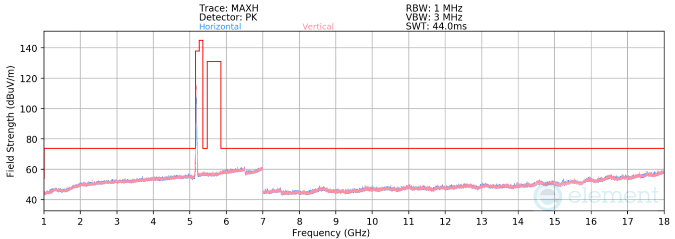
Plot 7-1027. Radiated Spurious Emissions above 1GHz CDD (802.11ax(SU) – Ch. 36)
