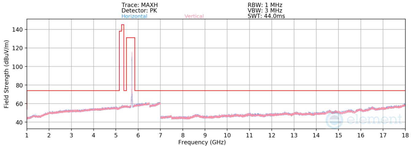
Plot 7-1022. Radiated Spurious Emissions above 1GHz CDD (802.11n – Ch. 144)
