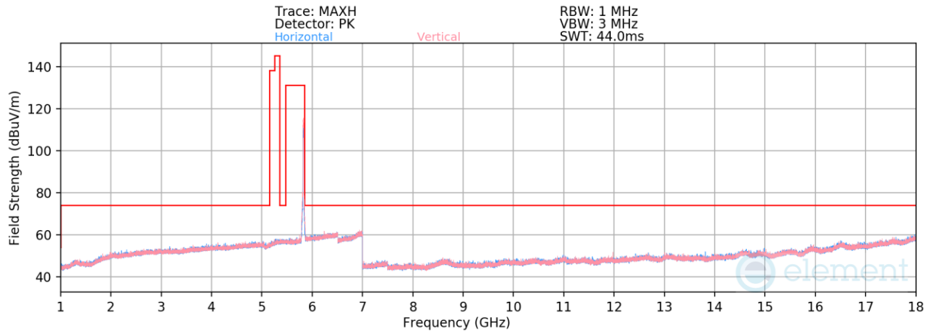
Plot 7-1026. Radiated Spurious Emissions above 1GHz CDD (802.11n – Ch. 165)
