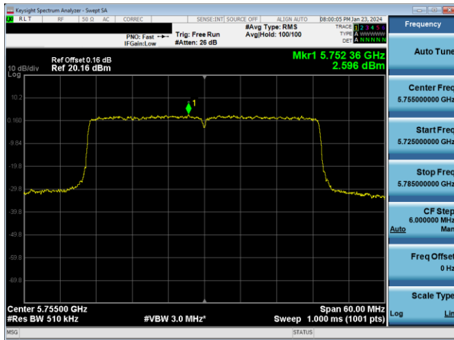
Plot 7-866. PSD CDD DIVERSITY Antenna WF2a (40MHz BW 802.11ac(SU) – Ch. 151, MCS4)
