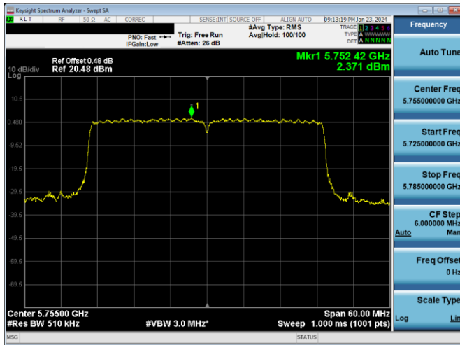
Plot 7-878. PSD CDD DIVERSITY Antenna WF2a (40MHz BW 802.11ac) - Ch. 151, MCS11)
