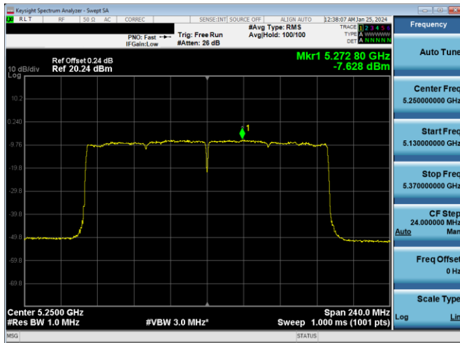
Plot 7-890. ISCED PSD CDD DIVERSITY Antenna WF2a (160MHz BW 11ax (SU) - Ch.50, MCS2)
