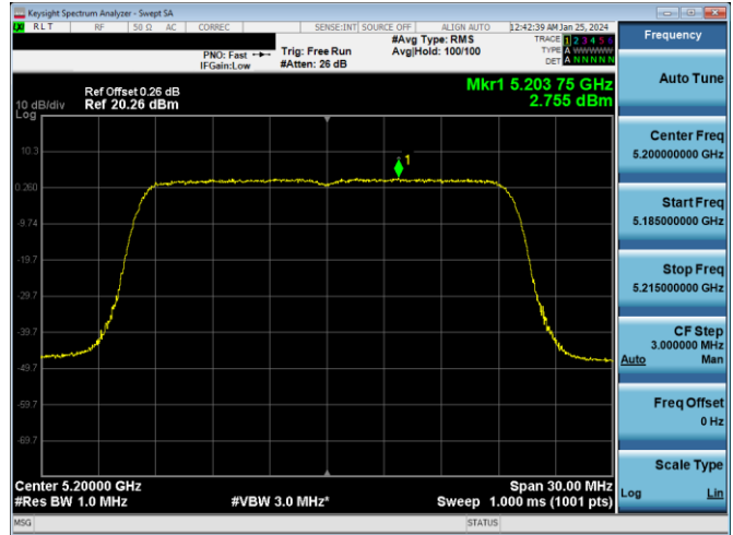
Plot 7-892. ISCED PSD SDM DIVERSITY Antenna WF2a (20MHz BW 11ax(SU) - Ch.40, MCS4)
