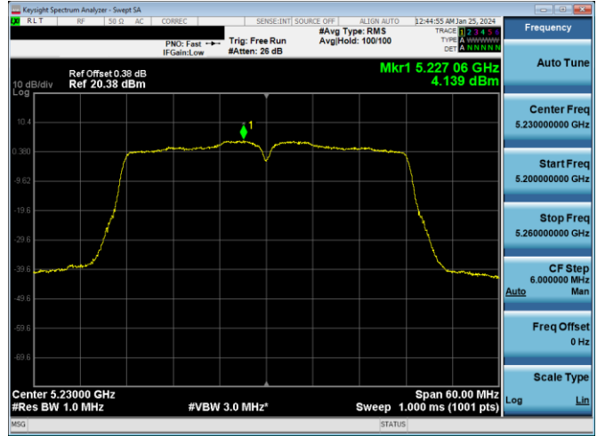
Plot 7-893. ISCED PSD SDM DIVERSITY Antenna WF2a (40MHz BW 11n - Ch.46, MCS12)
