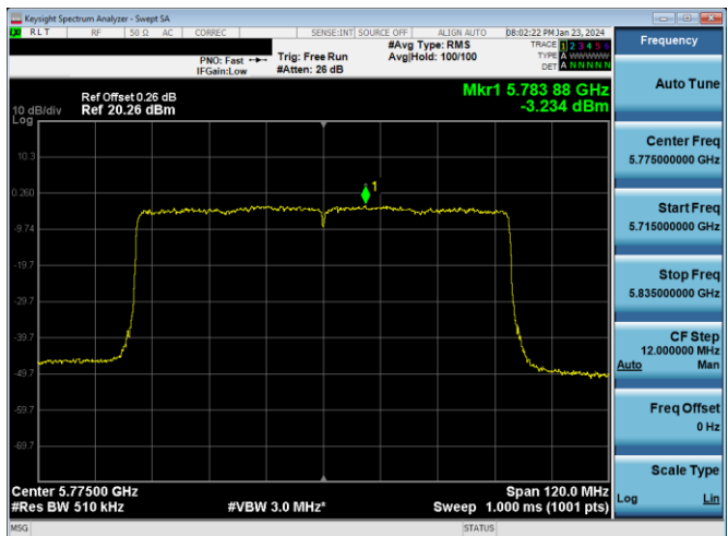
Plot 7-870. PSD CDD DIVERSITY Antenna WF2a (80MHz BW 802.11ac(SU) – Ch. 155, MCS4)
