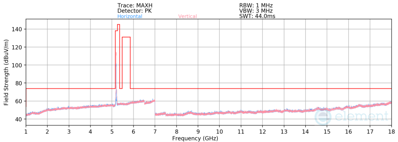
Plot 7-920. Radiated Spurious Emissions above 1GHz Antenna WF7a (802.11ax(SU) – Ch. 40)
