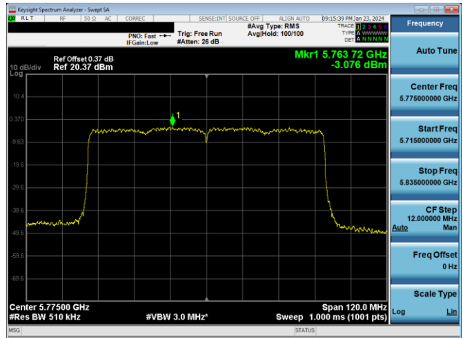
Plot 7-882. PSD CDD DIVERSITY Antenna WF2a (80MHz BW 802.11ac) - Ch. 155, MCS11)
