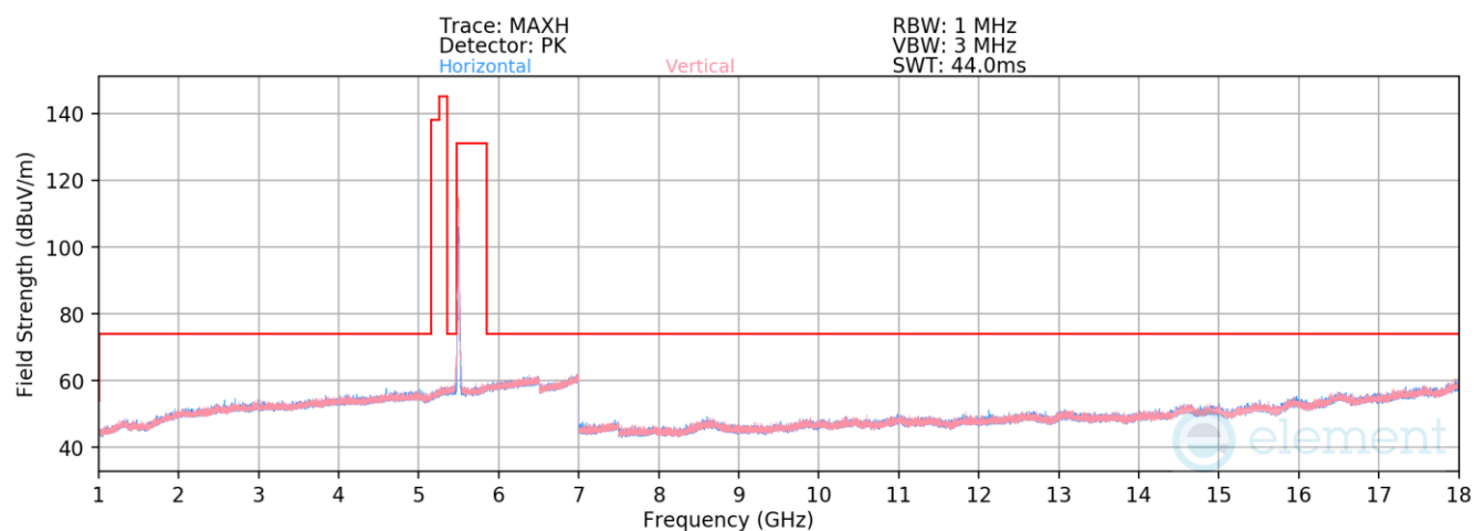
Plot 7-913. Radiated Spurious Emissions above 1GHz Antenna WF7a (802.11n – Ch. 100)
