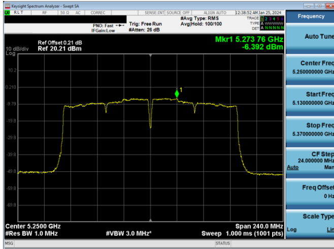
Plot 7-889. ISCED PSD CDD DIVERSITY Antenna WF2a (160MHz BW 11ac - Ch.50, MCS2)
