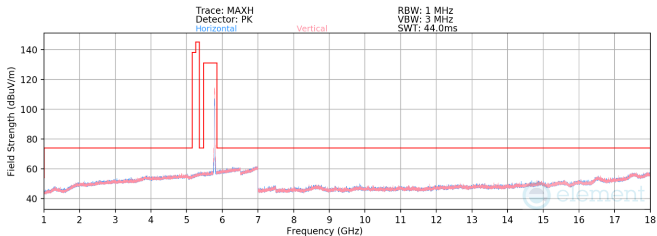
Plot 7-917. Radiated Spurious Emissions above 1GHz Antenna WF7a (802.11n – Ch. 157)
