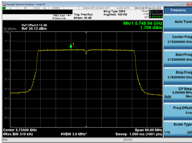
Plot 7-853. PSD CDD DIVERSITY Antenna WF7a (40MHz BW 802.11ac(SU) – Ch. 151, MCS2)
