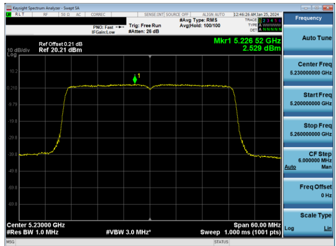
Plot 7-894. ISCED SDM DIVERSITY PSD Antenna WF2a (40MHz BW 11ax(SU) - Ch.46, MCS4)
