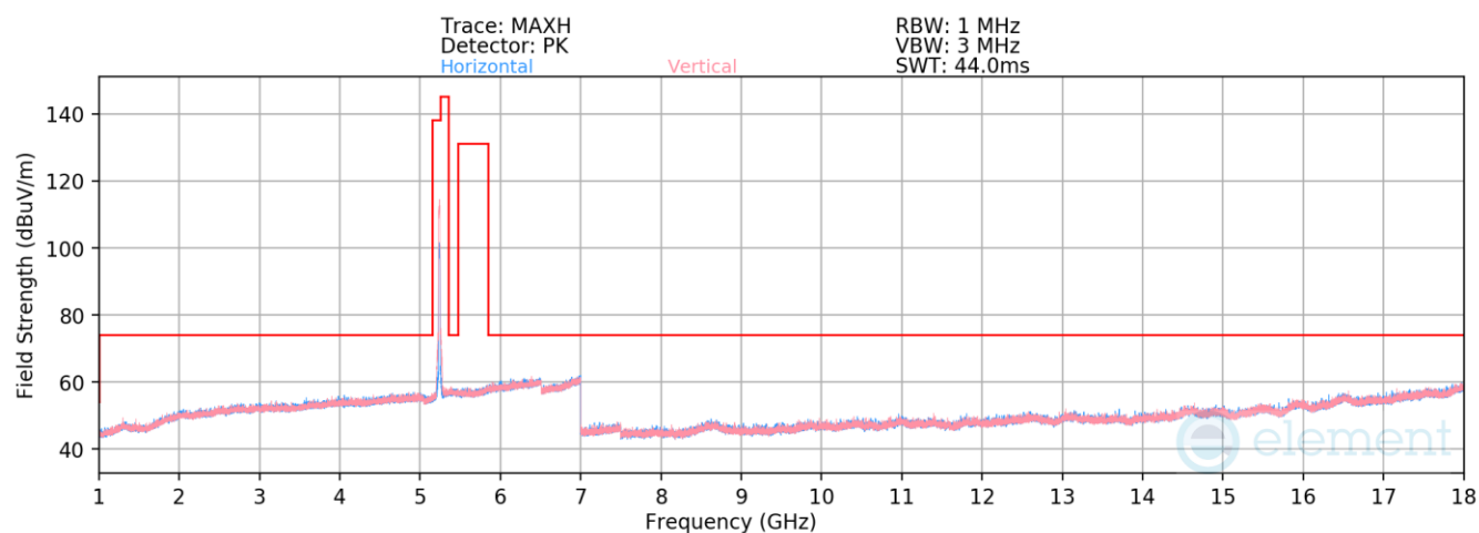
Plot 7-909. Radiated Spurious Emissions above 1GHz Antenna WF7a (802.11n – Ch. 48)
