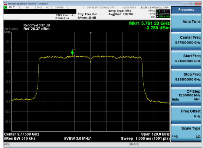
Plot 7-881. PSD CDD DIVERSITY Antenna WF7a (80MHz BW 802.11ac) - Ch. 155, MCS11)
