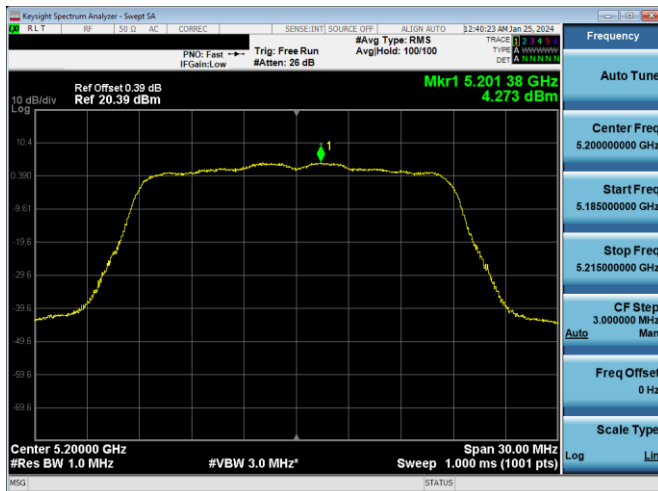
Plot 7-891. ISCED PSD CDD DIVERSITY Antenna WF2a (20MHz BW 11n - Ch.40, MCS12)
