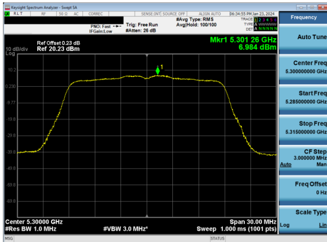
Plot 7-789. PSD CDD DIVERSITY Antenna WF2a (20MHz BW 802.11n – Ch. 60, MCS10)
