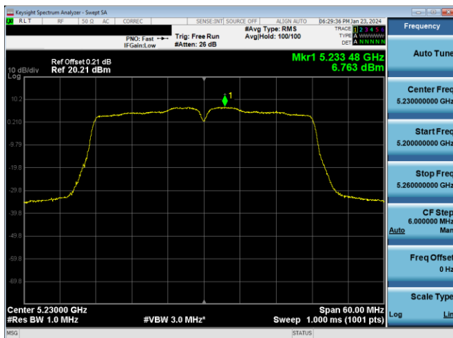
Plot 7-783. PSD CDD DIVERSITY Antenna WF2a (40MHz BW 802.11n – Ch. 46, MCS10)
