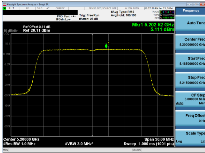
Plot 7-782. PSD CDD DIVERSITY Antenna WF2a (20MHz BW 802.11ax(SU) – Ch. 40, MCS2)
