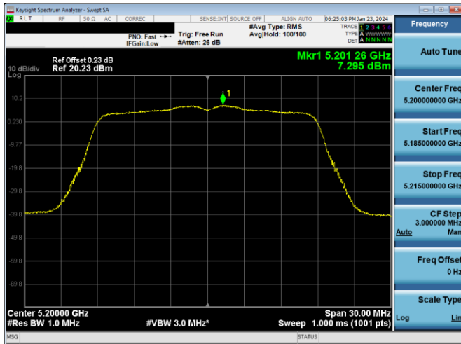
Plot 7-781. PSD CDD DIVERSITY Antenna WF2a (20MHz BW 802.11n – Ch. 40, MCS10)
