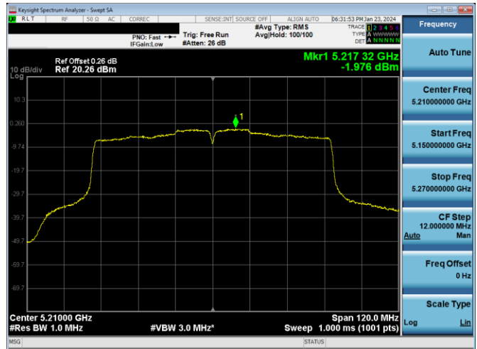
Plot 7-785. PSD CDD DIVERSITY Antenna WF2a (80MHz BW 802.11ac – Ch. 42, MCS2)
