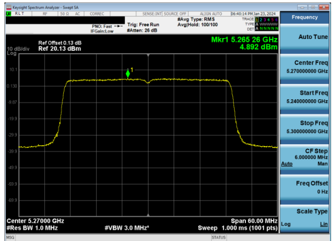
Plot 7-792. PSD CDD DIVERSITY Antenna WF2a (40MHz BW 802.11ax(SU) – Ch. 54, MCS2)
