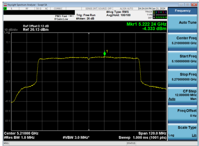
Plot 7-786. PSD CDD DIVERSITY Antenna WF2a (80MHz BW 802.11ax(SU) – Ch. 42, MCS2)
