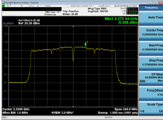
Plot 7-787. PSD CDD DIVERSITY Antenna WF2a (160MHz BW 802.11ac – Ch. 50, MCS2)
