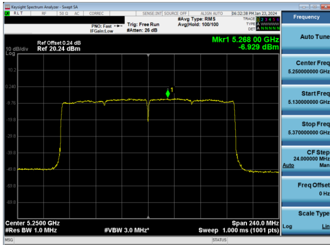
Plot 7-788. PSD CDD DIVERSITY Antenna WF2a (160MHz BW 802.11ax(SU) – Ch. 50, MCS2)
