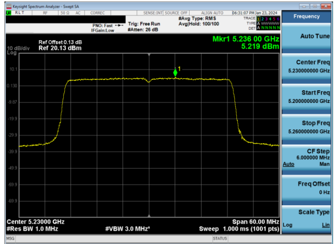
Plot 7-784. PSD CDD DIVERSITY Antenna WF2a (40MHz BW 802.11ax(SU) – Ch. 46, MCS2)
