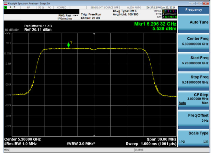
Plot 7-790. PSD CDD DIVERSITY Antenna WF2a (20MHz BW 802.11ax(SU) – Ch. 60, MCS2)
