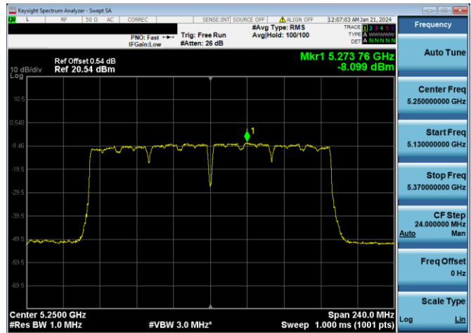
Plot 7-677. PSD CDD PRIMARY Antenna WF7a (160MHz BW 802.11ac - Ch. 50, MCS9)
