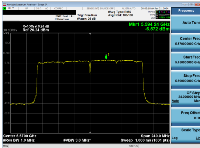
Plot 7-620. PSD CDD PRIMARY Antenna WF2a (160MHz BW 802.11ax(SU) – Ch. 114, MCS2)
