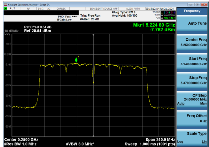
Plot 7-678. PSD CDD PRIMARY Antenna WF2a (160MHz BW 802.11ac - Ch. 50, MCS9)
