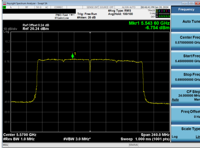
Plot 7-619. PSD CDD PRIMARY Antenna WF7a (160MHz BW 802.11ax(SU) – Ch. 114, MCS2)
