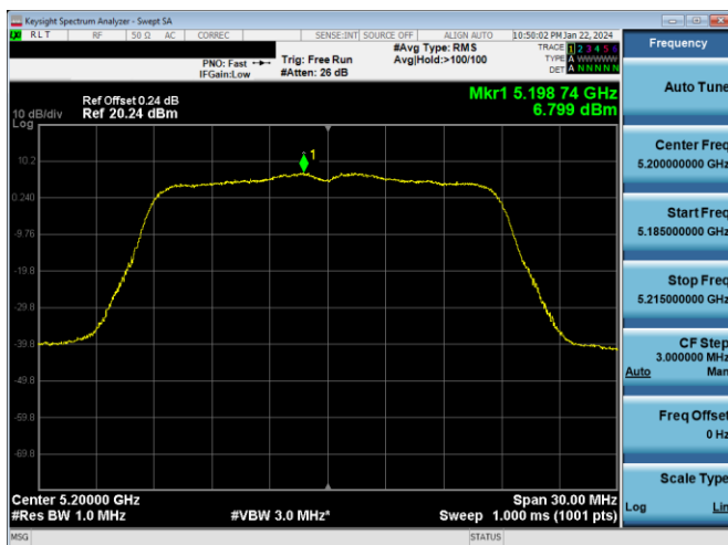
Plot 7-621. PSD CDD PRIMARY Antenna WF7a (20MHz BW 802.11n – Ch. 40, MCS12)
