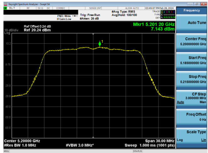
Plot 7-622. PSD CDD PRIMARY Antenna WF2a (20MHz BW 802.11n – Ch. 40, MCS12)
