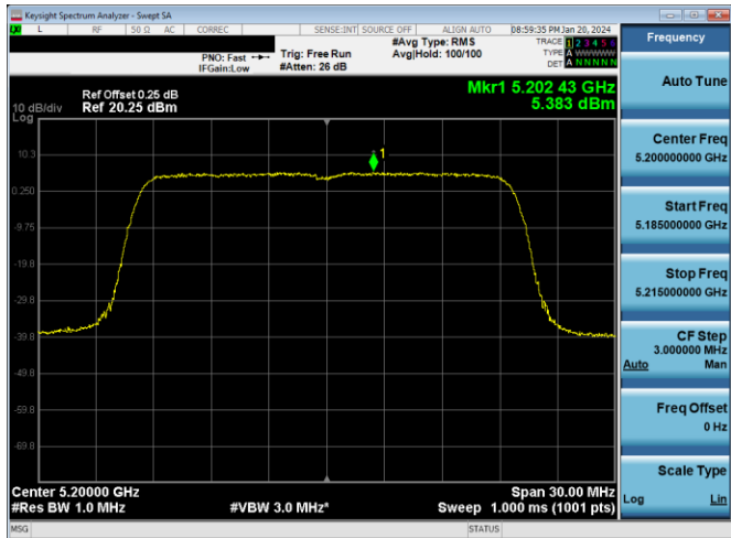
Plot 7-623. PSD CDD PRIMARY Antenna WF7a (20MHz BW 802.11ax(SU) – Ch. 40, MCS4)
