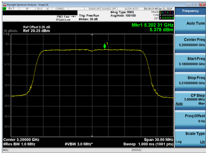
Plot 7-624. PSD CDD PRIMARY Antenna WF2a (20MHz BW 802.11ax(SU) – Ch. 40, MCS4)
