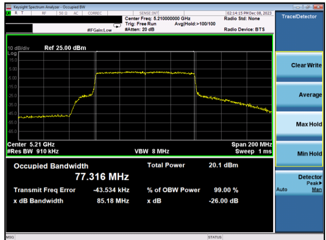
Plot 7-72. 26dB BW & 99% OBW Antenna WF7b (80MHz BW 802.11ax(SU) – Ch. 42, MCS2)
