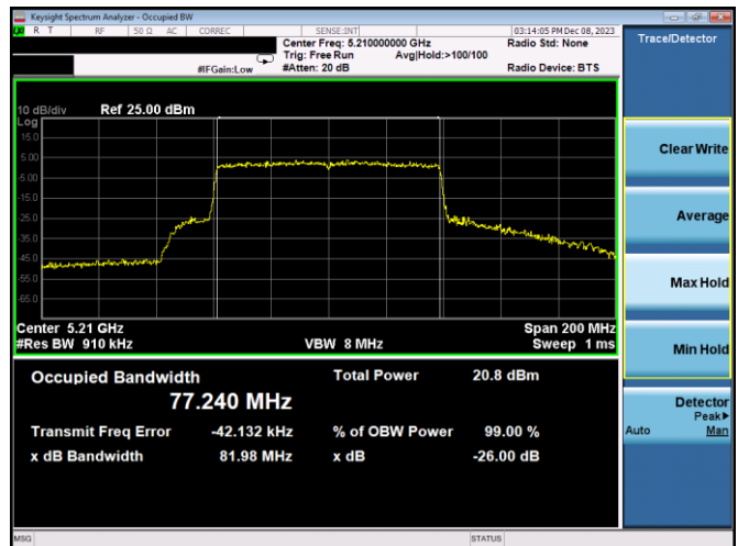
Plot 7-94. 26dB BW & 99% OBW Antenna WF7b (80MHz BW 802.11ax(SU) – Ch. 42, MCS4)
