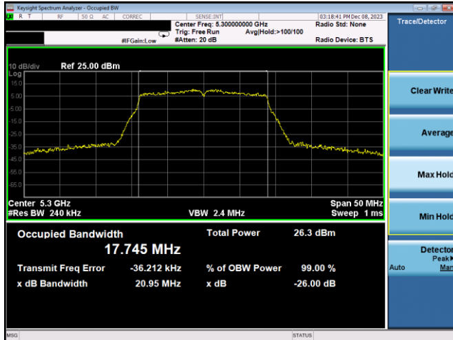
Plot 7-97. 26dB BW & 99% OBW Antenna WF7b (20MHz BW 802.11n – Ch. 60, MCS4)
