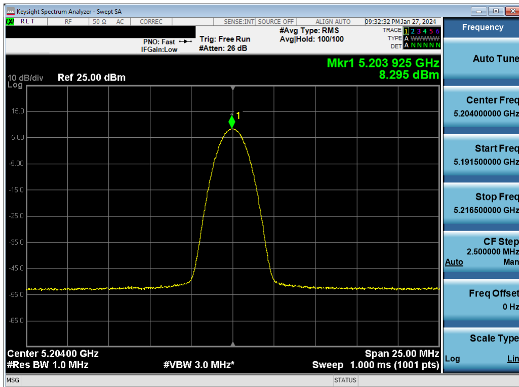
Plot 7-41. ISED PSD Antenna WF2a (BDR GFSK, ePA – 5204MHz)
