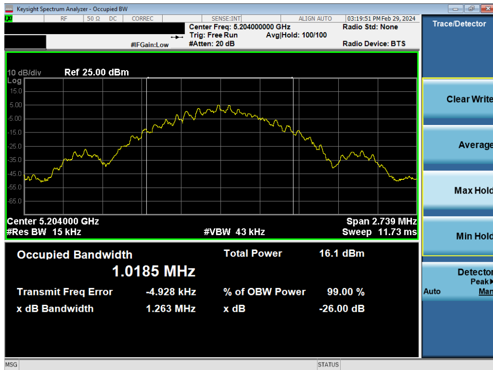
Plot 7-8. 26dB BW & 99% OBW Antenna WF7b (BDR GFSK, ePA- 5204MHz)
