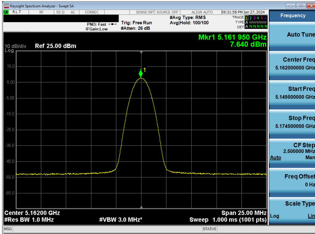
Plot 7-40. ISED PSD Antenna WF2a (BDR GFSK, ePA – 5162MHz)
