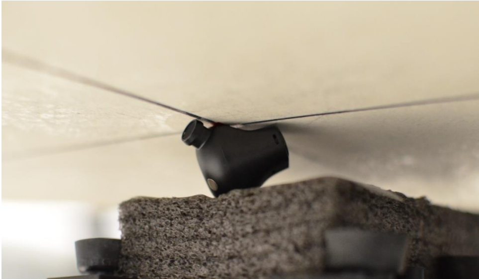
SAR Test Setup Photo 1: Head, Left Earbud, 0 mm
