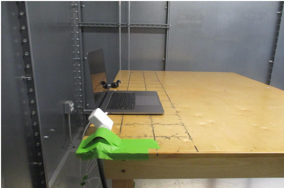
Figure 16: AC Line Test Setup (Side View)
