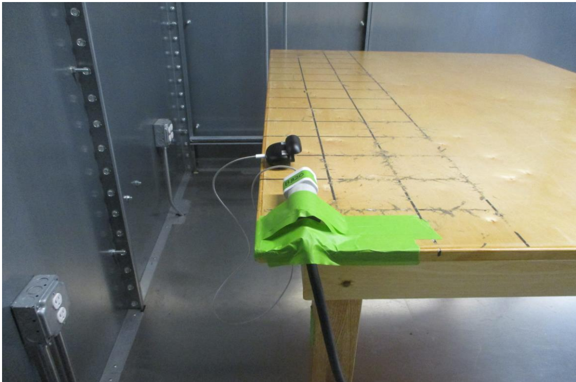
Figure 14: AC Line Test Setup (Side View)
