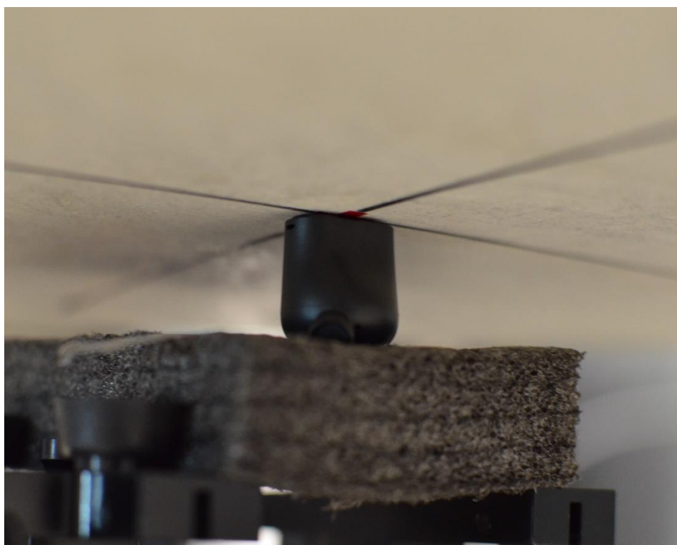
SAR Test Setup Photo 2: Body-Worn, Back Side, 0 mm
