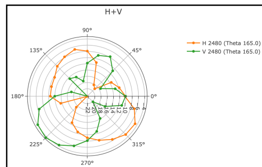
f = 2480 MHz
