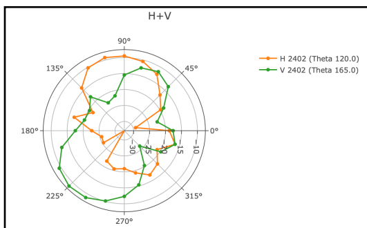
f = 2402 MHz
