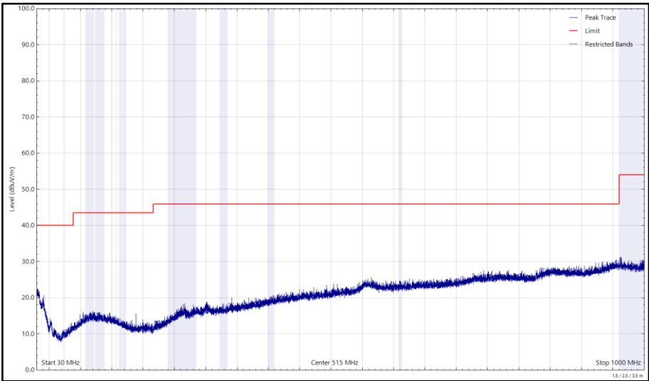
Figure 288 - U-NII-1 - 5180 MHz (CH36), 802.11a, Core 0, 30 MHz to 1 GHz, Vertical (Peak)
