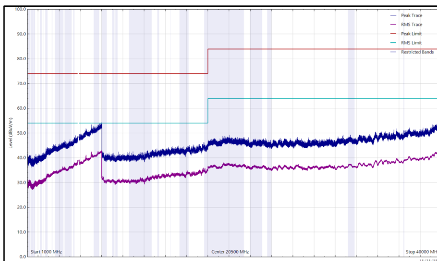
Figure 285 - U-NII-3 - 5825 MHz (CH165), VHT20, CDD, Core 0 + Core 1, 1 GHz to 40 GHz, Vertical
