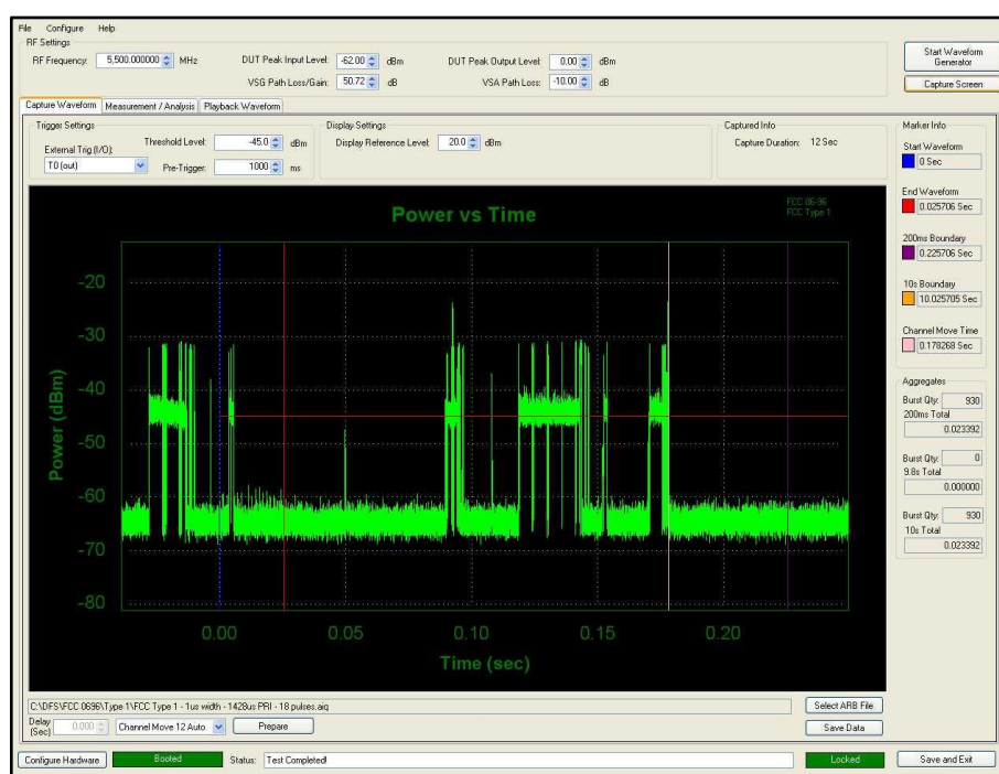
Figure 339 First 200 ms of Channel Shutdown Period
