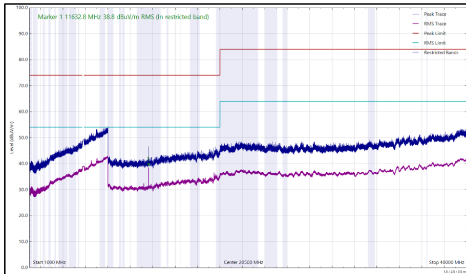
Figure 328 - U-NII-3 - 5825 MHz (CH165), HE20, RU26-0, CDD, Core 0 + Core 1, 1 GHz to 40 GHz, Horizontal
