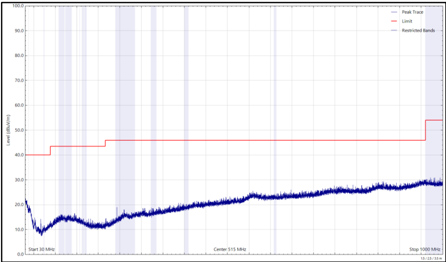
Figure 326 - U-NII-3 - 5825 MHz (CH165), 802.11a, Core 1, 30 MHz to 1 GHz, Vertical (Peak)
