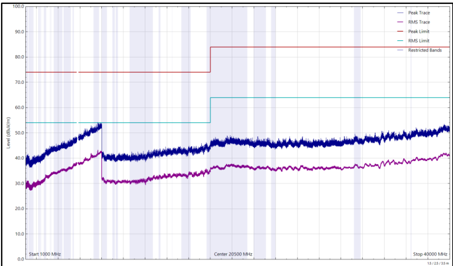
Figure 283 - U-NII-3 - 5745 MHz (CH149), VHT20, CDD, Core 0 + Core 1, 1 GHz to 40 GHz, Vertical
