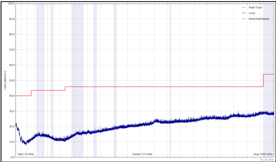
Figure 322 - U-NII-3 - 5825 MHz (CH165), 802.11a, Core 0, 30 MHz to 1 GHz, Vertical (Peak)
