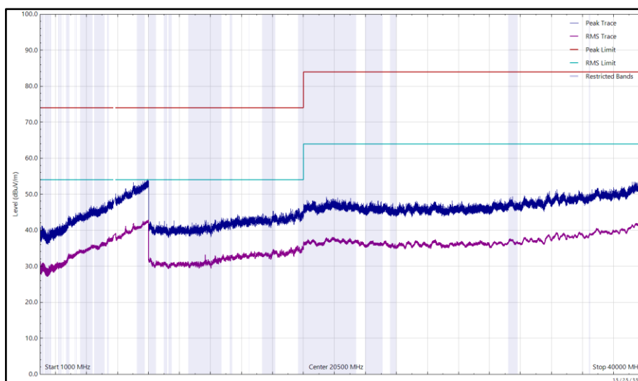
Figure 284 - U-NII-3 - 5825 MHz (CH165), VHT20, CDD, Core 0 + Core 1, 1 GHz to 40 GHz, Horizontal
