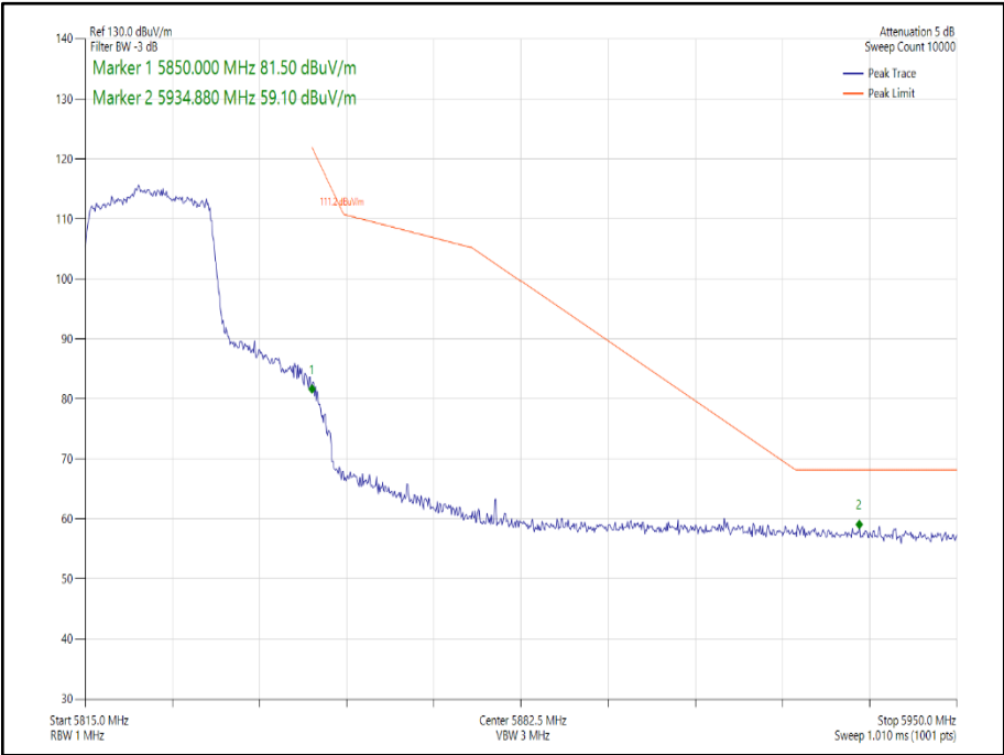
Figure 199 - - 802.11ax HE20 SDM, Cores 0-1, SU - 5825 MHz Band Edge Frequency 5850 MHz
