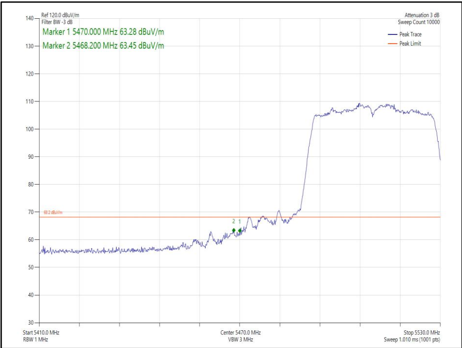
Figure 214 - 802.11n HT40 SDM, Cores 0-1 - 5510 MHz Band Edge Frequency 5470 MHz
