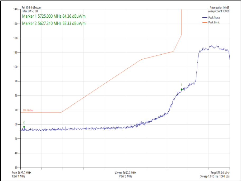
Figure 193 - - 802.11ax HE20 SDM, Cores 0-1, SU - 5745 MHz Band Edge Frequency 5725 MHz
