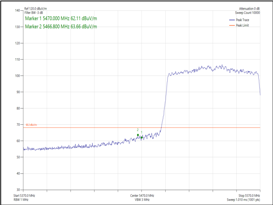
Figure 249 - 802.11ac VHT80 CDD, Cores 0-1 - 5530 MHz Band Edge Frequency 5470 MHz
