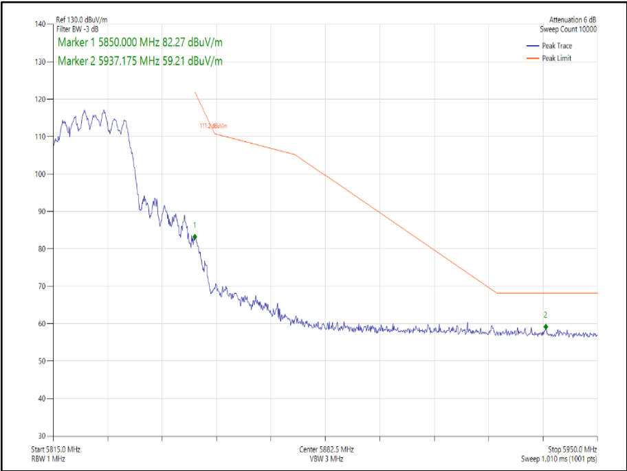
Figure 197 - - 802.11ax HE20 CDD, Cores 0-1, SU - 5825 MHz Band Edge Frequency 5850 MHz
