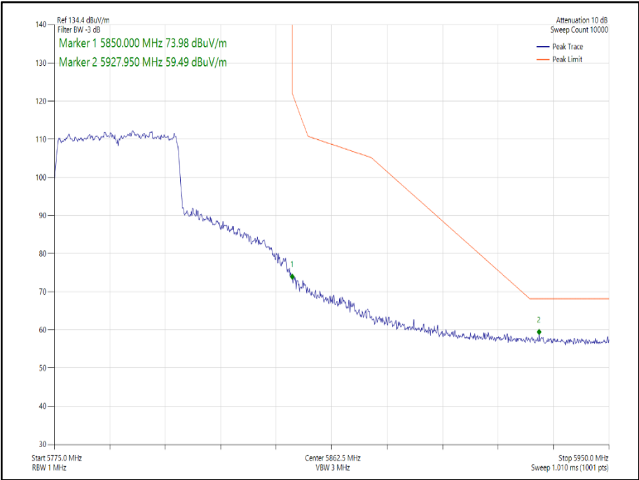
Figure 235 - 802.11ax HE40 SDM, Cores 0-1, SU - 5795 MHz Band Edge Frequency 5850 MHz
