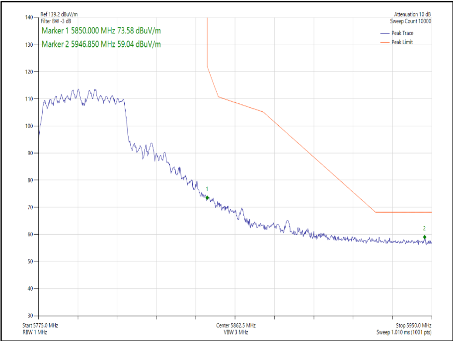
Figure 231 - 802.11n HT40 CDD, Cores 0-1 - 5795 MHz Band Edge Frequency 5850 MHz
