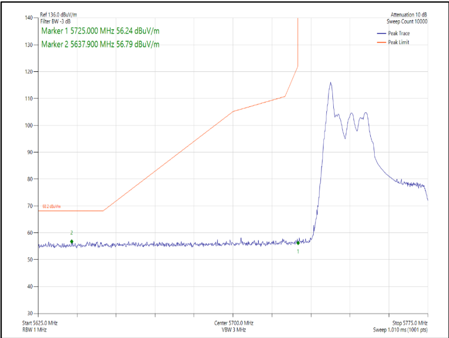
Figure 230 - 802.11ax HE40 SDM, Cores 0-1, 26-0 - 5755 MHz Band Edge Frequency 5725 MHz
