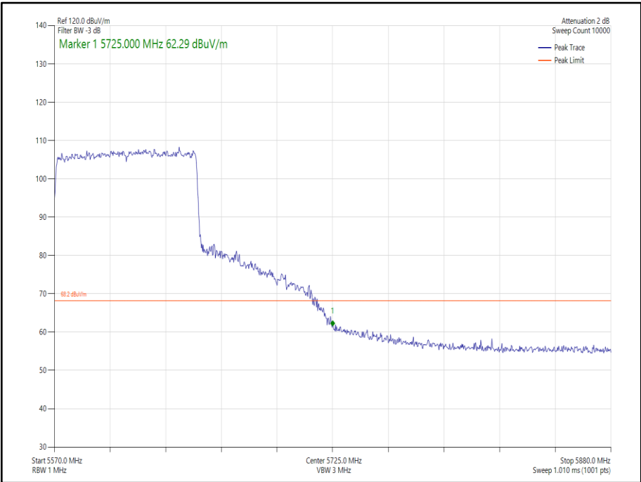
Figure 241 - 802.11ax HE80 Core 1 SU - 5610 MHz Band Edge Frequency 5725 MHz
