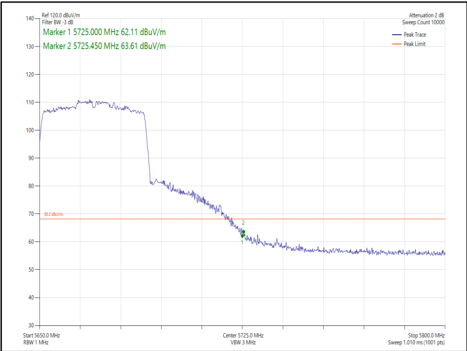
Figure 205 - 802.11ax HE40, Core 1, SU - 5670 MHz Band Edge Frequency 5725 MHz
