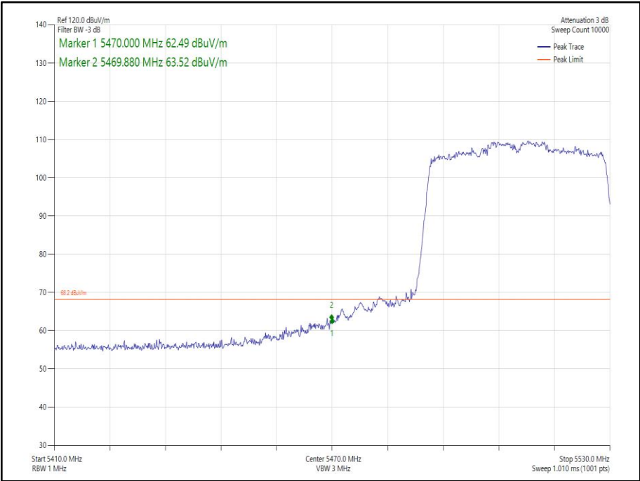
Figure 217 - 802.11ax HE40 SDM, Cores 0-1, SU - 5510 MHz Band Edge Frequency 5470 MHz
