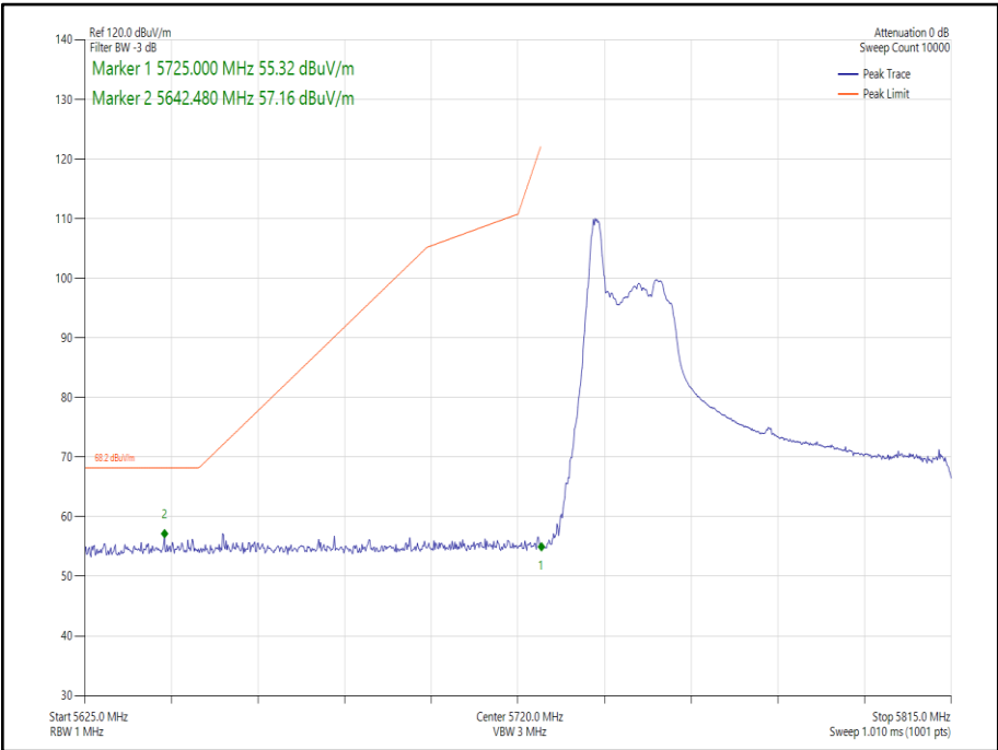
Figure 245 - 802.11ax HE80 Core 0 26-0 - 5775 MHz Band Edge Frequency 5725 MHz
