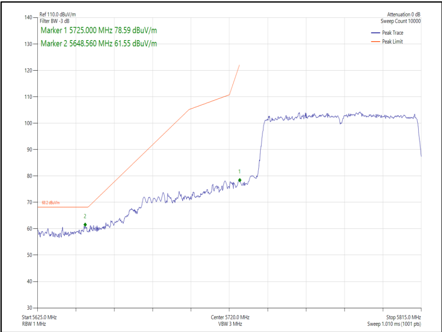
Figure 243 - 802.11ac VHT80 Core 0 - 5775 MHz Band Edge Frequency 5725 MHz
