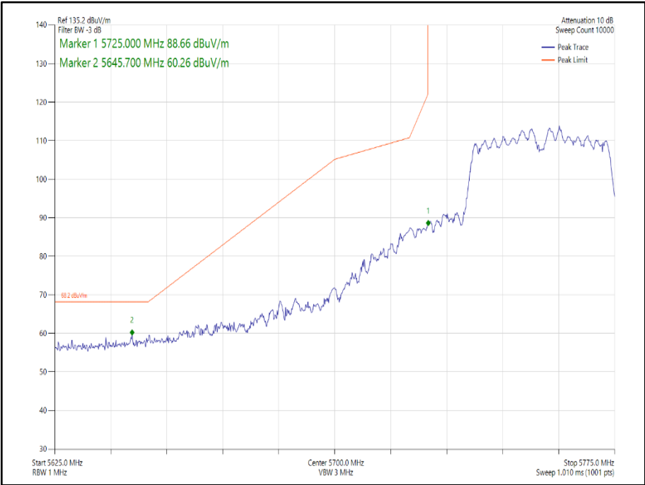
Figure 225 - 802.11n HT40 CDD, Cores 0-1 - 5755 MHz Band Edge Frequency 5725 MHz
