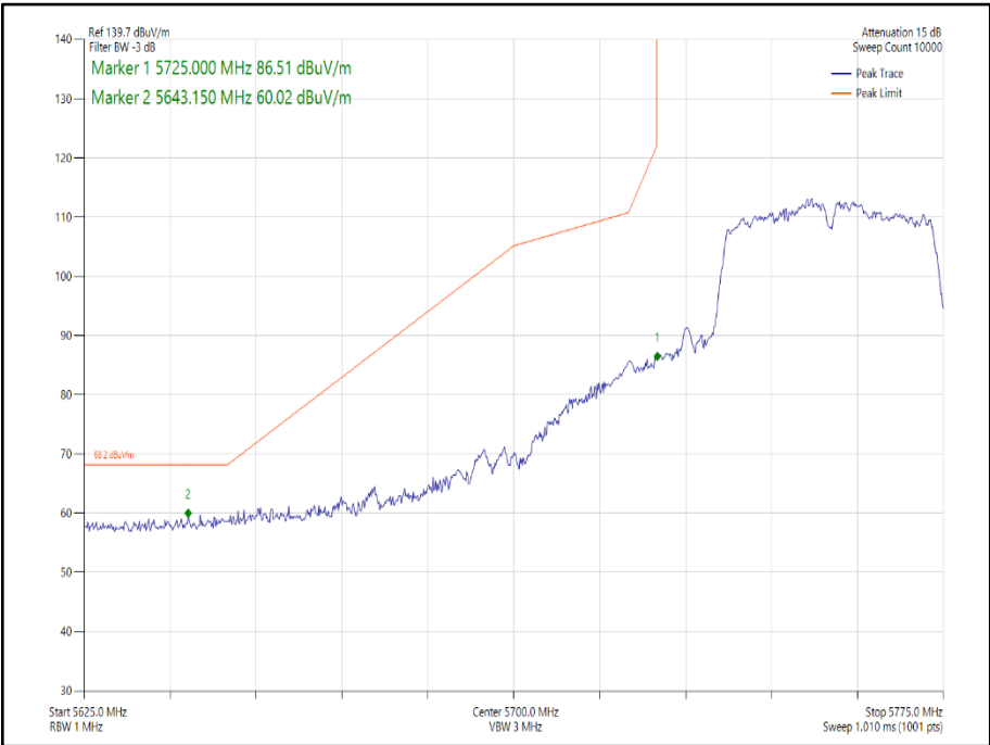
Figure 226 - 802.11n HT40 SDM, Cores 0-1 - 5755 MHz Band Edge Frequency 5725 MHz
