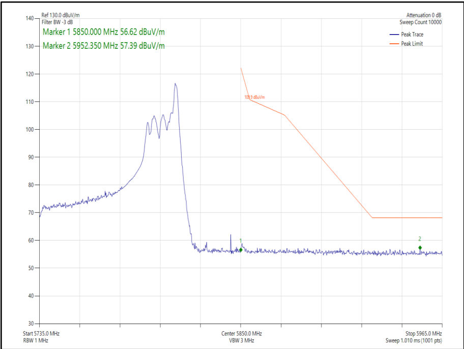
Figure 272 - 802.11ax HE80 SDM, Cores 0-1, 26-36 - 5775 MHz Band Edge Frequency 5850 MHz
