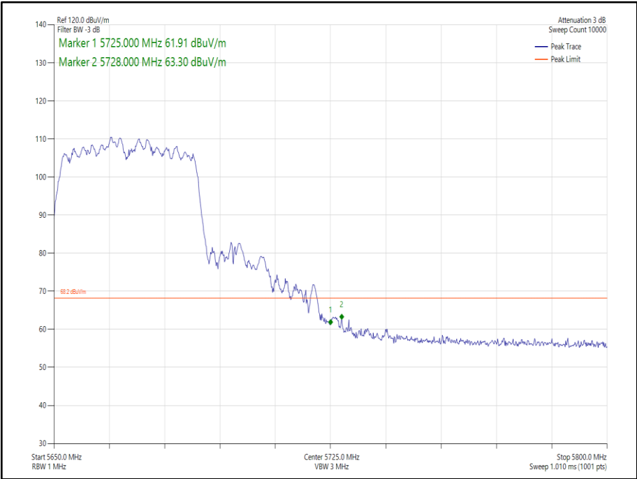
Figure 219 - 802.11n HT40 CDD, Cores 0-1 - 5670 MHz Band Edge Frequency 5725 MHz
