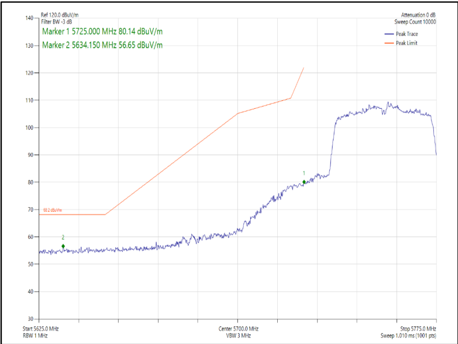
Figure 207 - 802.11n HT40, Core 0 - 5755 MHz Band Edge Frequency 5725 MHz
