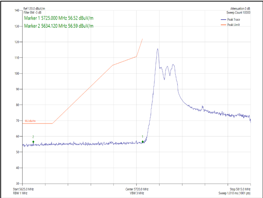
Figure 264 - 802.11ax HE80 CDD, Cores 0-1, 26-0 - 5775 MHz Band Edge Frequency 5725 MHz
