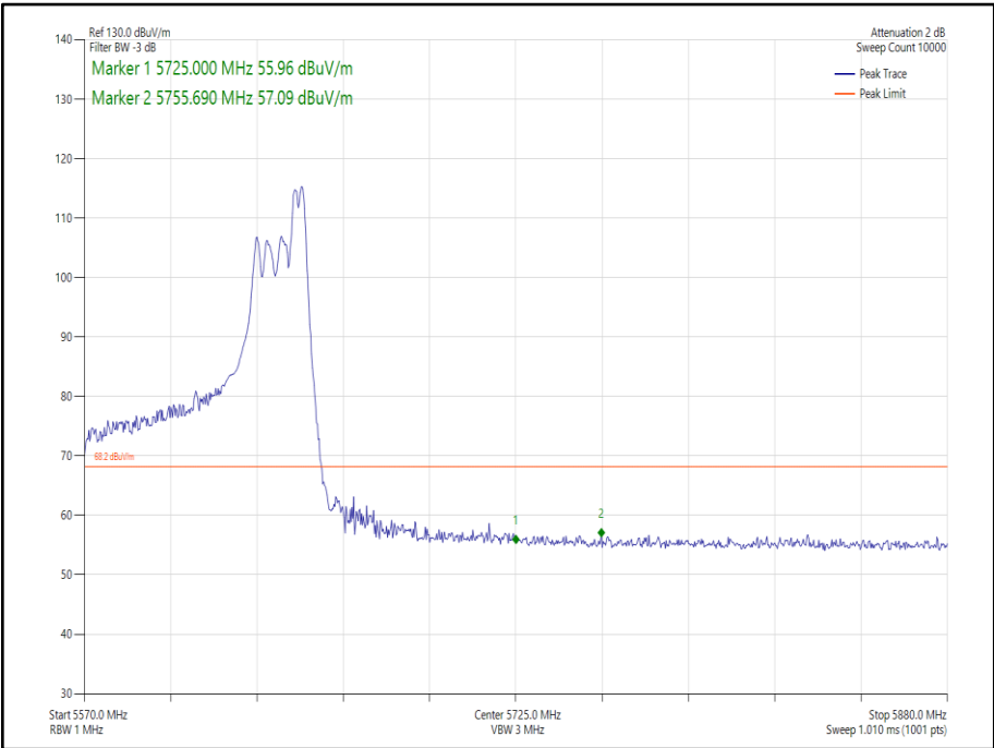
Figure 258 - 802.11ax HE80 CDD, Cores 0-1, 52-52- 5610 MHz Band Edge Frequency 5725 MHz
