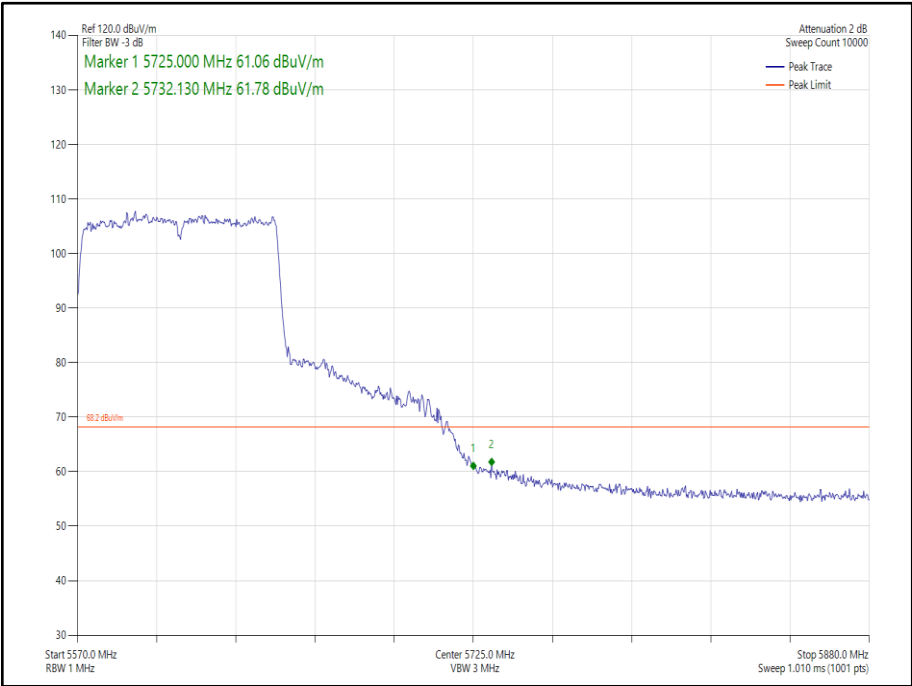
Figure 240 - 802.11ac VHT80 Core 1 - 5610 MHz Band Edge Frequency 5725 MHz
