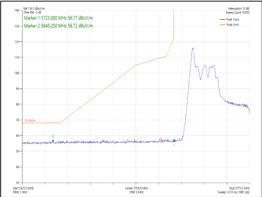
Figure 228 - 802.11ax HE40 CDD, Cores 0-1, 26-0 - 5755 MHz Band Edge Frequency 5725 MHz
