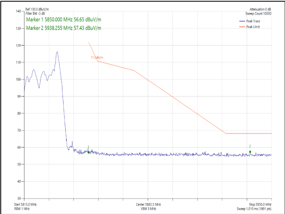
Figure 200 - 802.11ax HE20 SDM, Cores 0-1, 26-8 - 5825 MHz Band Edge Frequency 5850 MHz
