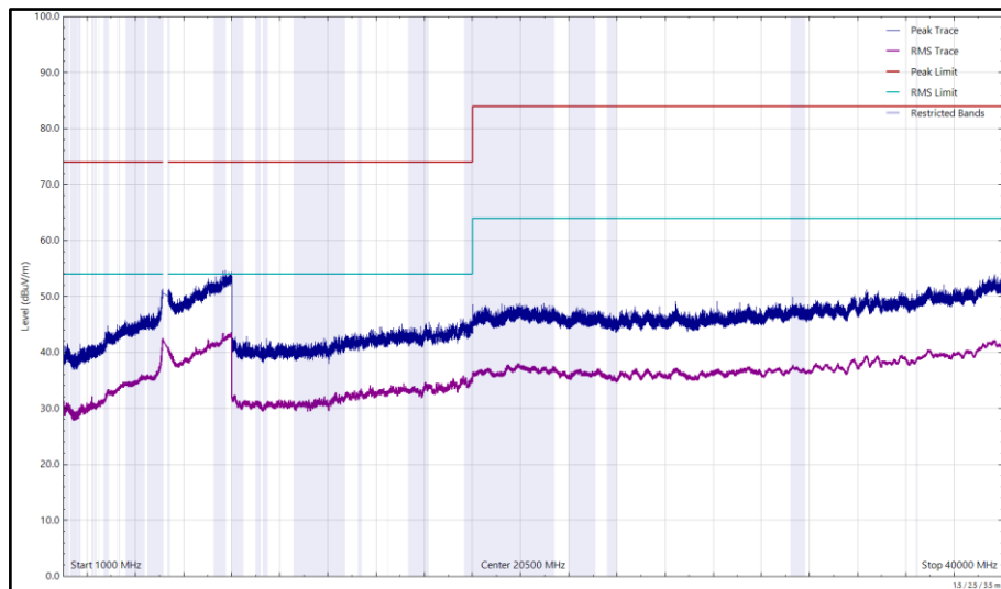
Figure 274 - U-NII-1 - 5180 MHz (CH36), VHT20, CDD, Core 0 + Core 1, 1 GHz to 40 GHz, Horizontal
