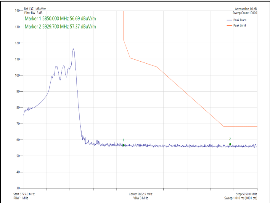
Figure 236 - 802.11ax HE40 SDM, Cores 0-1, 26-17 - 5795 MHz Band Edge Frequency 5850 MHz
