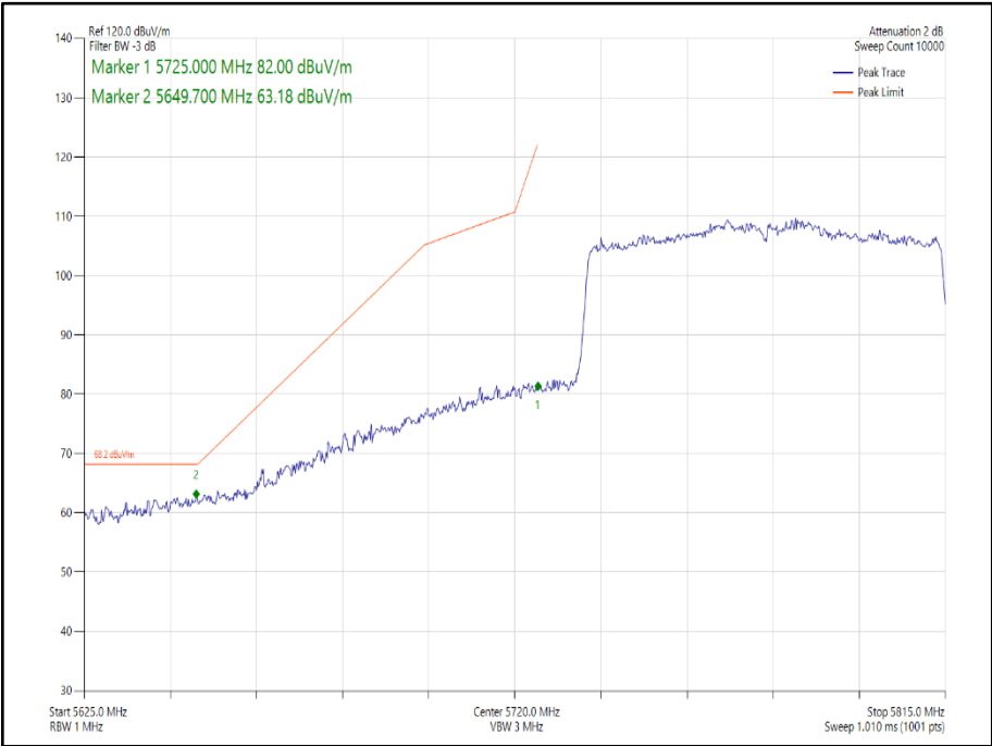
Figure 265 - 802.11ax HE80 SDM, Cores 0-1, SU - 5775 MHz Band Edge Frequency 5725 MHz
