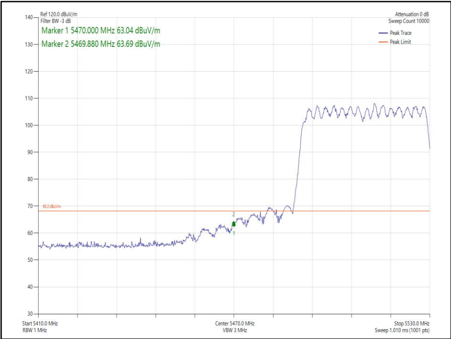
Figure 215 - 802.11ax HE40 CDD, Cores 0-1, SU - 5510 MHz Band Edge Frequency 5470 MHz
