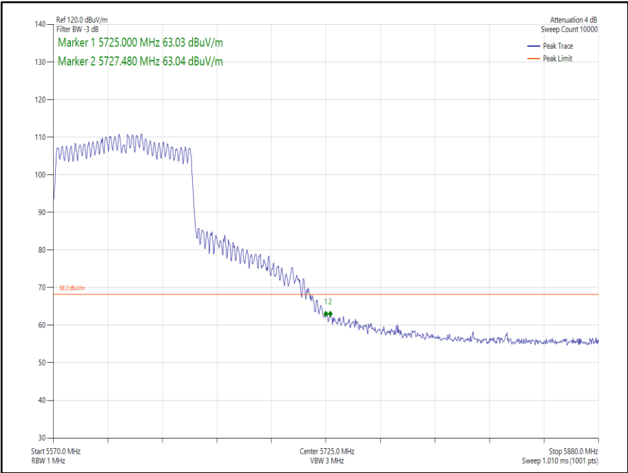
Figure 257 - 802.11ax HE80 CDD, Cores 0-1, SU - 5610 MHz Band Edge Frequency 5725 MHz
