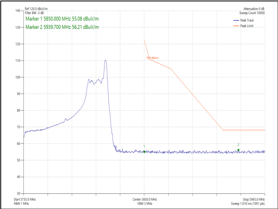
Figure 248 - 802.11ax HE80 Core 0 26-36 - 5775 MHz Band Edge Frequency 5850 MHz
