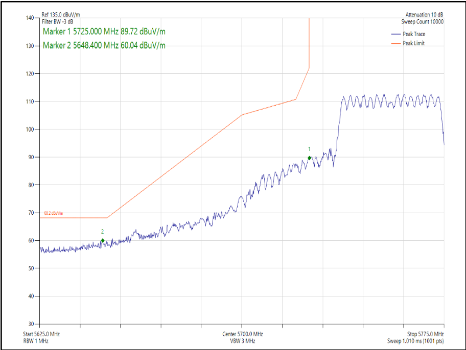
Figure 227 - 802.11ax HE40 CDD, Cores 0-1, SU - 5755 MHz Band Edge Frequency 5725 MHz
