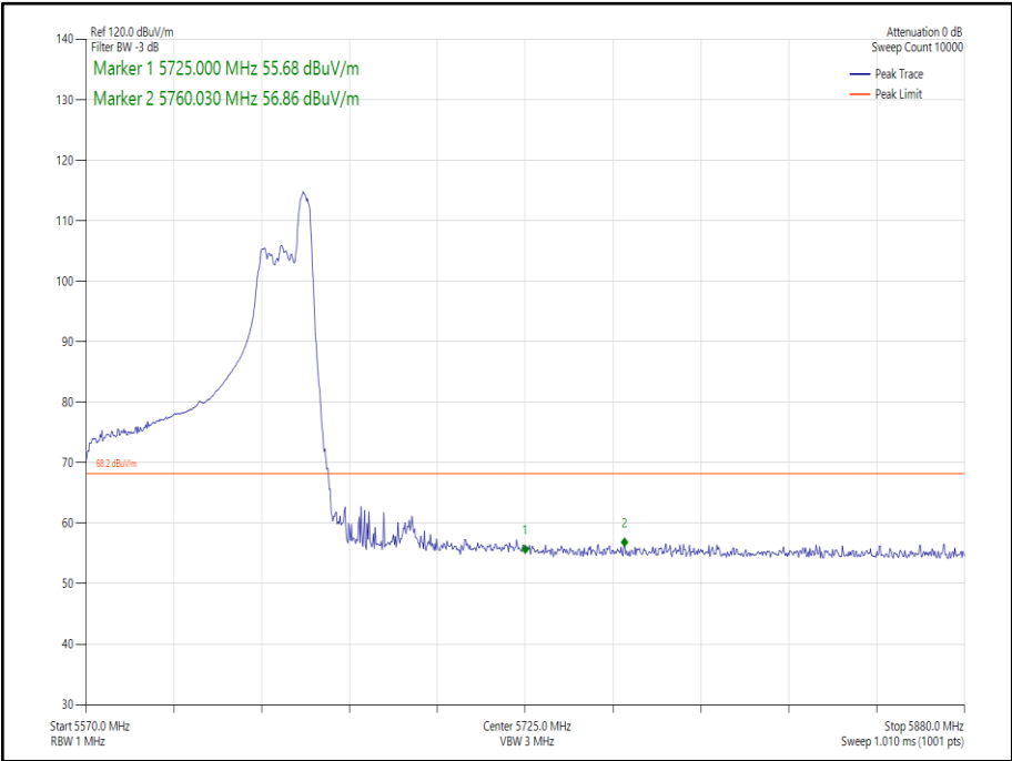
Figure 242 - 802.11ax HE80 Core 1 52-52 - 5610 MHz Band Edge Frequency 5725 MHz
