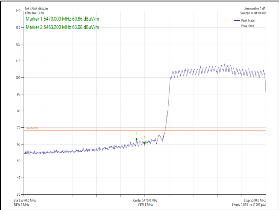
Figure 251 - 802.11ax HE80 CDD, Cores 0-1, SU - 5530 MHz Band Edge Frequency 5470 MHz
