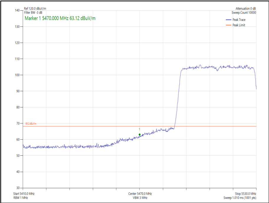
Figure 202 - 802.11ax HE40, Core 1, SU - 5510 MHz Band Edge Frequency 5470 MHz
