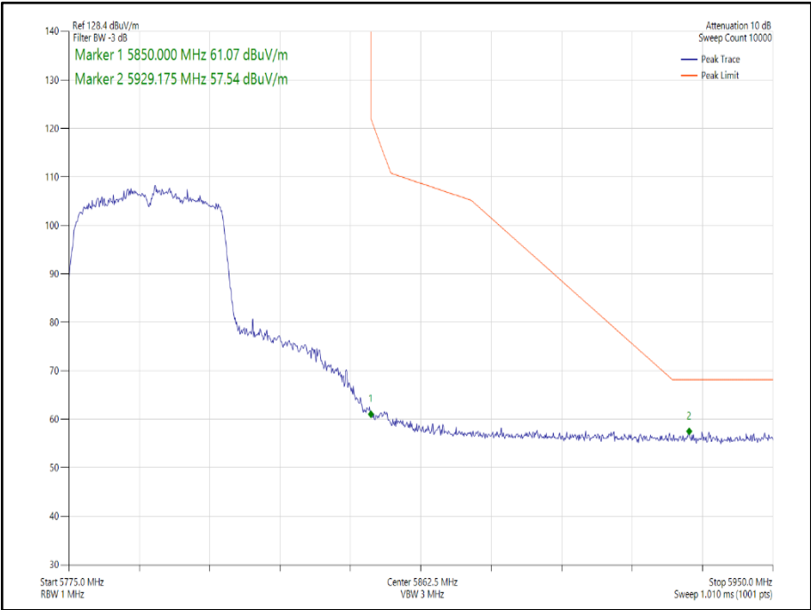
Figure 210 - 802.11n HT40, Core 0 - 5795 MHz Band Edge Frequency 5850 MHz
