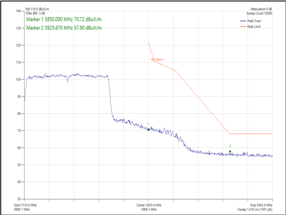
Figure 246 - 802.11ac VHT80 Core 0 - 5775 MHz Band Edge Frequency 5850 MHz
