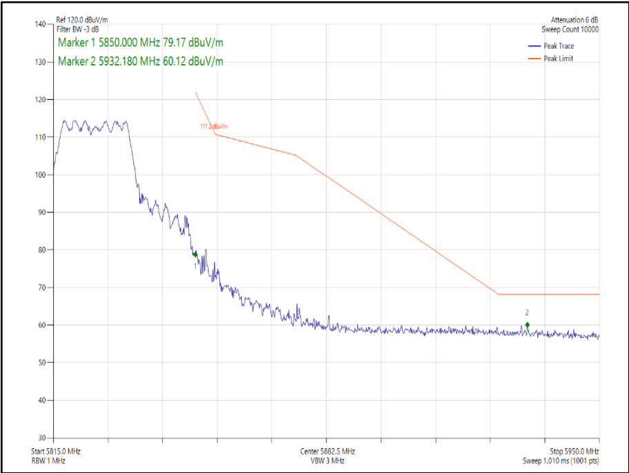
Figure 195 - 802.11n HT20 CDD, Cores 0-1 - 5825 MHz Band Edge Frequency 5850 MHz
