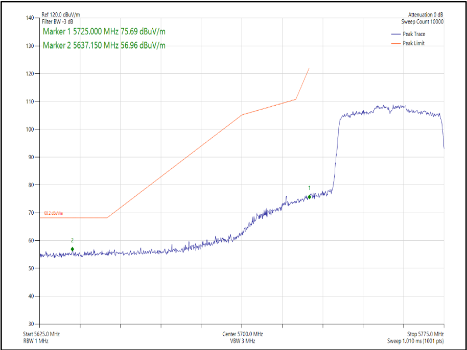
Figure 208 - 802.11ax HE40, Core 0, SU - 5755 MHz Band Edge Frequency 5725 MHz
