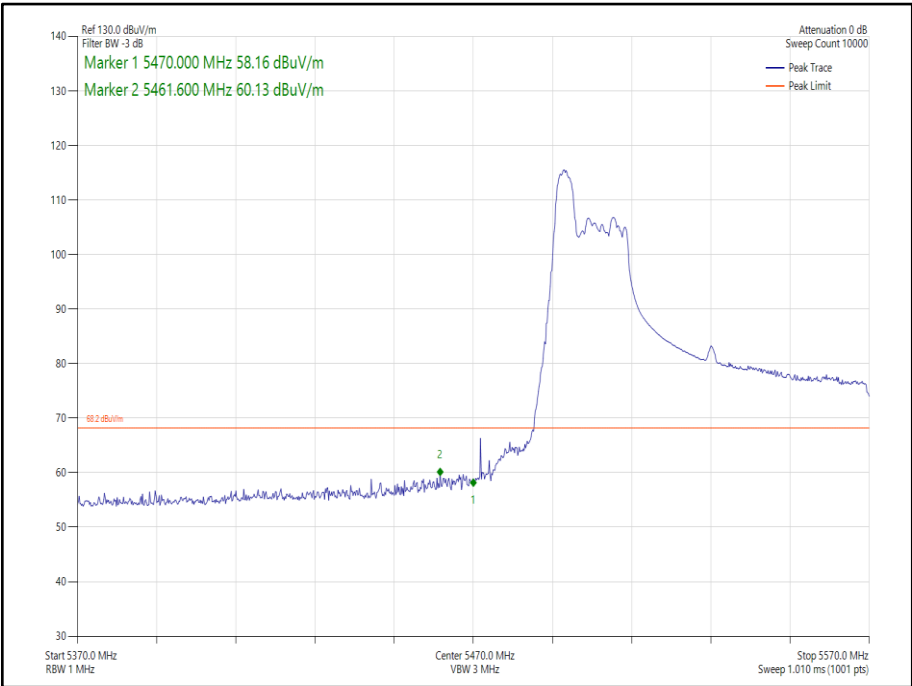
Figure 239 - 802.11ax HE80 Core 1 52-37- 5530 MHz Band Edge Frequency 5470 MHz
