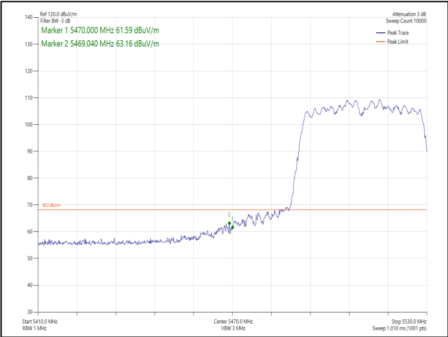
Figure 213 - 802.11n HT40 CDD, Cores 0-1 - 5510 MHz Band Edge Frequency 5470 MHz
