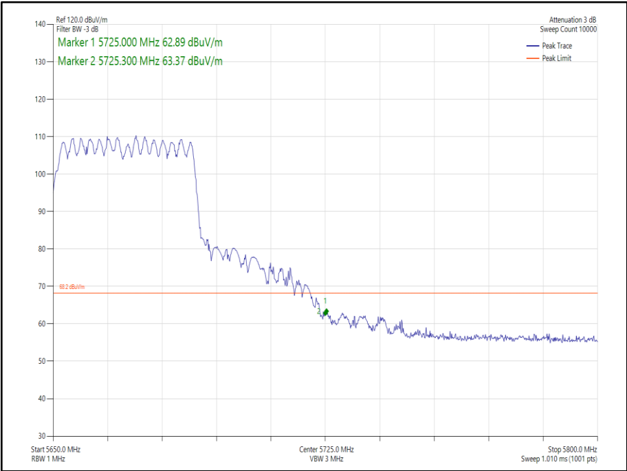
Figure 221 - 802.11ax HE40 CDD, Cores 0-1, SU - 5670 MHz Band Edge Frequency 5725 MHz
