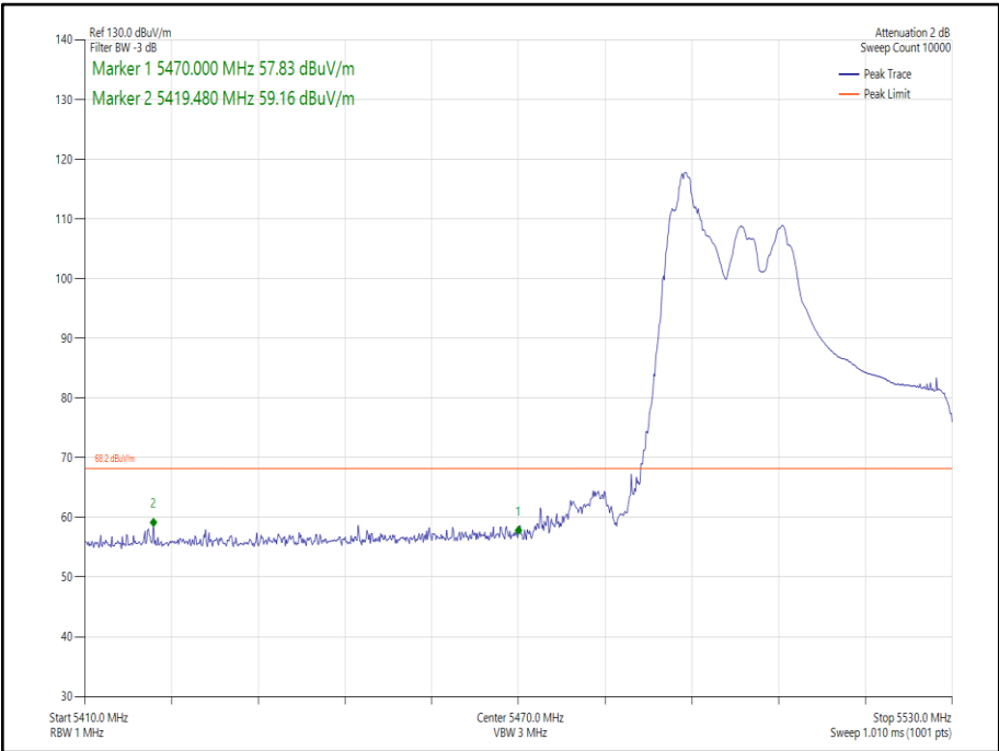
Figure 216 - 802.11ax HE40 CDD, Cores 0-1, 52-37 - 5510 MHz Band Edge Frequency 5470 MHz
