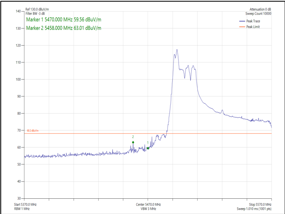
Figure 252 - 802.11ax HE80 CDD, Cores 0-1, 52-37- 5530 MHz Band Edge Frequency 5470 MHz
