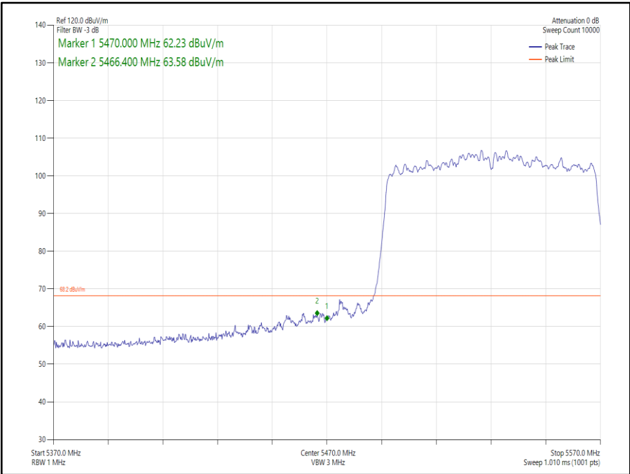
Figure 250 - 802.11ac VHT80 SDM, Cores 0-1 - 5530 MHz Band Edge Frequency 5470 MHz
