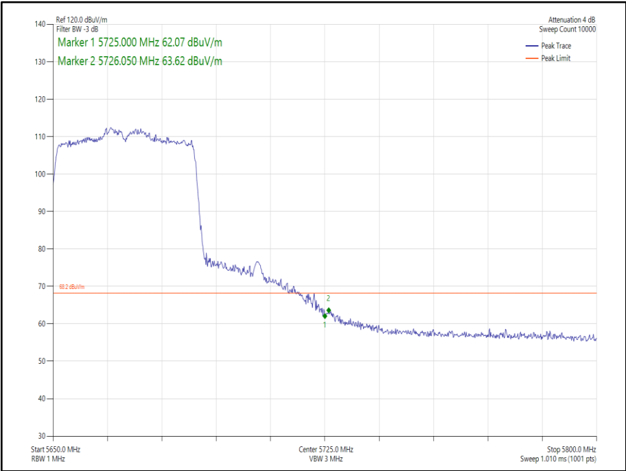
Figure 223 - 802.11ax HE40 SDM, Cores 0-1, SU - 5670 MHz Band Edge Frequency 5725 MHz
