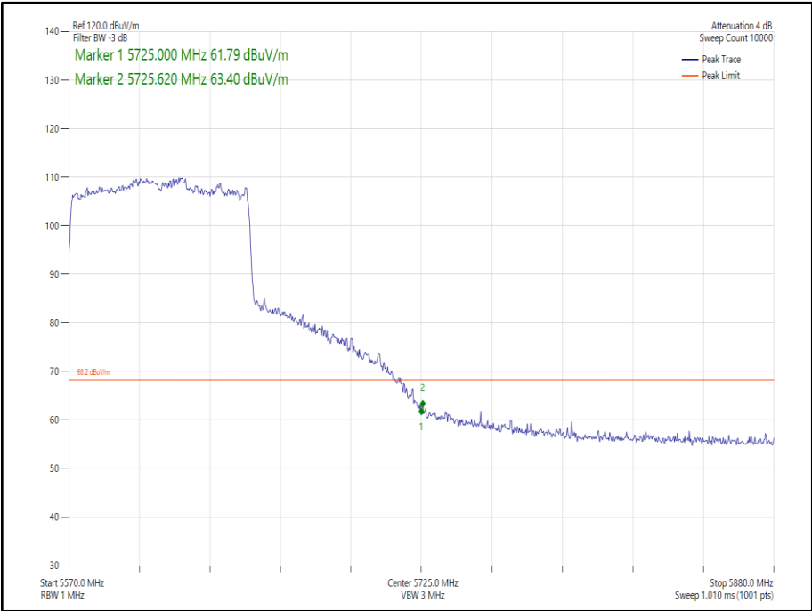
Figure 259 - 802.11ax HE80 SDM, Cores 0-1, SU - 5610 MHz Band Edge Frequency 5725 MHz
