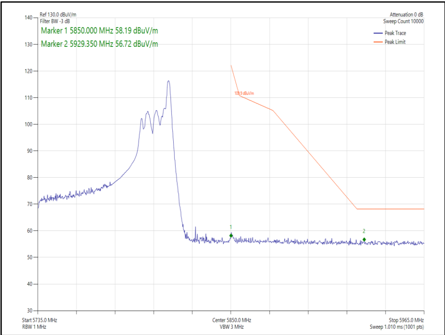
Figure 270 - 802.11ax HE80 CDD, Cores 0-1, 26-36 - 5775 MHz Band Edge Frequency 5850 MHz
