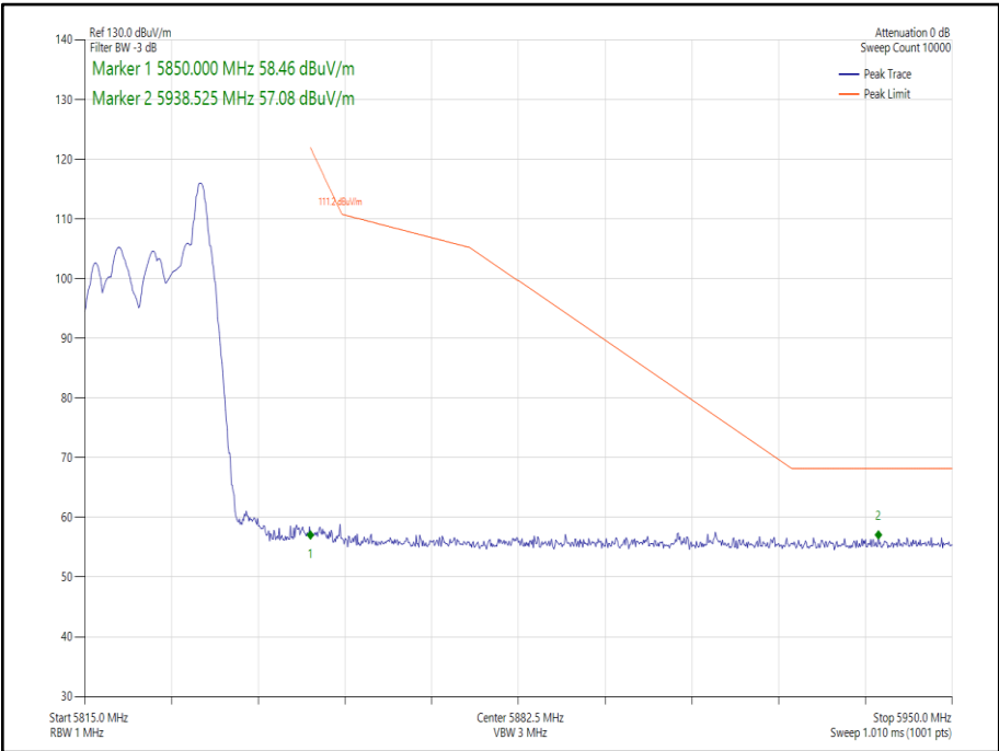
Figure 198 - 802.11ax HE20 CDD, Cores 0-1, 26-8 - 5825 MHz Band Edge Frequency 5850 MHz
