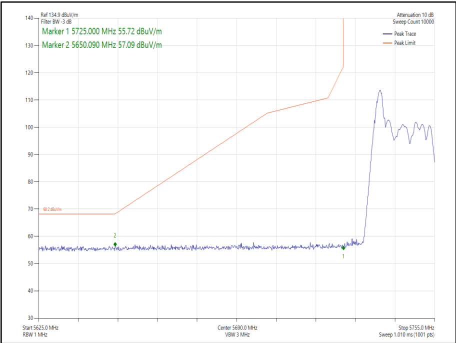
Figure 194 - 802.11ax HE20 SDM, Cores 0-1, 26-0 - 5745 MHz Band Edge Frequency 5725 MHz
