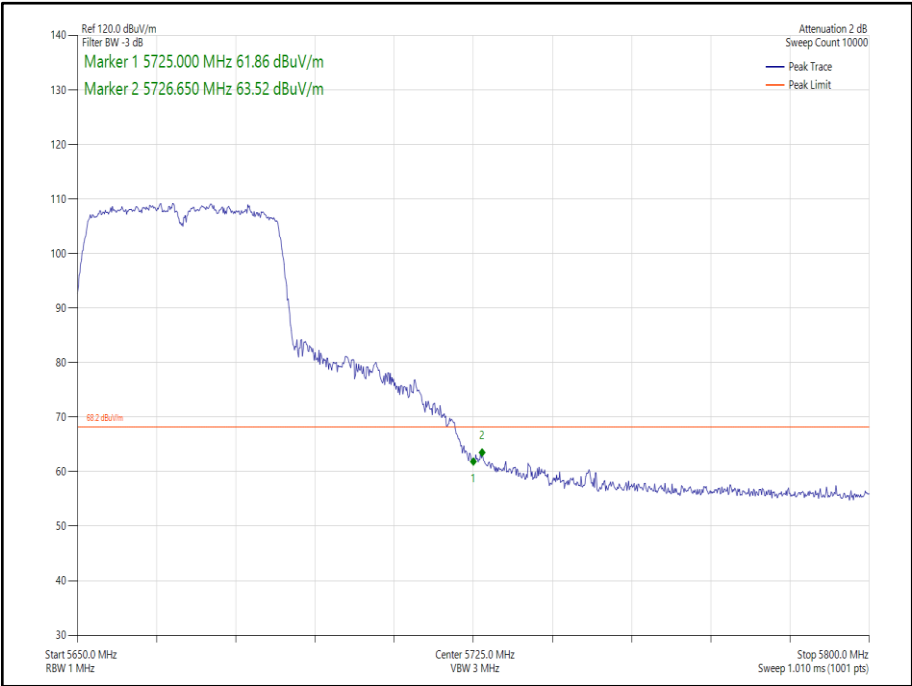
Figure 204 - 802.11n HT40, Core 1 - 5670 MHz Band Edge Frequency 5725 MHz
