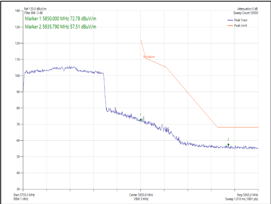
Figure 247 - 802.11ax HE80 Core 0 SU - 5775 MHz Band Edge Frequency 5850 MHz
