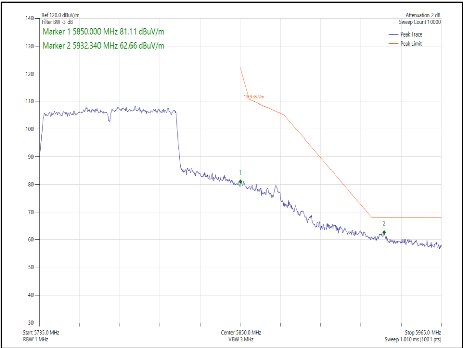
Figure 268 - 802.11ac VHT80 SDM, Cores 0-1 - 5775 MHz Band Edge Frequency 5850 MHz
