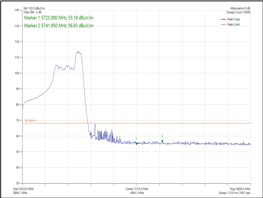
Figure 206 - 802.11ax HE40, Core 1, 52-44 - 5670 MHz Band Edge Frequency 5725 MHz
