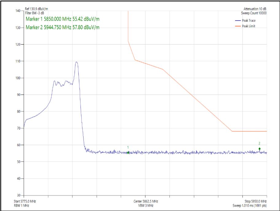
Figure 212 - 802.11ax HE40, Core 0, 26-17 - 5795 MHz Band Edge Frequency 5850 MHz
