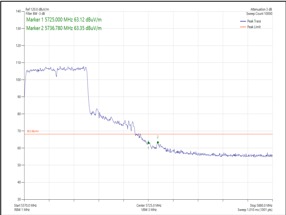
Figure 256 - 802.11ac VHT80 SDM, Cores 0-1 - 5610 MHz Band Edge Frequency 5725 MHz
