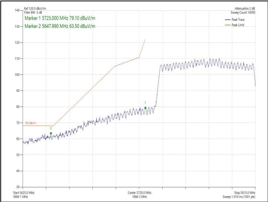
Figure 263 - 802.11ax HE80 CDD, Cores 0-1, SU - 5775 MHz Band Edge Frequency 5725 MHz
