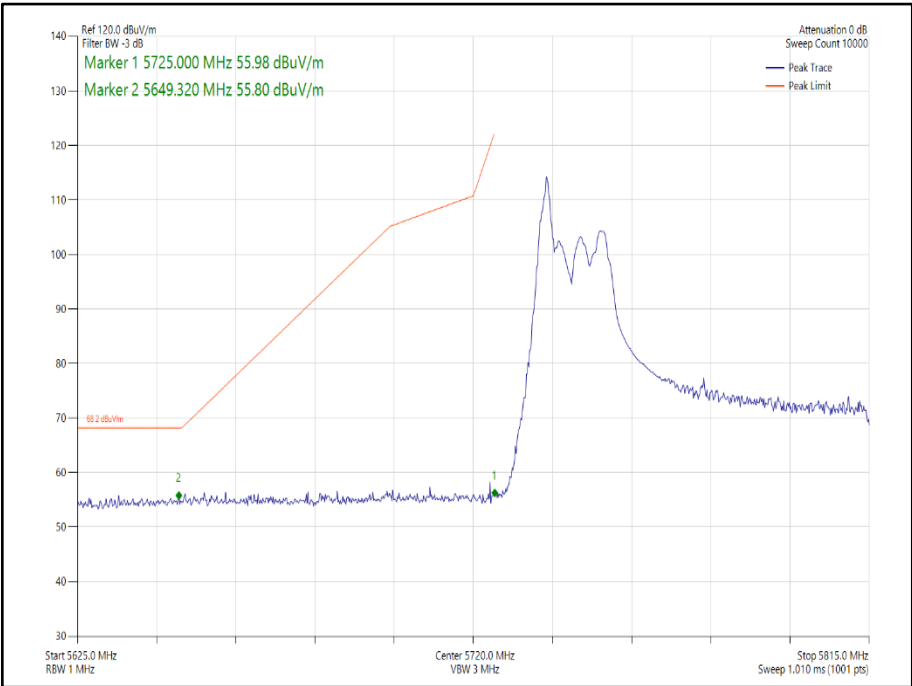
Figure 266 - 802.11ax HE80 SDM, Cores 0-1, 26-0 - 5775 MHz Band Edge Frequency 5725 MHz
