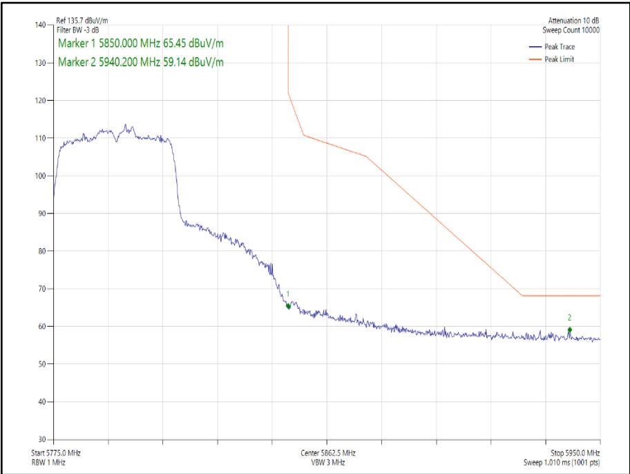
Figure 232 - 802.11n HT40 SDM, Cores 0-1 - 5795 MHz Band Edge Frequency 5850 MHz
