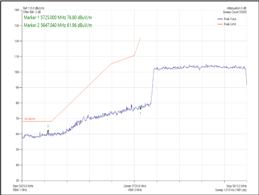
Figure 244 - 802.11ax HE80 Core 0 SU - 5775 MHz Band Edge Frequency 5725 MHz
