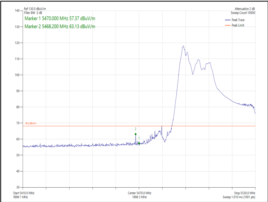
Figure 218 - 802.11ax HE40 SDM, Cores 0-1, 52-37 - 5510 MHz Band Edge Frequency 5470 MHz
