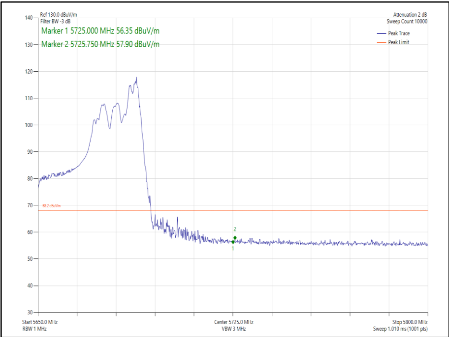
Figure 222 - 802.11ax HE40 CDD, Cores 0-1, 52-44 - 5670 MHz Band Edge Frequency 5725 MHz
