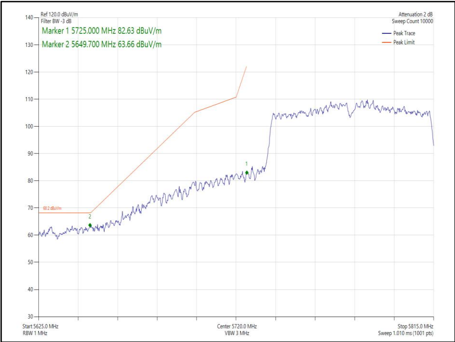
Figure 261 - 802.11ac VHT80 CDD, Cores 0-1 - 5775 MHz Band Edge Frequency 5725 MHz
