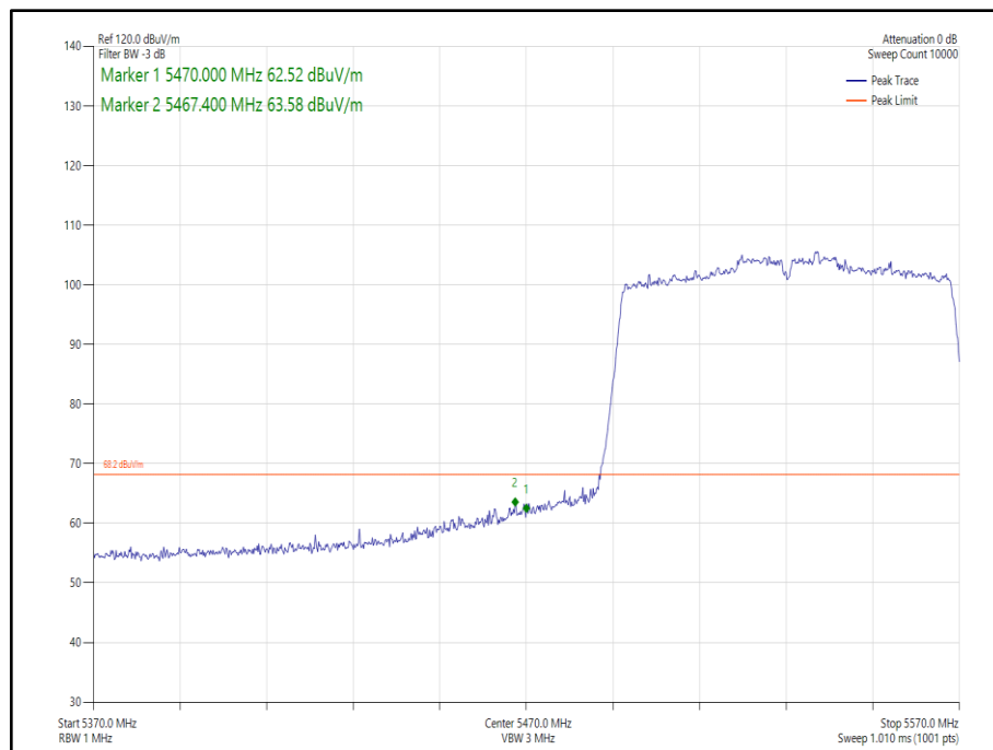
Figure 237 - 802.11ac VHT80 Core 1 - 5530 MHz Band Edge Frequency 5470 MHz
