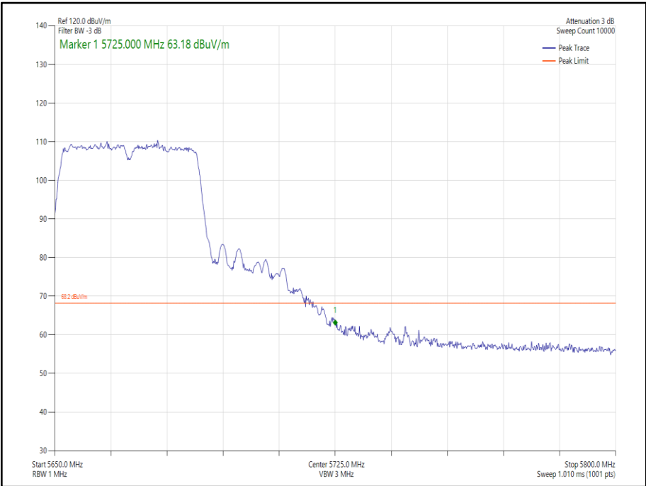
Figure 220 - 802.11n HT40 SDM, Cores 0-1 - 5670 MHz Band Edge Frequency 5725 MHz
