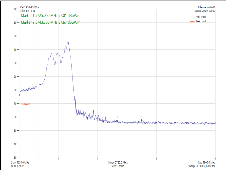
Figure 224 - 802.11ax HE40 SDM, Cores 0-1, 52-44 - 5670 MHz Band Edge Frequency 5725 MHz
