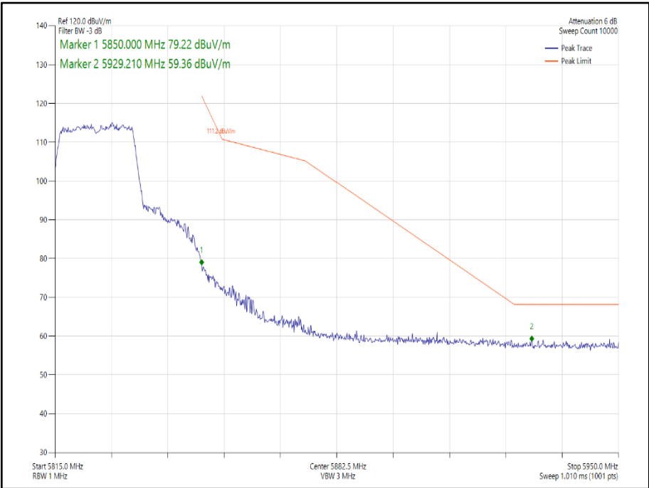
Figure 196 - 802.11n HT20 SDM, Cores 0-1 - 5825 MHz Band Edge Frequency 5850 MHz
