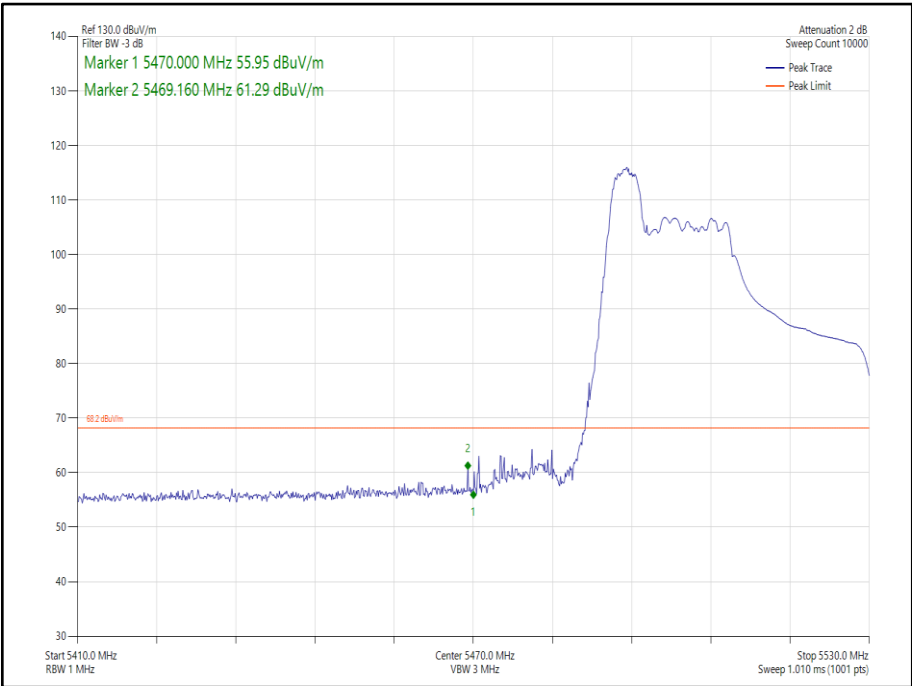
Figure 203 - 802.11ax HE40, Core 1, 52-37 - 5510 MHz Band Edge Frequency 5470 MHz
