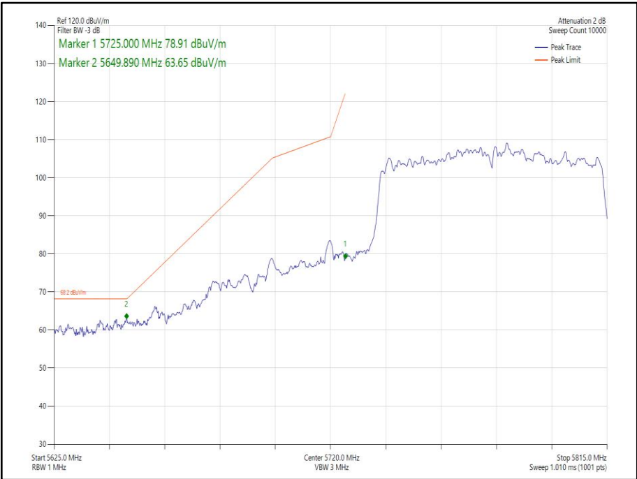
Figure 262 - 802.11ac VHT80 SDM, Cores 0-1 - 5775 MHz Band Edge Frequency 5725 MHz
