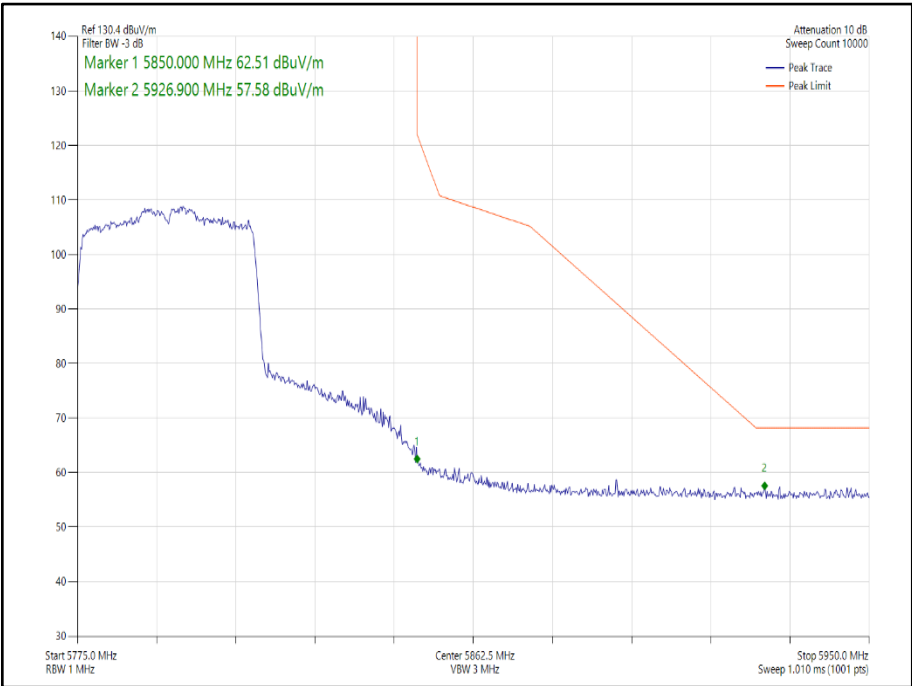
Figure 211 - 802.11ax HE40, Core 0, SU - 5795 MHz Band Edge Frequency 5850 MHz
