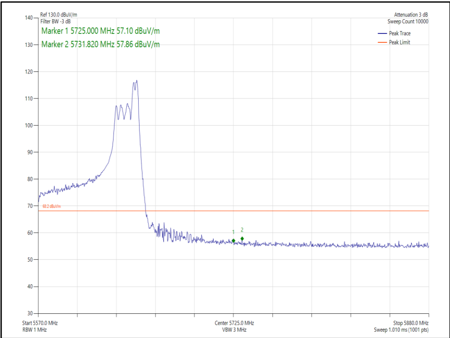
Figure 260 - 802.11ax HE80 SDM, Cores 0-1, 52-52 - 5610 MHz Band Edge Frequency 5725 MHz
