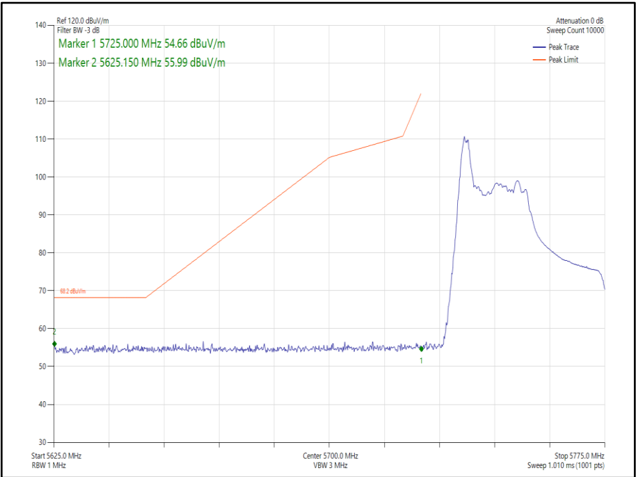
Figure 209 - 802.11ax HE40, Core 0, 26-0 - 5755 MHz Band Edge Frequency 5725 MHz
