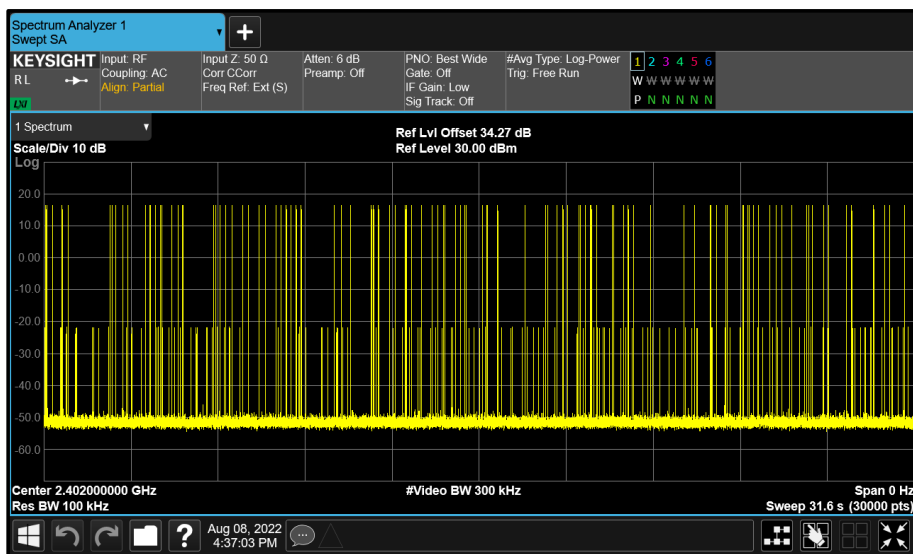
Figure 31 - GFSK - 2402 MHz Accumulated Transmit Time
