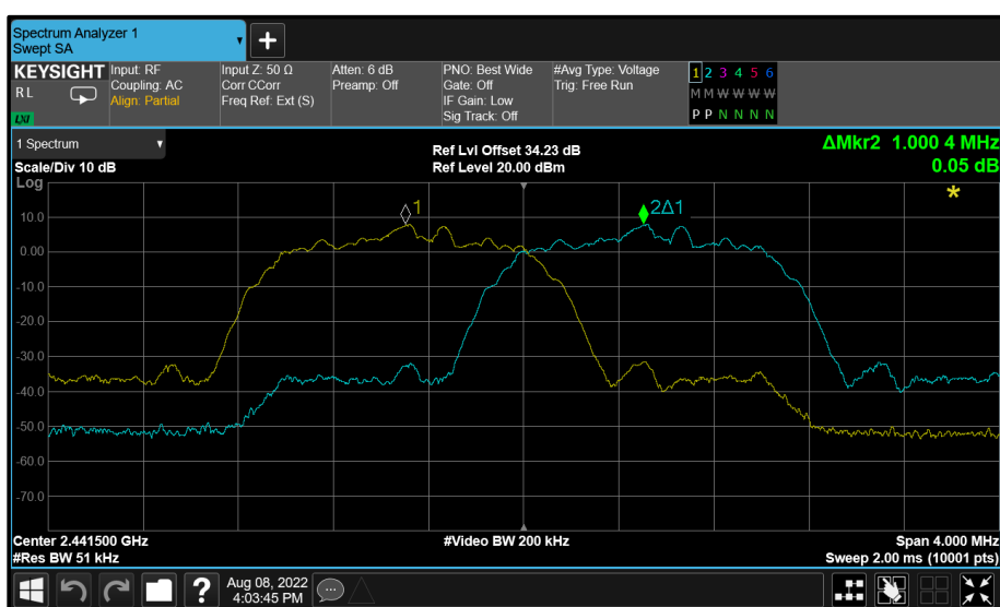
Figure 50 - \pi/4 DQPSK - 2441 MHz (CH39)
