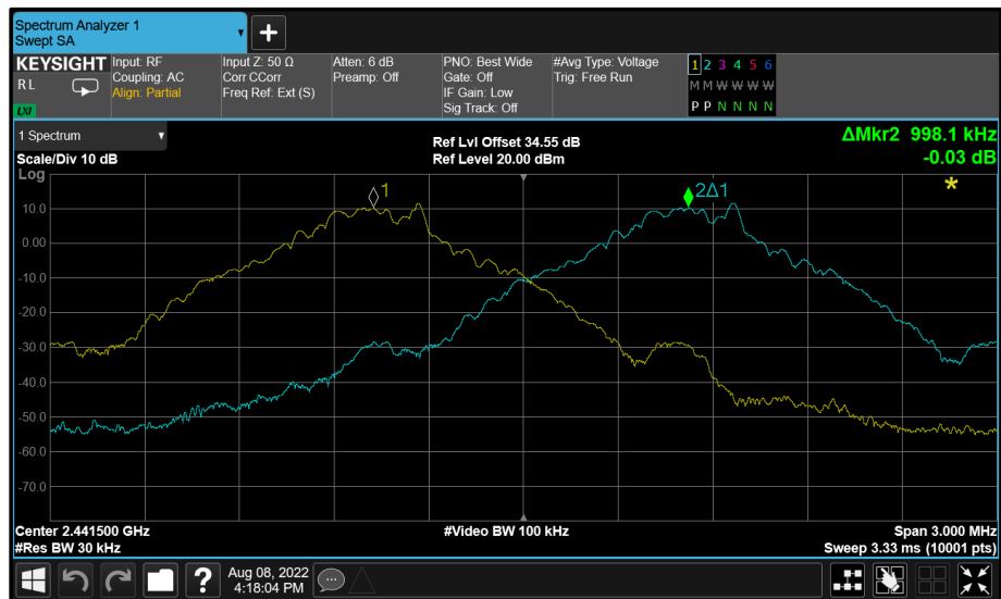
Figure 52 - GFSK - 2441 MHz (CH39)
