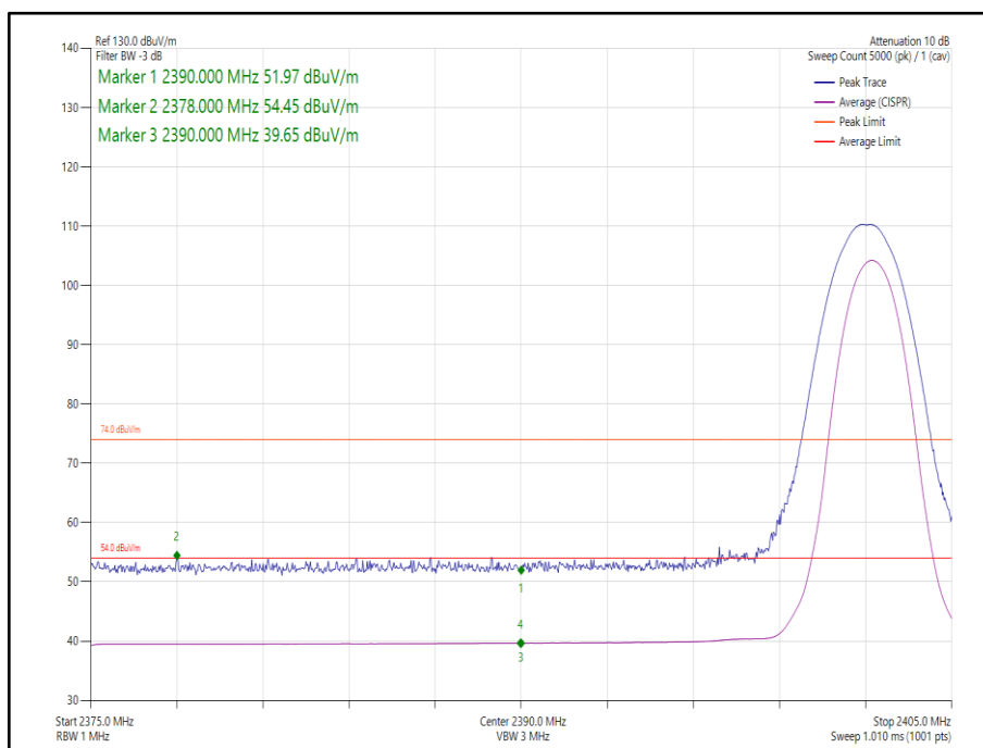
Figure 20 - Static - \pi/4 DQPSK/2DH5 - 2402 MHz - Band Edge Frequency 2390.0 MHz
