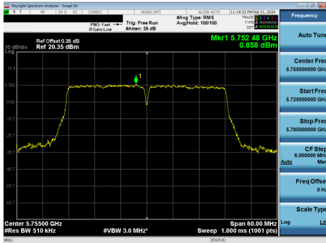
Plot 7-547. PSD Antenna 2a (40MHz BW 802.11n – Ch. 151, MCS7)
