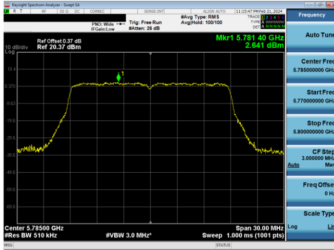
Plot 7-545. PSD Antenna 2a (20MHz BW 802.11n – Ch. 157, MCS7)
