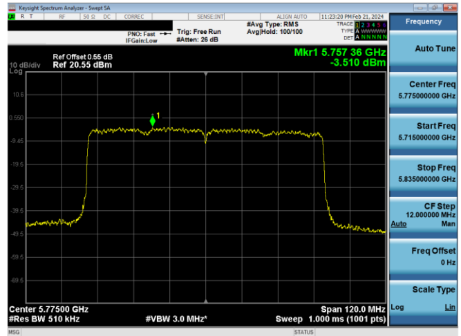
Plot 7-550. PSD Antenna 2a (80MHz BW 802.11ax SU – Ch. 155, MCS11)
