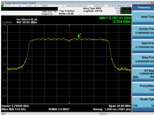
Plot 7-546. PSD Antenna 2a (20MHz BW 802.11ax(SU) – Ch. 157, MCS11)
