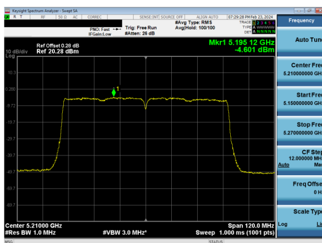
Plot 7-571. ISED PSD Antenna 2a (80MHz BW 11ac – Ch.42, MCS9)
