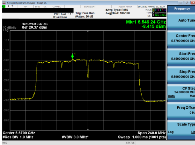
Plot 7-510. PSD Antenna 2a (160MHz BW 802.11ac – Ch. 114, MCS4)
