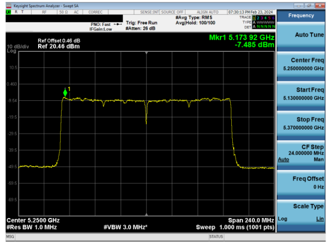
Plot 7-574. ISED PSD Antenna 2a (160MHz BW 11ax (SU) – Ch.50, MCS11)
