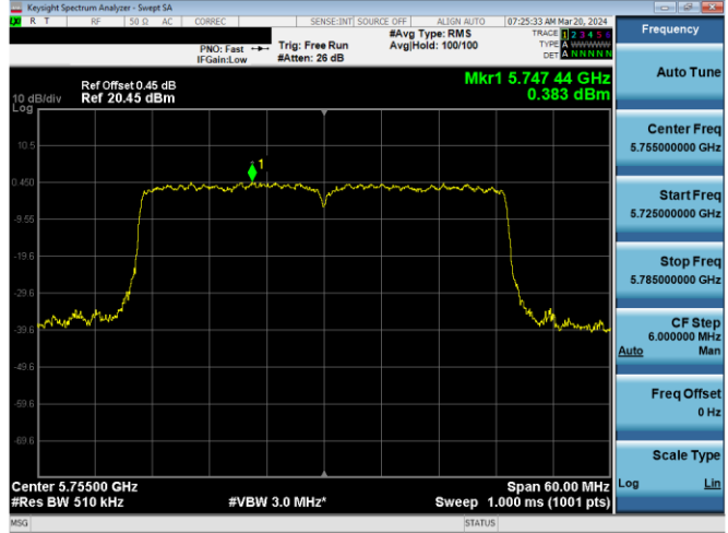
Plot 7-548. PSD Antenna 2a (40MHz BW 802.11ax(SU) – Ch. 151, MCS11)
