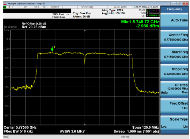
Plot 7-549. PSD Antenna 2a (80MHz BW 802.11ac – Ch. 155, MCS9)
