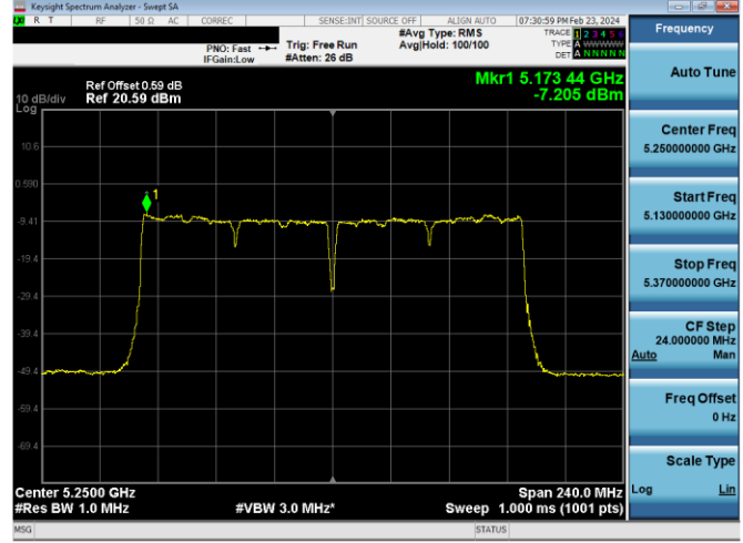
Plot 7-573. ISED PSD Antenna 2a (160MHz BW 11ac – Ch.50, MCS9)
