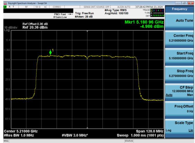
Plot 7-572. ISED PSD Antenna 2a (80MHz BW 11ax (SU) – Ch.42, MCS11)
