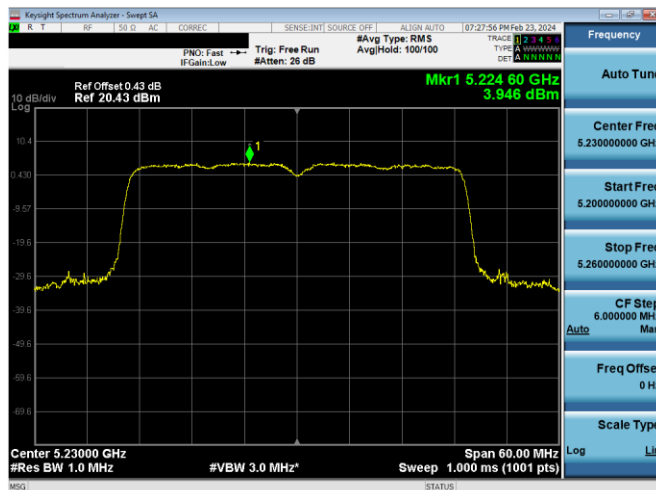
Plot 7-570. ISED PSD Antenna 2a (40MHz BW 11ax(SU) – Ch.46, MCS11)
