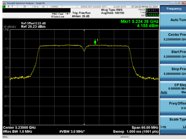
Plot 7-569. ISED PSD Antenna 2a (40MHz BW 11n – Ch.46, MCS7)
