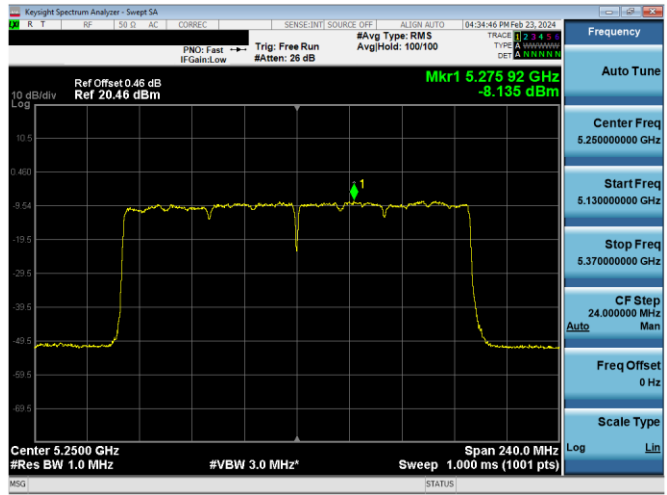
Plot 7-467. ISED PSD Antenna 4a (160MHz BW 11ax (SU) – Ch.50, MCS11)
