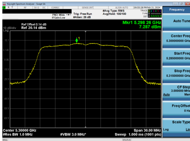
Plot 7-498. PSD Antenna 2a (20MHz BW 802.11n – Ch. 60, MCS4)
