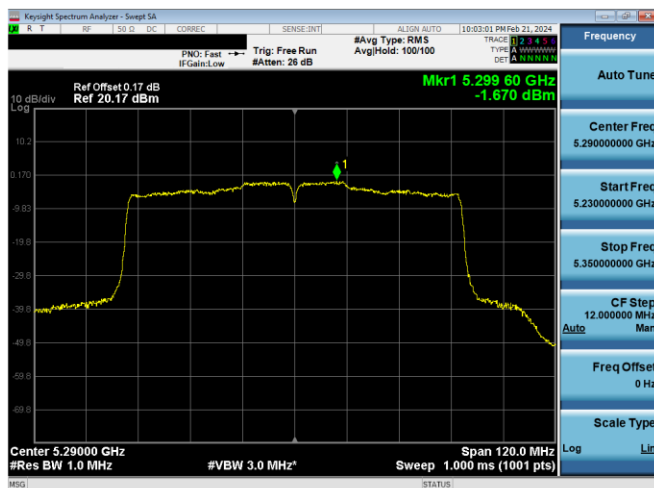
Plot 7-502. PSD Antenna 2a (80MHz BW 802.11ac – Ch. 58, MCS4)
