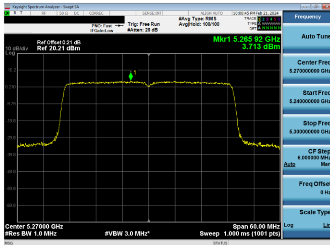
Plot 7-501. PSD Antenna 2a (40MHz BW 802.11ax(SU) – Ch. 54, MCS4)
