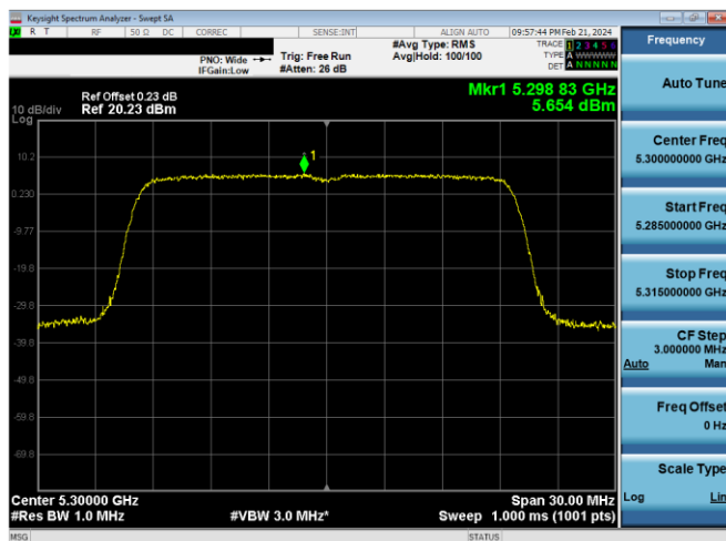
Plot 7-499. PSD Antenna 2a (20MHz BW 802.11ax(SU) – Ch. 60, MCS4)
