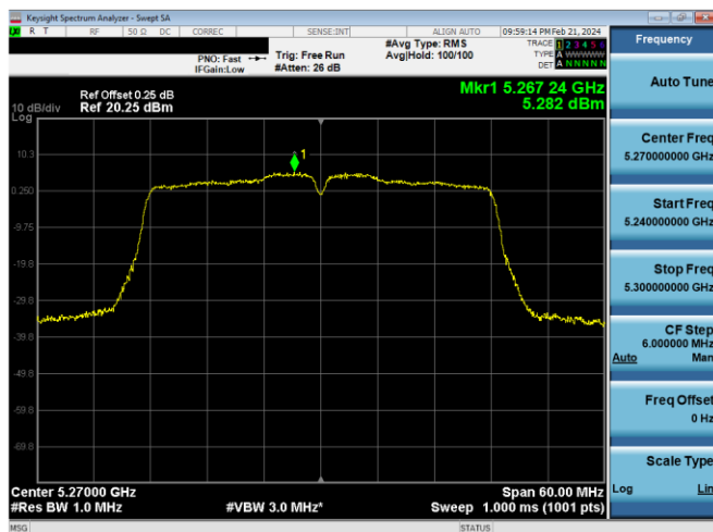
Plot 7-500. PSD Antenna 2a (40MHz BW 802.11n – Ch. 54, MCS4)
