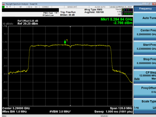
Plot 7-503. PSD Antenna 2a (80MHz BW 802.11ax(SU) – Ch. 58, MCS4)
