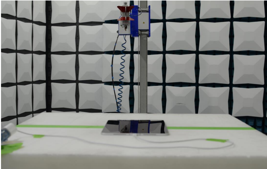
Figure 2: 1-18GHz Test Setup (Rear View)
