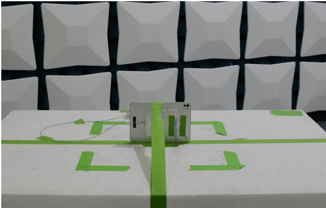
Figure 9: 30MHz-1GHz Test Setup (Front View)
