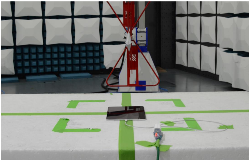
Figure 8: 30MHz-1GHz Test Setup (Rear View)
