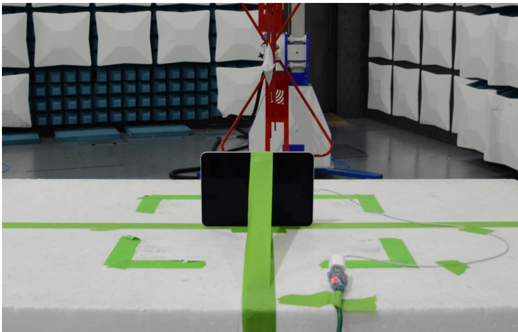
Figure 10: 30MHz-1GHz Test Setup (Rear View)
