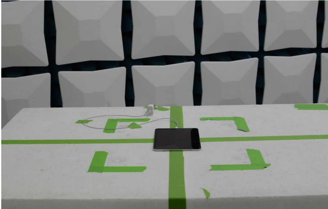
Figure 7: 30MHz-1GHz Test Setup (Front View)
