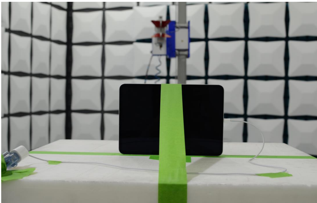
Figure 4: 1-18GHz Test Setup (Rear View)
