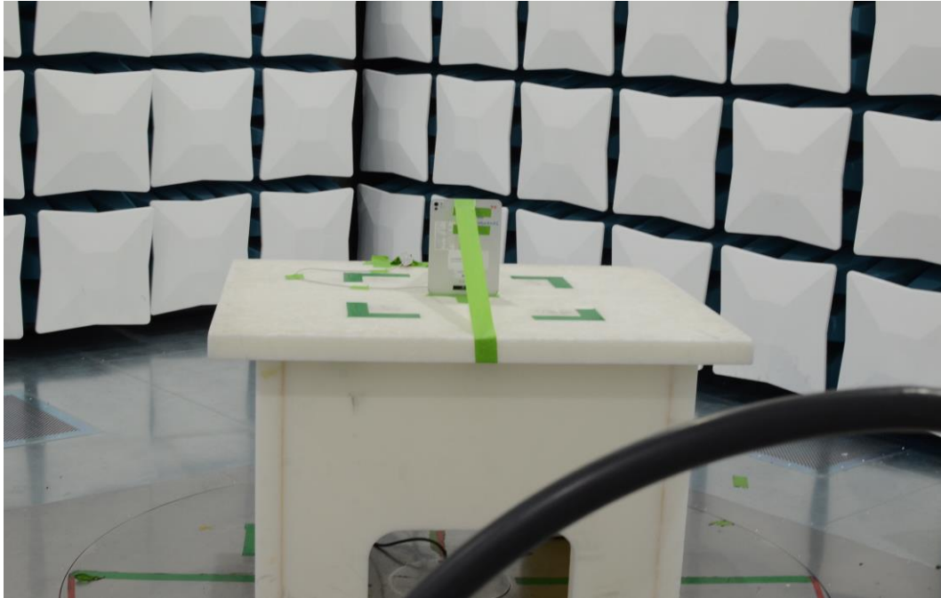
Figure 21: 9kHz-30MHz Test Setup (Front View)
