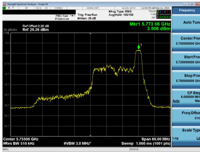
Plot 7-624. PSD CDD Diversity Antenna WF5B (40MHz BW 11ax Index 17 - RU26 - Ch.151)
