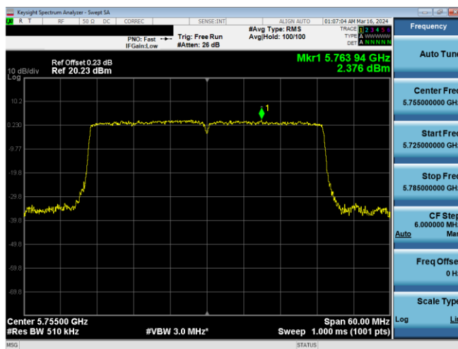
Plot 7-626. PSD CDD Diversity Antenna WF5B (40MHz BW 11ax - RU484 - Ch.151)
