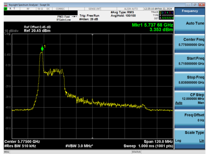
Plot 7-629. PSD CDD Diversity Antenna 2a (80MHz BW 11ax Index 0 - RU26 - Ch.155)
