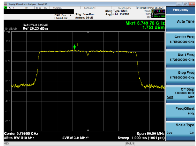
Plot 7-627. PSD CDD Diversity Antenna 2a (40MHz BW 11ax - RU484 - Ch.151)
