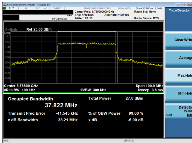
Plot 7-164. 6dB BW & 99% OBW Antenna 2a (40MHz BW 11ax – RU484 – Ch.151)
