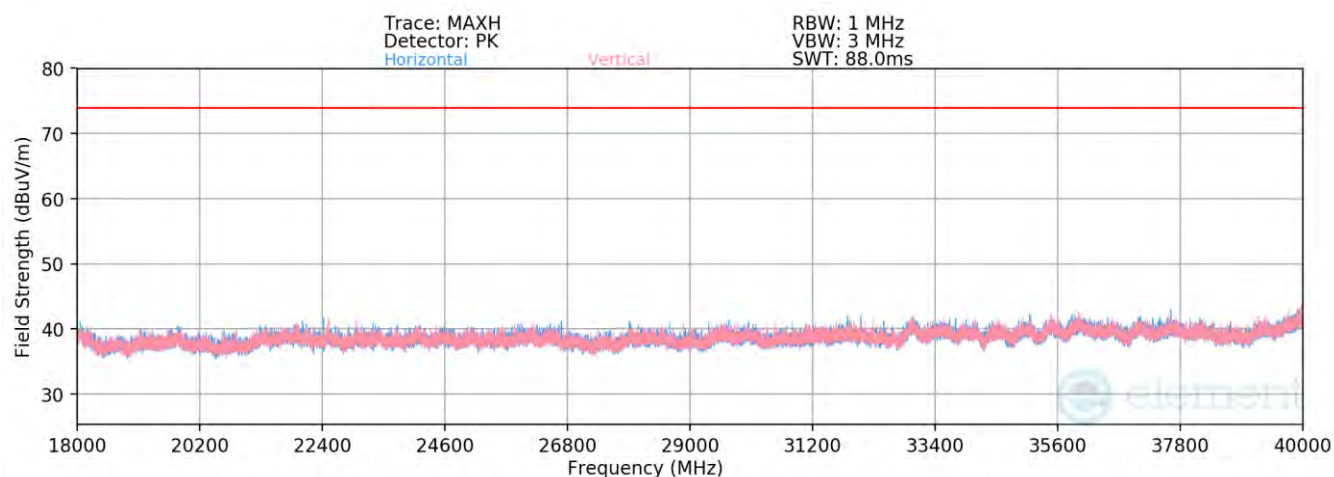
Plot 7-89. Radiated Spurious Emissions Above 18GHz TxBF (1Mbps, ePA – Ch. 19)
