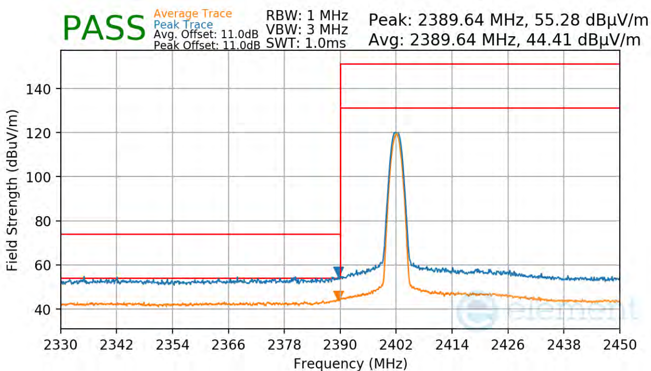
Plot 7-91. Radiated Restricted Lower Band Edge Measurement Antenna 4a (Average & Peak)
