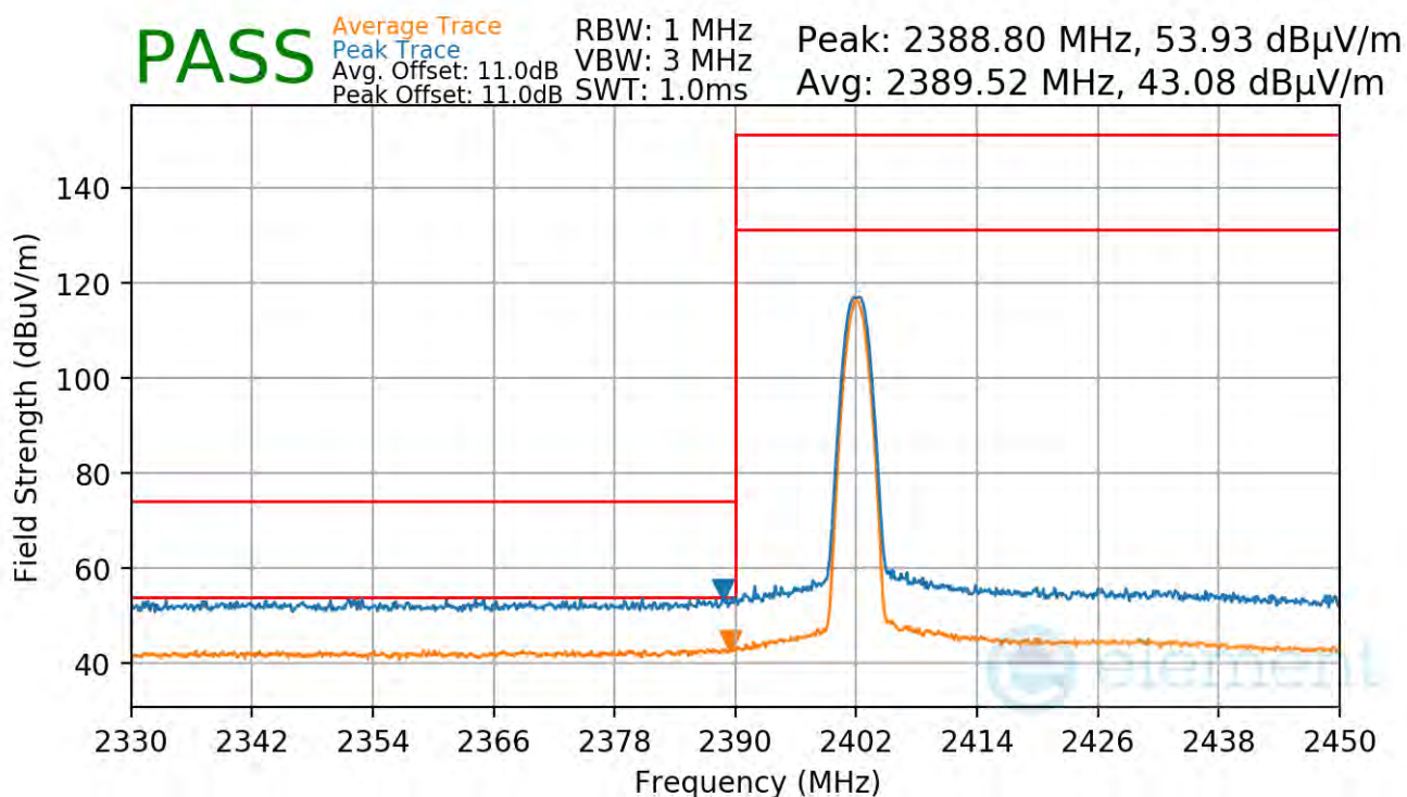
Plot 7-95. Radiated Restricted Lower Band Edge Measurement Antenna 2a (Average & Peak)
