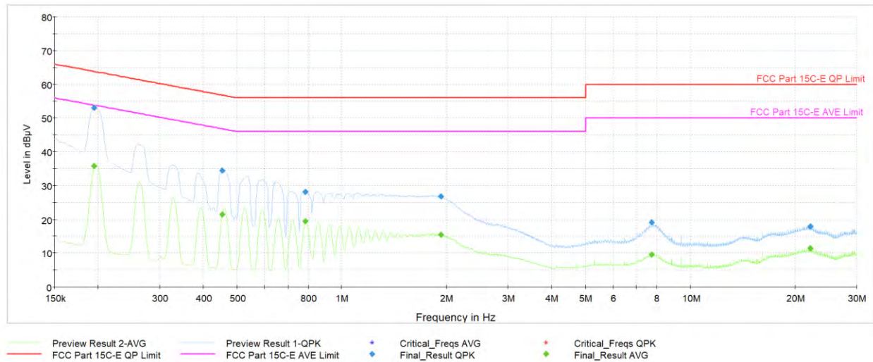
Plot 7-105. AC Line Conducted Plot with Bluetooth LE TxBF (N, 1Mbps ePA – Ch.19, with AC/DC Adapter)
