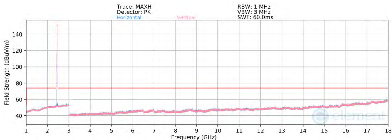
Plot 7-82. Radiated Spurious Emissions 1-18GHz Antenna 4a (1Mbps, ePA – Ch. 19)
