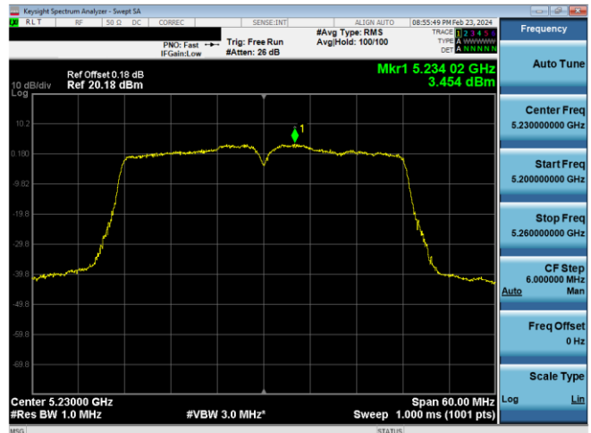
Plot 7-892. ISED PSD SDM Antenna WF7 (40MHz BW 11n – Ch.46, MCS12)
