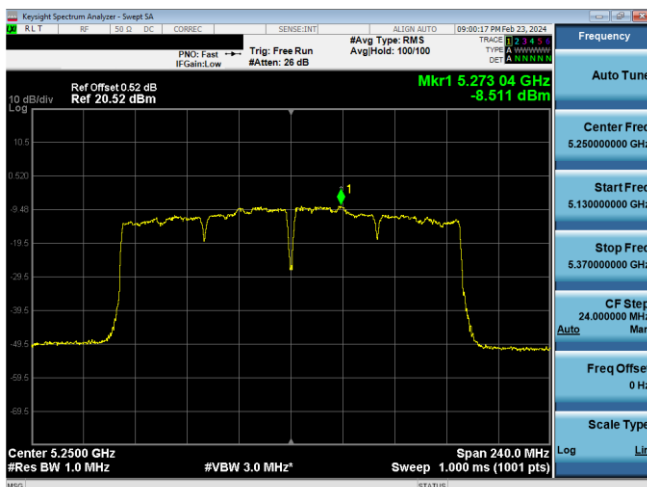
Plot 7-896. ISED PSD CDD Antenna WF7 (160MHz BW 11ac – Ch.50, MCS4)
