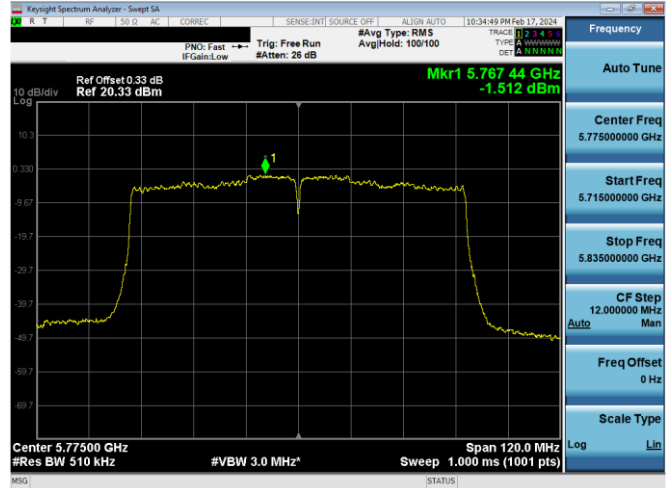
Plot 7-867. PSD CDD Antenna WF7 (80MHz BW 802.11ac – Ch. 155, MCS4)
