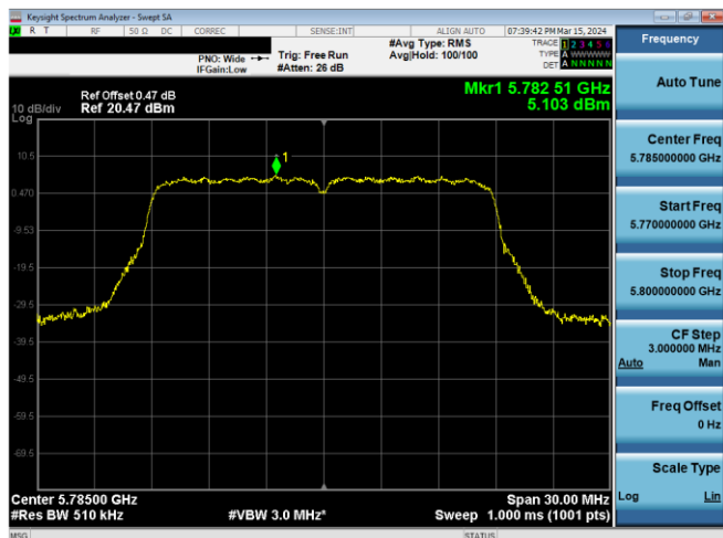
Plot 7-771. PSD CDD Antenna WF7 (20MHz BW 802.11n – Ch. 157, MCS15)
