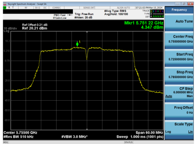
Plot 7-851. PSD CDD Antenna WF7 (40MHz BW 802.11n – Ch. 151, MCS10)
