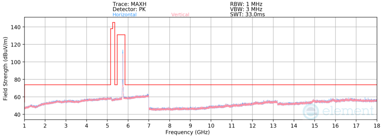
Plot 7-915. Radiated Spurious Emissions above 1GHz Antenna WF5b (802.11n – Ch. 149)
