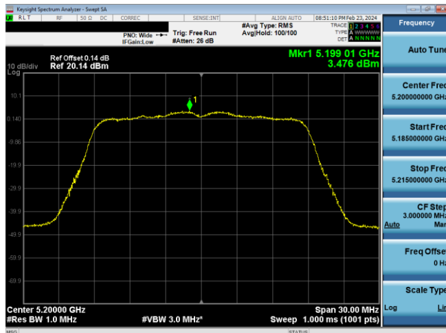
Plot 7-890. ISED PSD CDD Antenna WF7 (20MHz BW 11n – Ch.40, MCS12)
