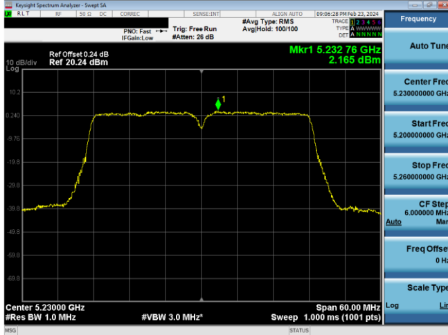
Plot 7-900. ISED PSD SDM Antenna WF7 (40MHz BW 11n – Ch.46, MCS15)
