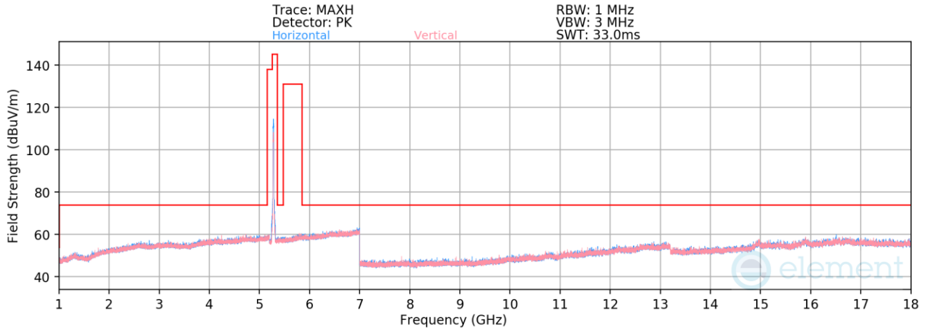
Plot 7-910. Radiated Spurious Emissions above 1GHz Antenna WF5b (802.11n – Ch. 56)
