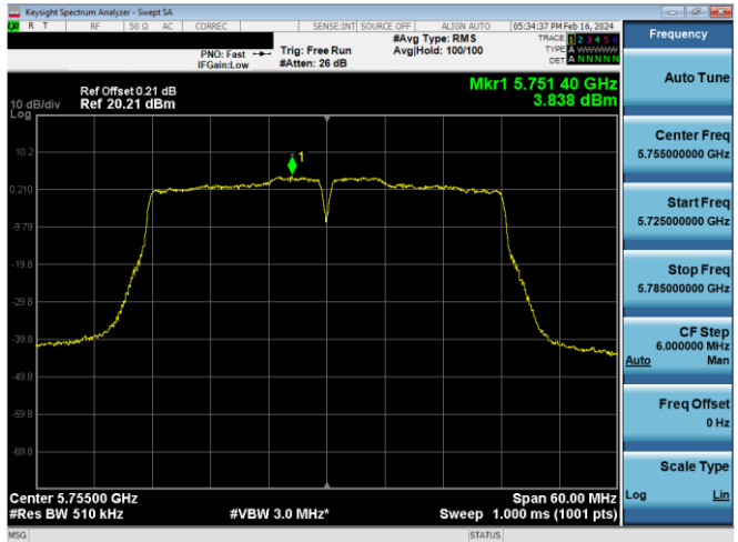
Plot 7-850. PSD CDD Antenna WF5b (40MHz BW 802.11n – Ch. 151, MCS10)
