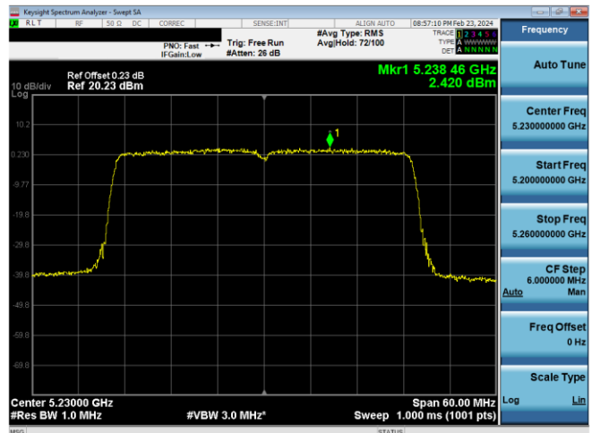
Plot 7-893. ISED SDM PSD Antenna WF7 (40MHz BW 11ax(SU) – Ch.46, MCS4)
