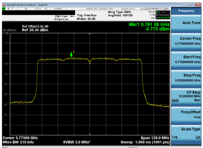
Plot 7-881. PSD CDD Antenna WF7 (80MHz BW 802.11ax(SU) – Ch. 155, MCS11)
