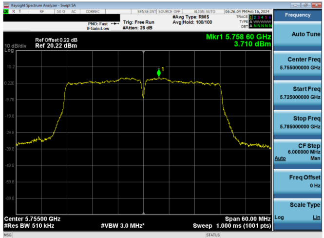
Plot 7-862. PSD CDD Antenna WF5b (40MHz BW 802.11n – Ch. 151, MCS12)
