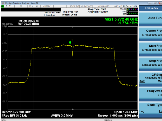
Plot 7-866. PSD CDD Antenna WF5b (80MHz BW 802.11ac – Ch. 155, MCS4)
