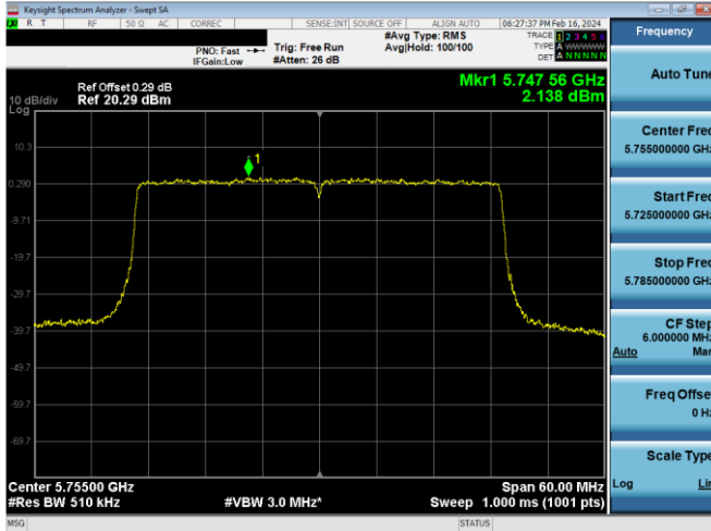
Plot 7-864. PSD CDD Antenna WF5b (40MHz BW 802.11ax(SU) – Ch. 151, MCS4)
