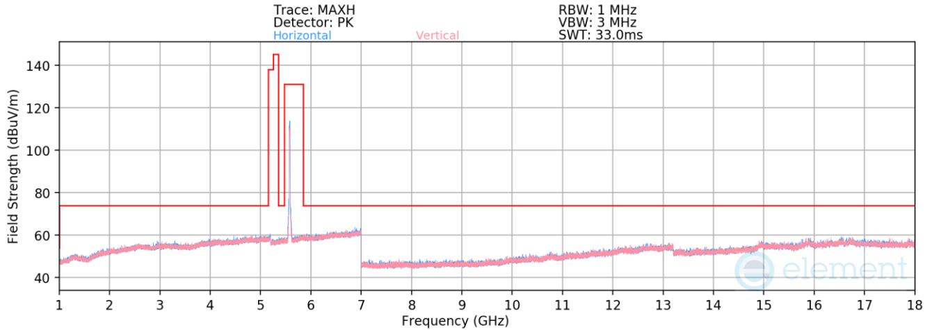
Plot 7-913. Radiated Spurious Emissions above 1GHz Antenna WF5b (802.11n – Ch. 116)
