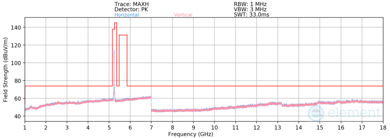
Plot 7-908. Radiated Spurious Emissions above 1GHz Antenna WF5b (802.11n – Ch. 48)
