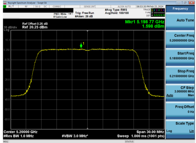
Plot 7-891. ISED PSD SDM Antenna WF7 (20MHz BW 11ax(SU) – Ch.40, MCS4)
