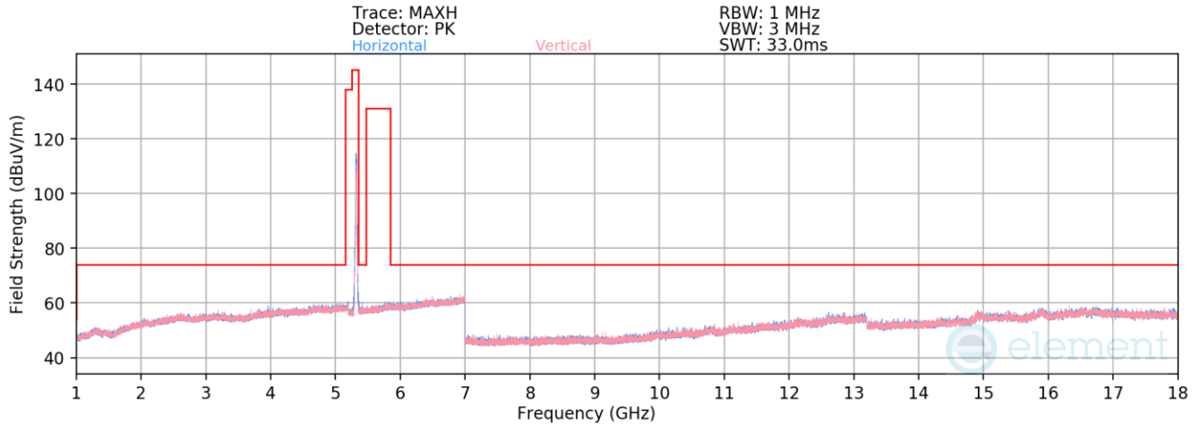
Plot 7-911. Radiated Spurious Emissions above 1GHz Antenna WF5b (802.11n – Ch. 64)
