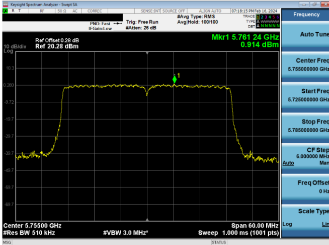
Plot 7-876. PSD CDD Antenna WF5b (40MHz BW 802.11ax(SU) – Ch. 151, MCS11)
