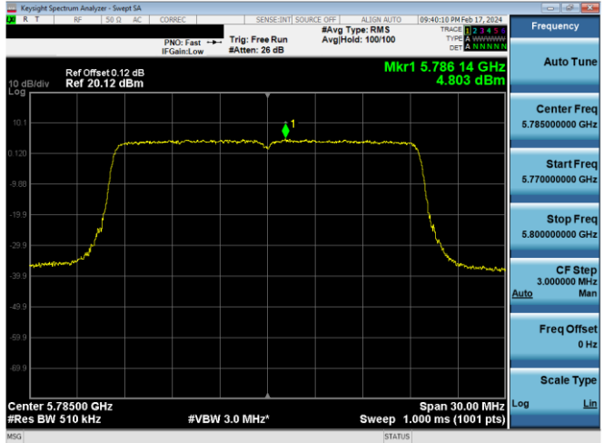
Plot 7-849. PSD CDD Antenna WF7 (20MHz BW 802.11ax(SU) – Ch. 157, MCS2)
