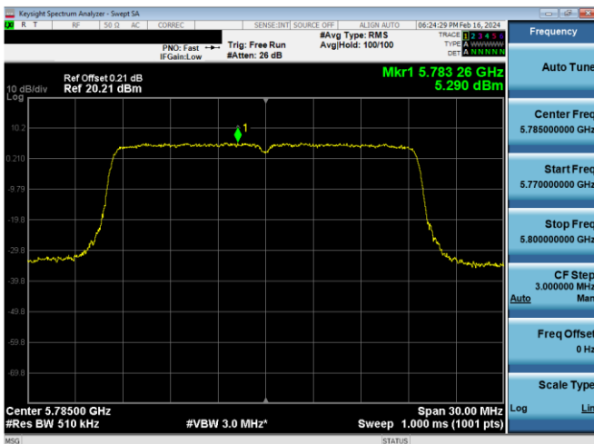
Plot 7-860. PSD CDD Antenna WF5b (20MHz BW 802.11ax(SU) – Ch. 157, MCS4)
