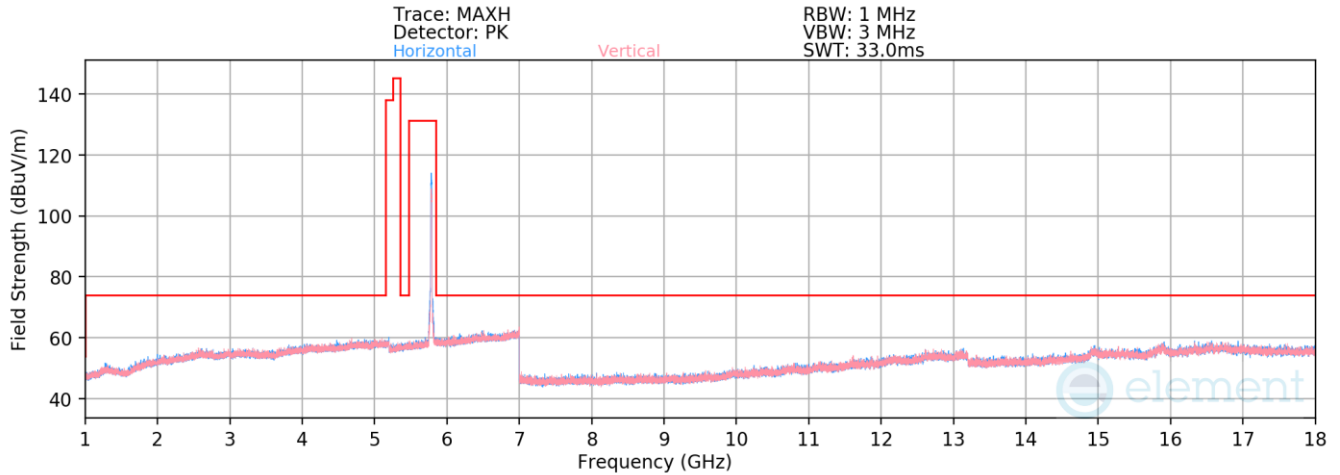
Plot 7-916. Radiated Spurious Emissions above 1GHz Antenna WF5b (802.11n – Ch. 157)
