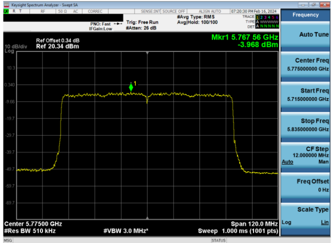
Plot 7-880. PSD CDD Antenna WF5b (80MHz BW 802.11ax(SU) – Ch. 155, MCS11)
