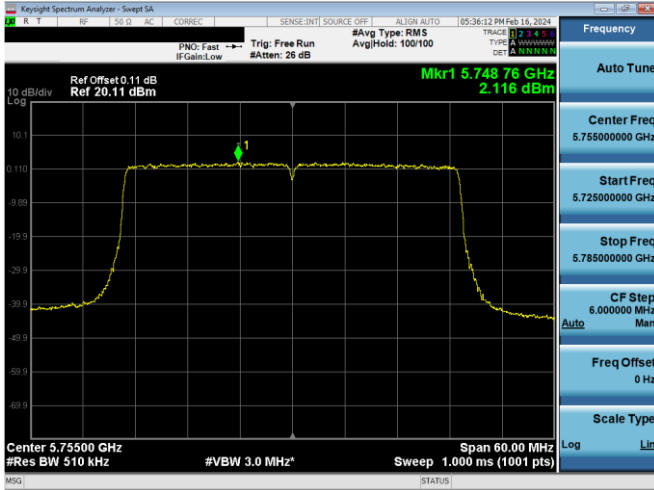
Plot 7-852. PSD CDD Antenna WF5b (40MHz BW 802.11ax(SU) – Ch. 151, MCS2)
