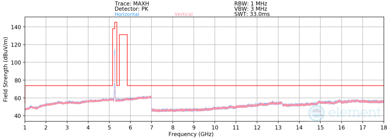
Plot 7-909. Radiated Spurious Emissions above 1GHz Antenna WF5b (802.11n – Ch. 52)
