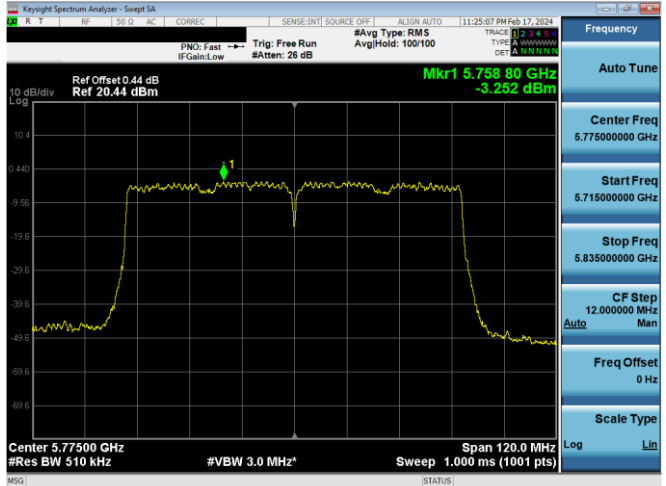
Plot 7-879. PSD CDD Antenna WF7 (80MHz BW 802.11ac – Ch. 155, MCS9)
