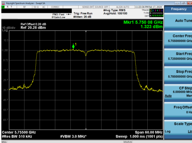
Plot 7-877. PSD CDD Antenna WF7 (40MHz BW 802.11ax(SU) – Ch. 151, MCS11)
