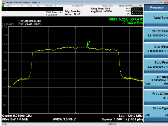
Plot 7-894. ISED PSD CDD Antenna WF7 (80MHz BW 11ac – Ch.42, MCS4)
