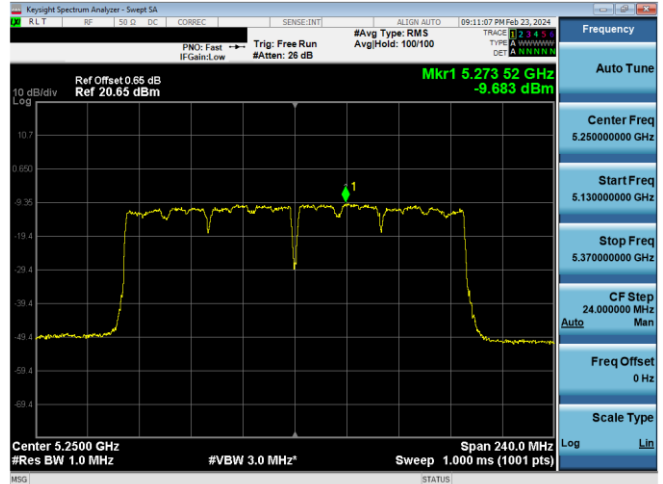
Plot 7-904. ISED PSD CDD Antenna WF7 (160MHz BW 11ac – Ch.50, MCS9)
