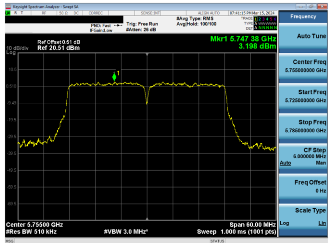
Plot 7-775. PSD CDD Antenna WF7 (40MHz BW 802.11n – Ch. 151, MCS15)
