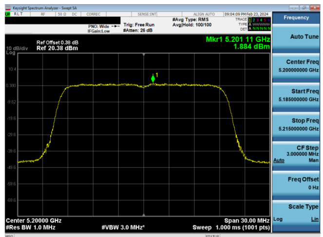
Plot 7-899. ISED PSD CDD Antenna WF7 (20MHz BW 11ax(SU) – Ch.40, MCS11)
