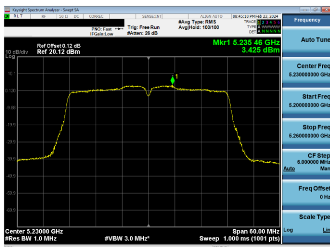
Plot 7-884. ISD PSD SDM Antenna WF7 (40MHz BW 11n – Ch.46, MCS10)
