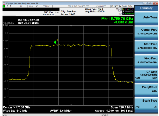
Plot 7-868. PSD CDD Antenna WF5b (80MHz BW 802.11ax(SU) – Ch. 155, MCS4)
