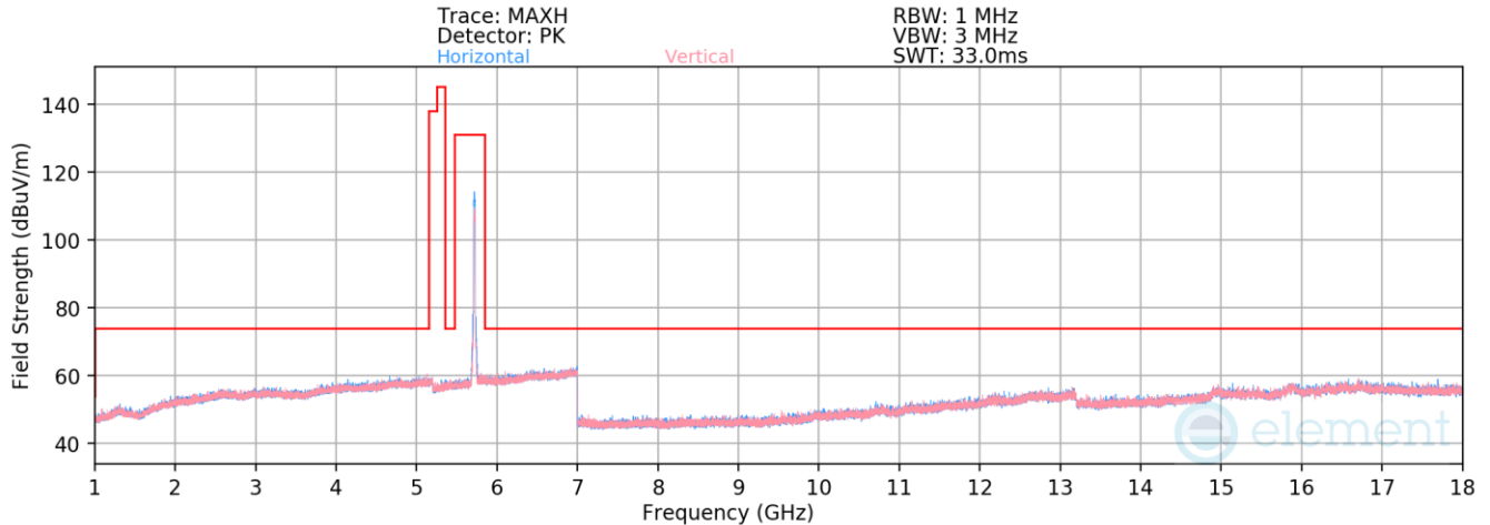
Plot 7-914. Radiated Spurious Emissions above 1GHz Antenna WF5b (802.11n – Ch. 144)
