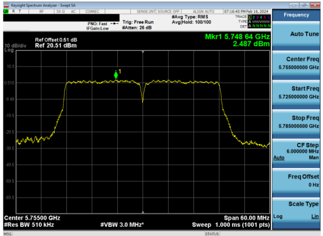
Plot 7-774. PSD CDD Antenna WF5b (40MHz BW 802.11n – Ch. 151, MCS15)
