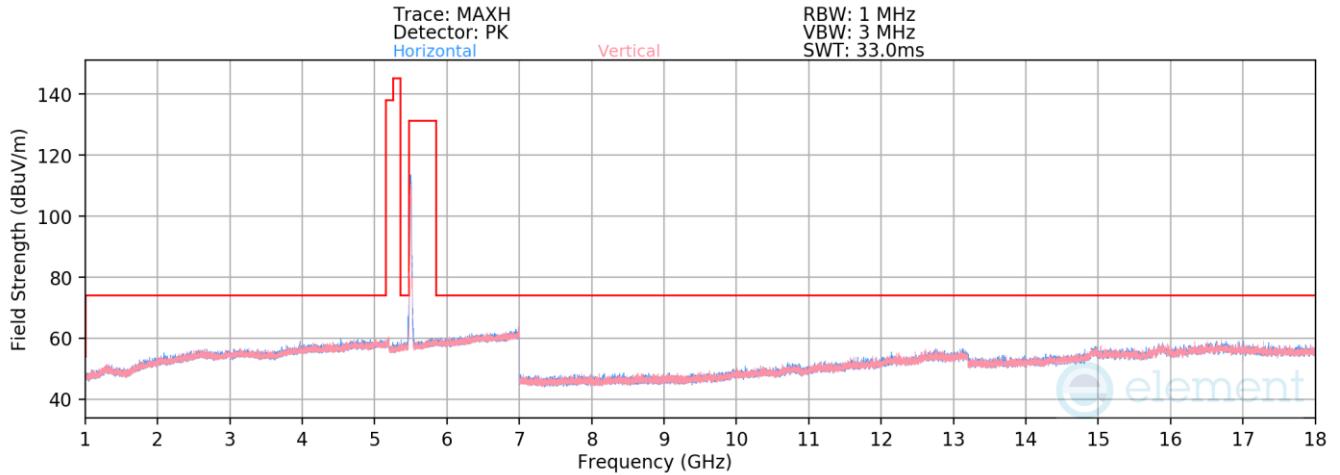
Plot 7-912. Radiated Spurious Emissions above 1GHz Antenna WF5b (802.11n – Ch. 100)
