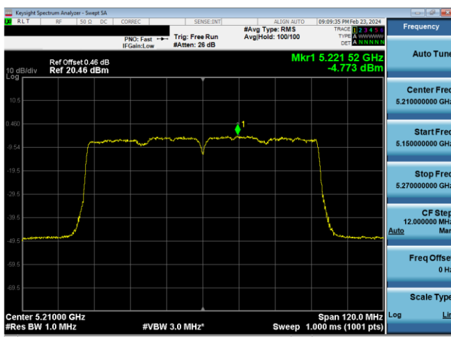
Plot 7-902. ISED PSD CDD Antenna WF7 (80MHz BW 11ac – Ch.42, MCS9)
