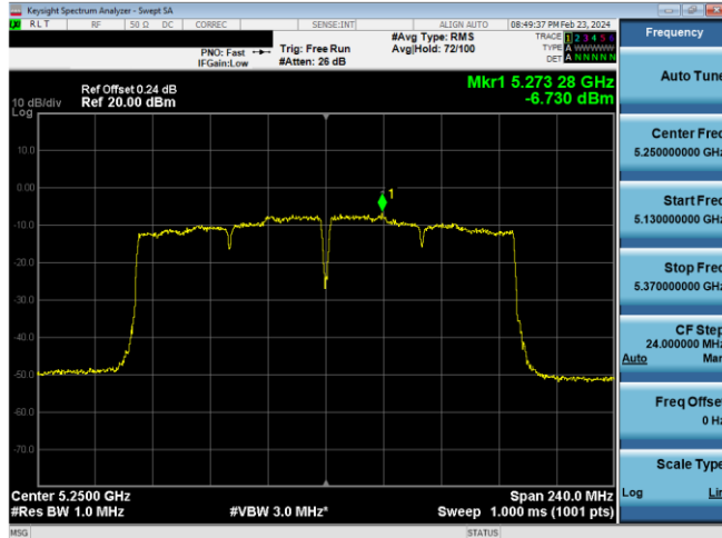
Plot 7-888. ISED PSD CDD Antenna WF7 (160MHz BW 11ac – Ch.50, MCS2)
