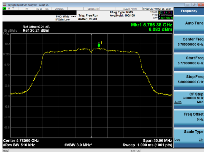
Plot 7-847. PSD CDD Antenna WF7 (20MHz BW 802.11n – Ch. 157, MCS10)
