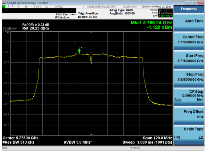
Plot 7-855. PSD CDD Antenna WF7 (80MHz BW 802.11ac – Ch. 155, MCS2)
