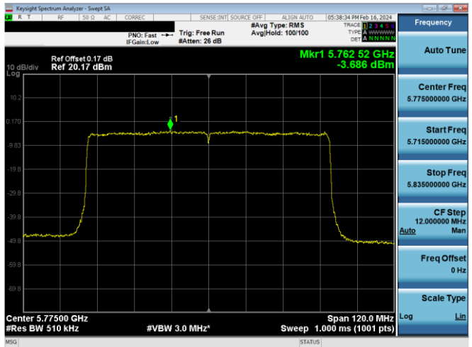
Plot 7-856. PSD CDD Antenna WF5b (80MHz BW 802.11ax(SU) – Ch. 155, MCS2)
