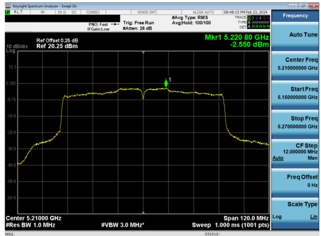
Plot 7-886. ISD PSD CDD Antenna WF7 (80MHz BW 11ac – Ch.42, MCS2)
