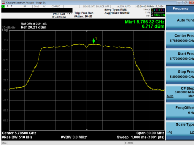
Plot 7-846. PSD CDD Antenna WF5b (20MHz BW 802.11n – Ch. 157, MCS10)
