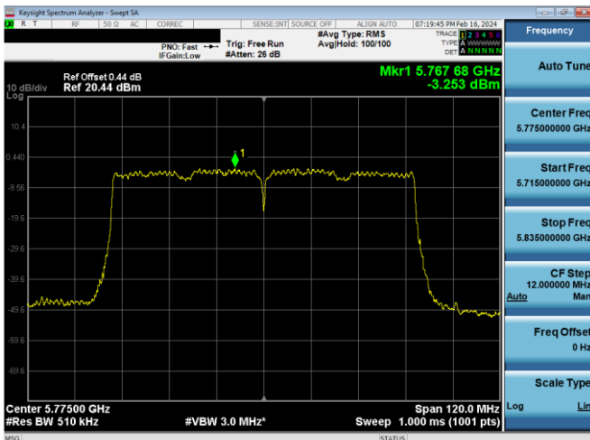
Plot 7-878. PSD CDD Antenna WF5b (80MHz BW 802.11ac – Ch. 155, MCS9)
