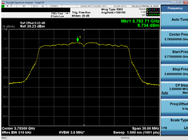
Plot 7-858. PSD CDD Antenna WF5b (20MHz BW 802.11n – Ch. 157, MCS12)
