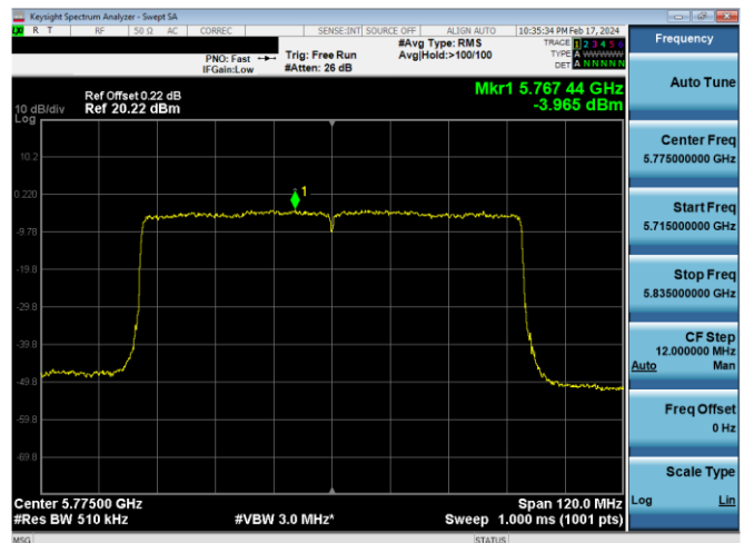
Plot 7-869. PSD CDD Antenna WF7 (80MHz BW 802.11ax(SU) – Ch. 155, MCS4)
