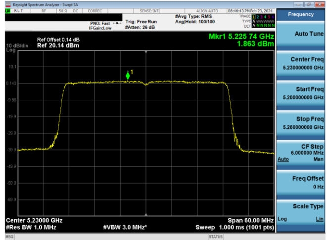
Plot 7-885. ISD PSD CDD Antenna WF7 (40MHz BW 11ax(SU) – Ch.46, MCS2)
