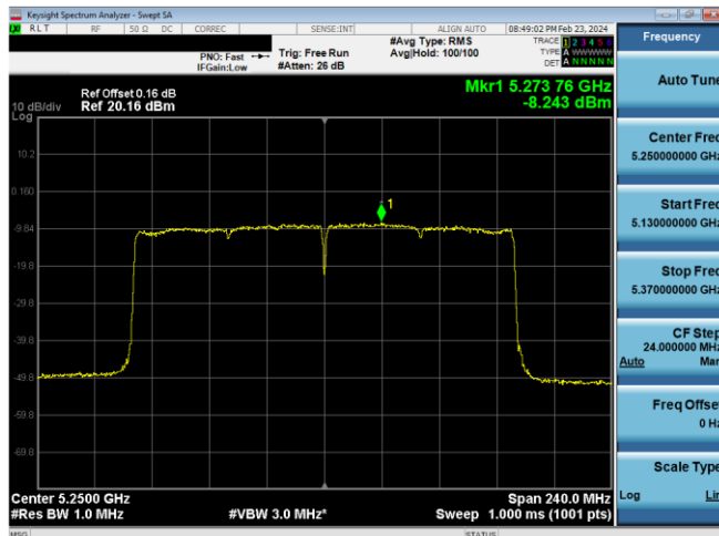
Plot 7-889. ISED PSD CDD Antenna WF7 (160MHz BW 11ax (SU) – Ch.50, MCS2)
