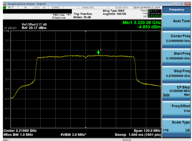
Plot 7-887. ISD PSD CDD Antenna WF7 (80MHz BW 11ax (SU) – Ch.42, MCS2)
