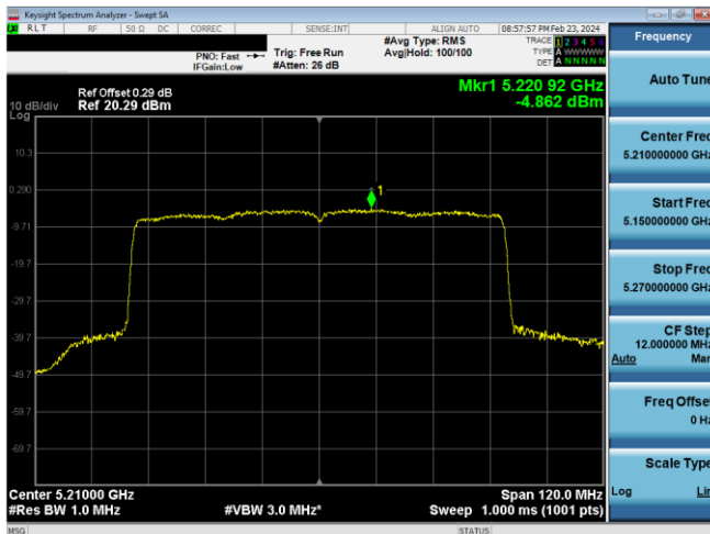
Plot 7-895. ISED PSD CDD Antenna WF7 (80MHz BW 11ax (SU) – Ch.42, MCS4)
