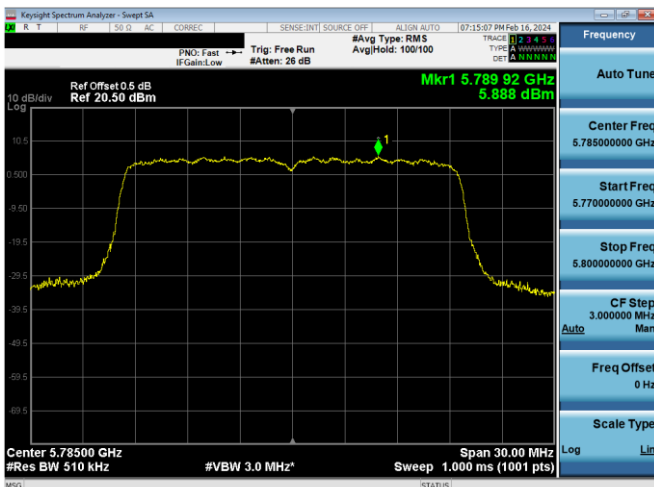
Plot 7-772. PSD CDD Antenna WF5b (20MHz BW 802.11ax(SU) – Ch. 157, MCS11)
