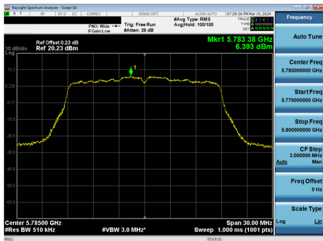
Plot 7-859. PSD CDD Antenna WF7 (20MHz BW 802.11n – Ch. 157, MCS12)
