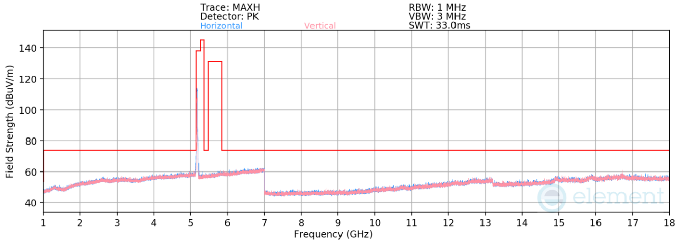
Plot 7-918. Radiated Spurious Emissions above 1GHz Antenna WF5b (802.11ax(SU) – Ch. 36)
