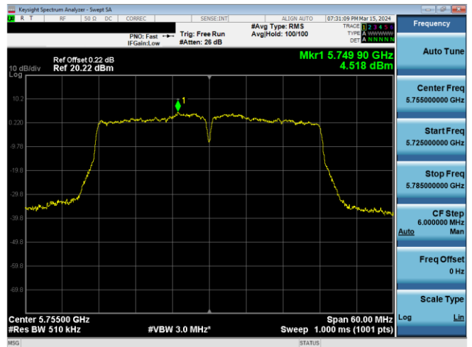
Plot 7-863. PSD CDD Antenna WF7 (40MHz BW 802.11n – Ch. 151, MCS12)
