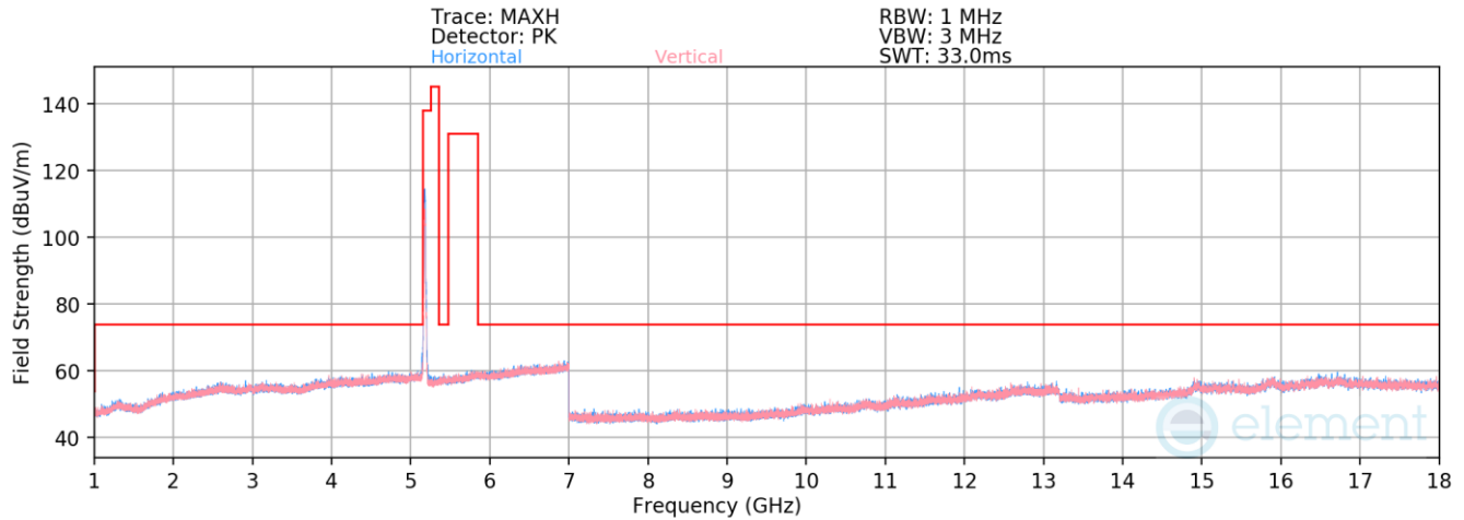
Plot 7-906. Radiated Spurious Emissions above 1GHz Antenna WF5b (802.11n – Ch. 36)
