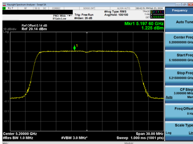
Plot 7-883. ISD PSD SDM Antenna WF7 (20MHz BW 11ax(SU) – Ch.40, MCS2)
