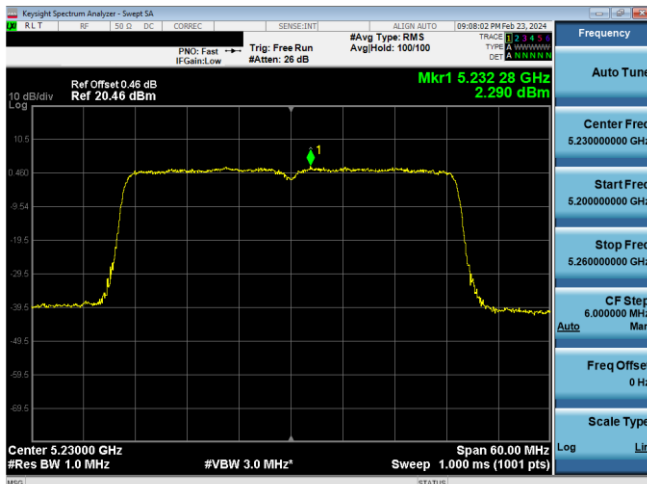
Plot 7-901. ISED PSD SDM Antenna WF7 (40MHz BW 11ax(SU) – Ch.46, MCS11)
