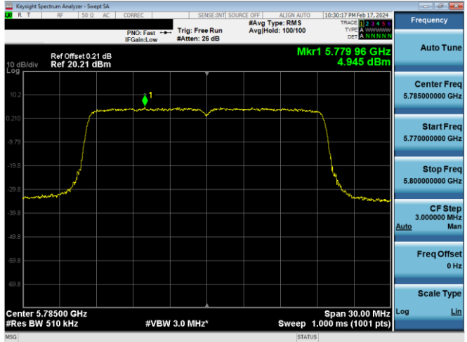
Plot 7-861. PSD CDD Antenna WF7 (20MHz BW 802.11ax(SU) – Ch. 157, MCS4)
