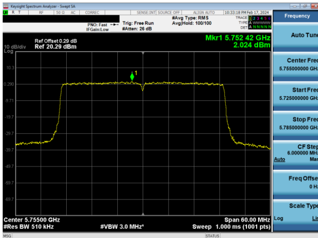
Plot 7-865. PSD CDD Antenna WF7 (40MHz BW 802.11ax(SU) – Ch. 151, MCS4)
