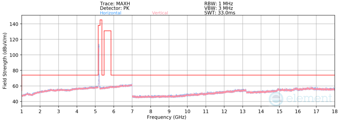
Plot 7-907. Radiated Spurious Emissions above 1GHz Antenna WF5b (802.11n – Ch. 40)
