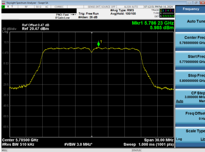
Plot 7-770. PSD CDD Antenna WF5b (20MHz BW 802.11n – Ch. 157, MCS15)
