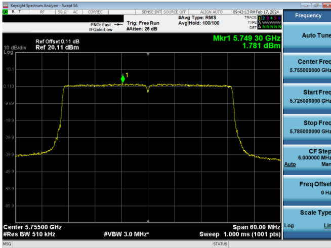
Plot 7-853. PSD CDD Antenna WF7 (40MHz BW 802.11ax(SU) – Ch. 151, MCS2)
