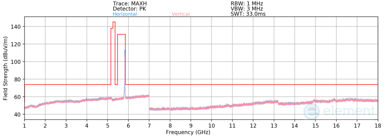
Plot 7-917. Radiated Spurious Emissions above 1GHz Antenna WF5b (802.11n – Ch. 165)
