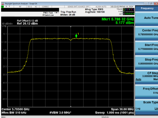
Plot 7-848. PSD CDD Antenna WF5b (20MHz BW 802.11ax(SU) – Ch. 157, MCS2)
