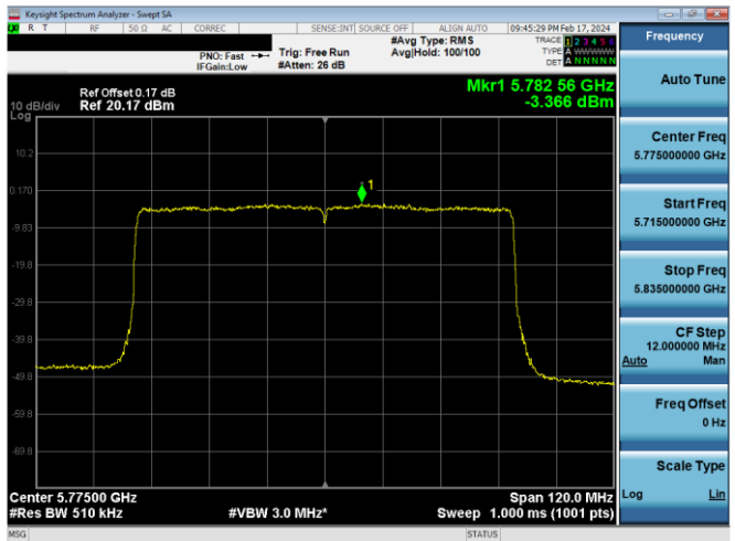
Plot 7-857. PSD CDD Antenna WF7 (80MHz BW 802.11ax(SU) – Ch. 155, MCS2)
