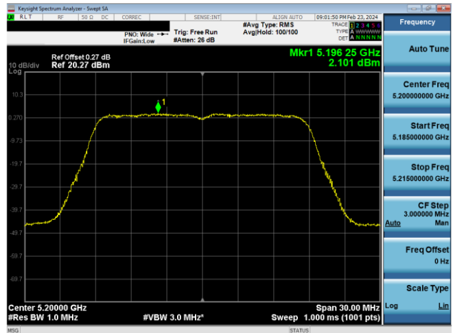
Plot 7-898. ISED PSD CDD Antenna WF7 (20MHz BW 11n – Ch.40, MCS15)
