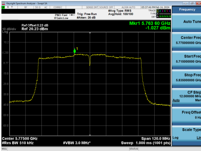
Plot 7-854. PSD CDD Antenna WF5b (80MHz BW 802.11ac – Ch. 155, MCS2)
