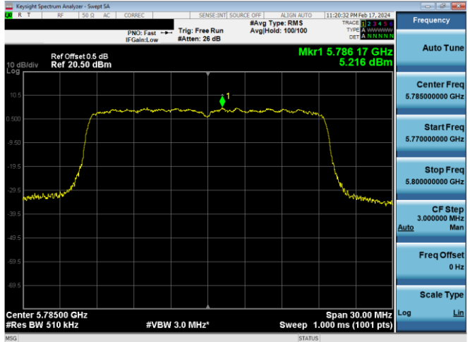
Plot 7-773. PSD CDD Antenna WF7 (20MHz BW 802.11ax(SU) – Ch. 157, MCS11)
