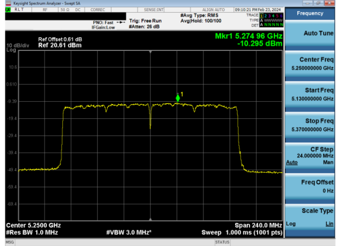
Plot 7-905. ISED PSD CDD Antenna WF7 (160MHz BW 11ax (SU) – Ch.50, MCS11)
