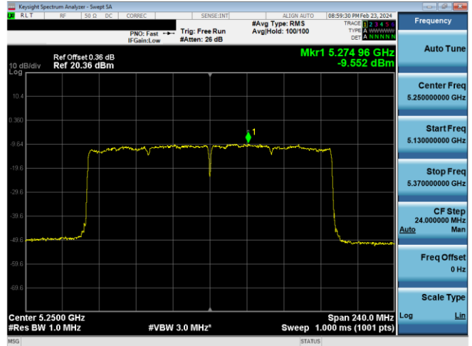
Plot 7-897. ISED CDD SDM Antenna WF7 (160MHz BW 11ax (SU) – Ch.50, MCS4)
