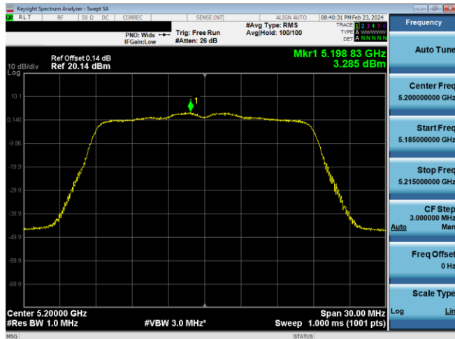
Plot 7-882. ISD PSD SDM Antenna WF7 (20MHz BW 11n – Ch.40, MCS10)
