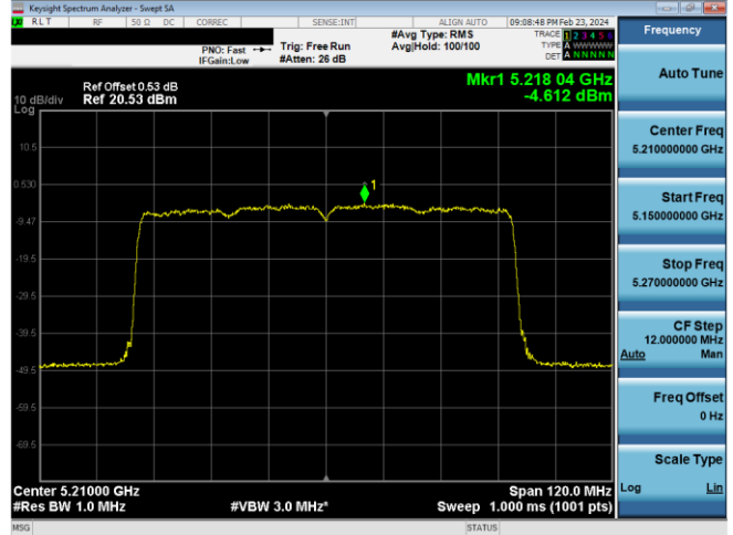
Plot 7-903. ISED PSD CDD Antenna WF7 (80MHz BW 11ax (SU) – Ch.42, MCS11)
