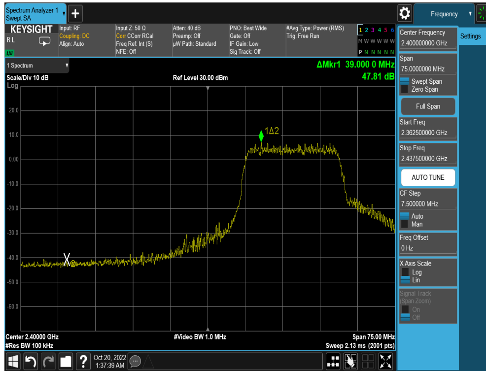
Plot 7-57. Band Edge Plot (802.11n MCS7 – Ch. 2)
