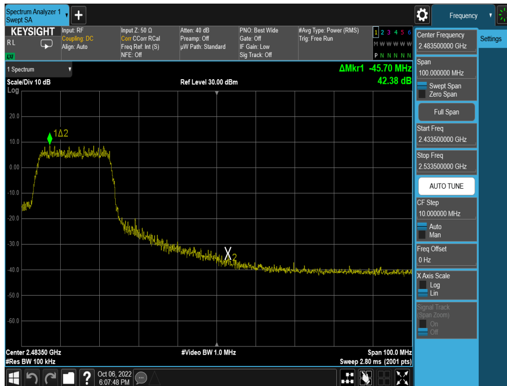
Plot 7-58. Band Edge Plot (802.11n MCS7 – Ch. 8)
