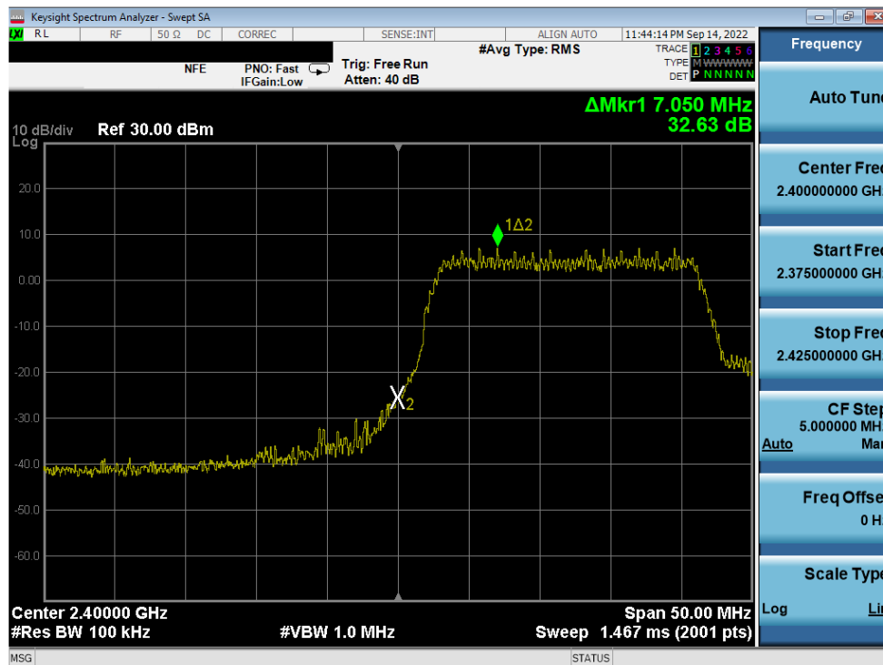
Plot 7-56. Band Edge Plot (802.11n MCS7 – Ch. 1)
