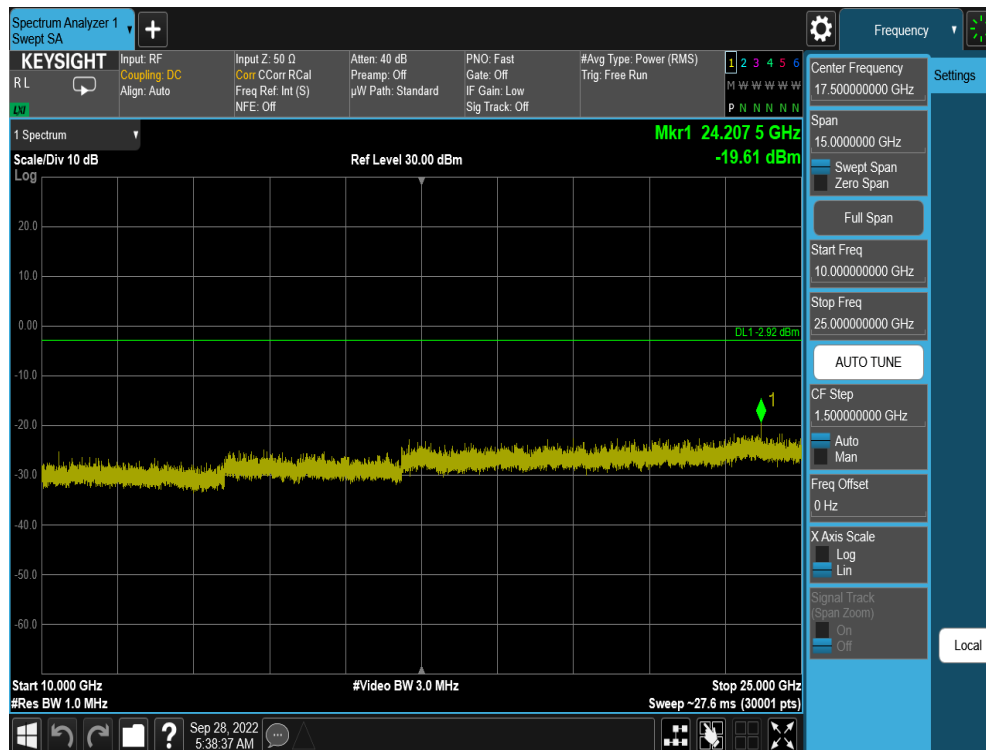
Plot 7-69. Conducted Spurious Plot (802.11b – Ch. 11)
