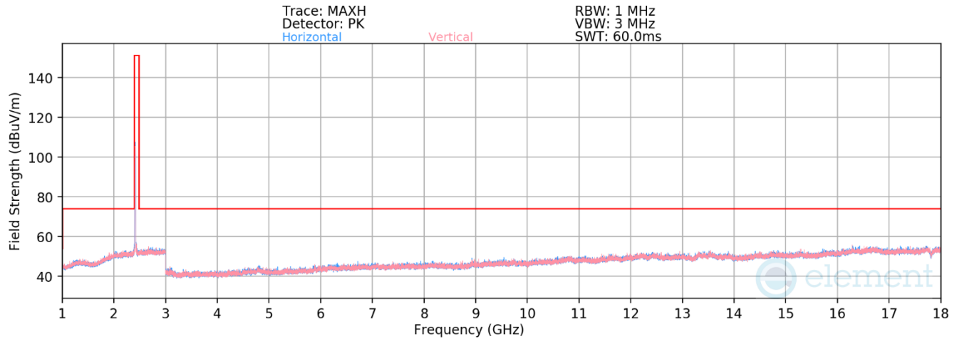
Plot 7-70. Radiated Spurious Emissions above 1GHz (802.11b – Ch. 1)
