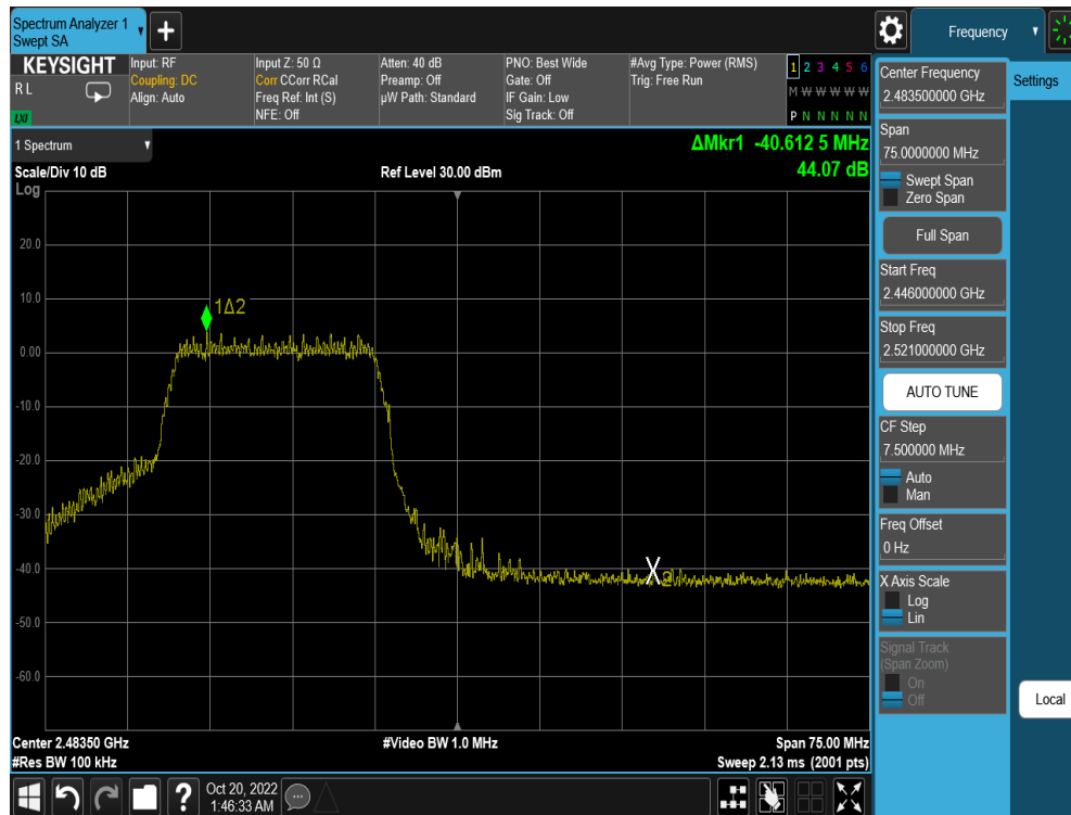
Plot 7-62. Band Edge Plot (802.11n MCS7 – Ch. 12)
