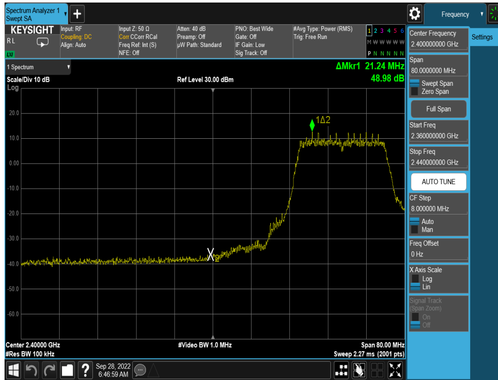
Plot 7-47. Band Edge Plot (802.11n MCS0 – Ch. 4)
