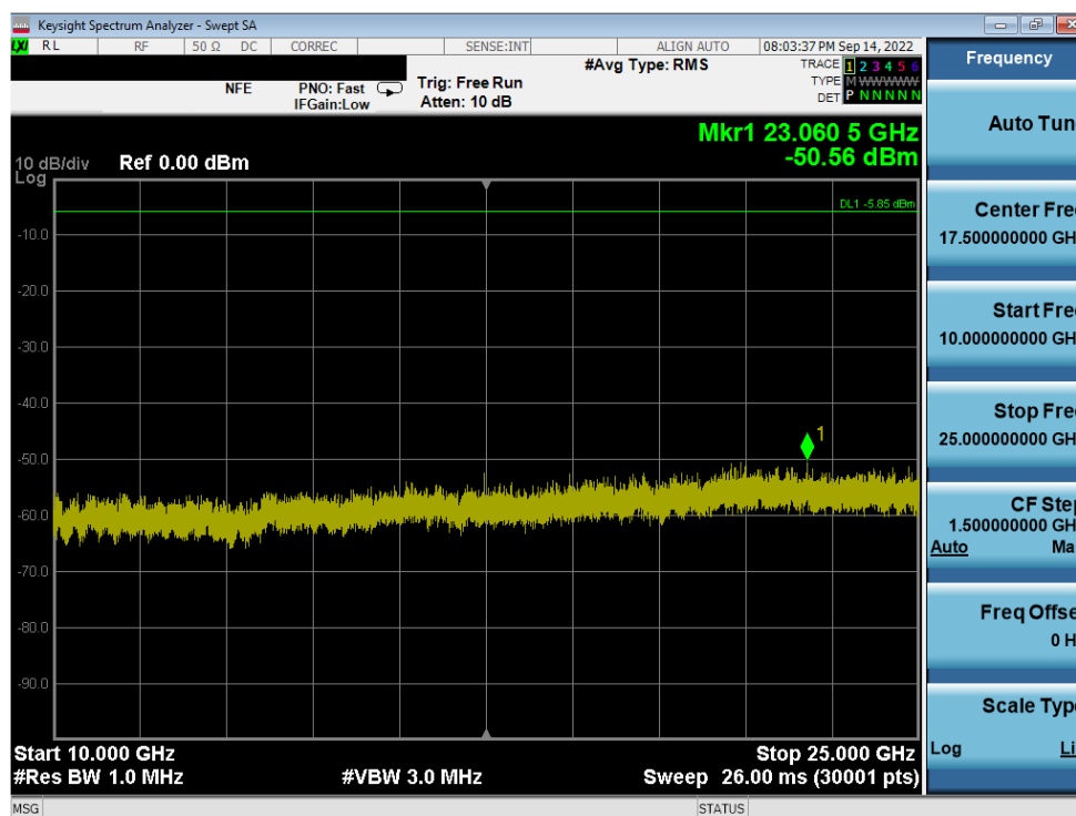
Plot 7-67. Conducted Spurious Plot (802.11b – Ch. 6)
