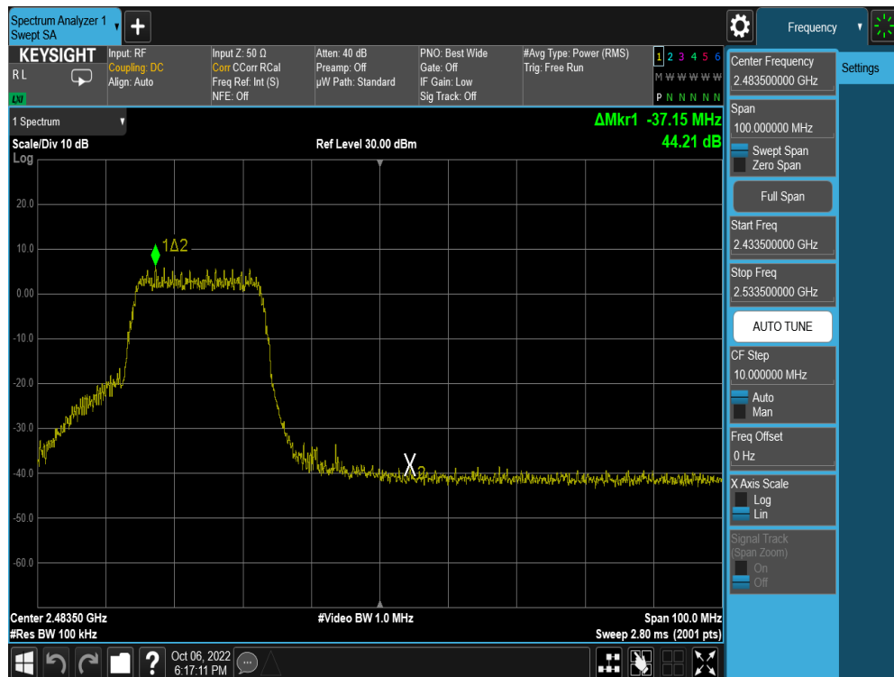
Plot 7-60. Band Edge Plot (802.11n MCS7 – Ch. 10)
