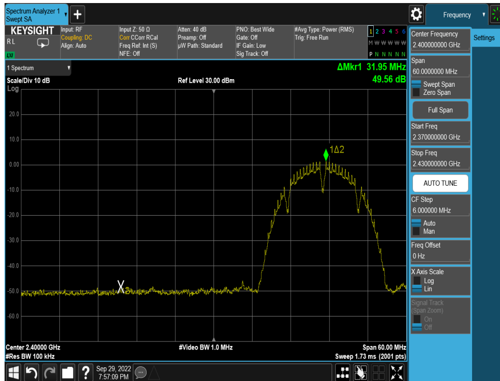
Plot 7-26. Band Edge Plot (802.11b – Ch. 2)
