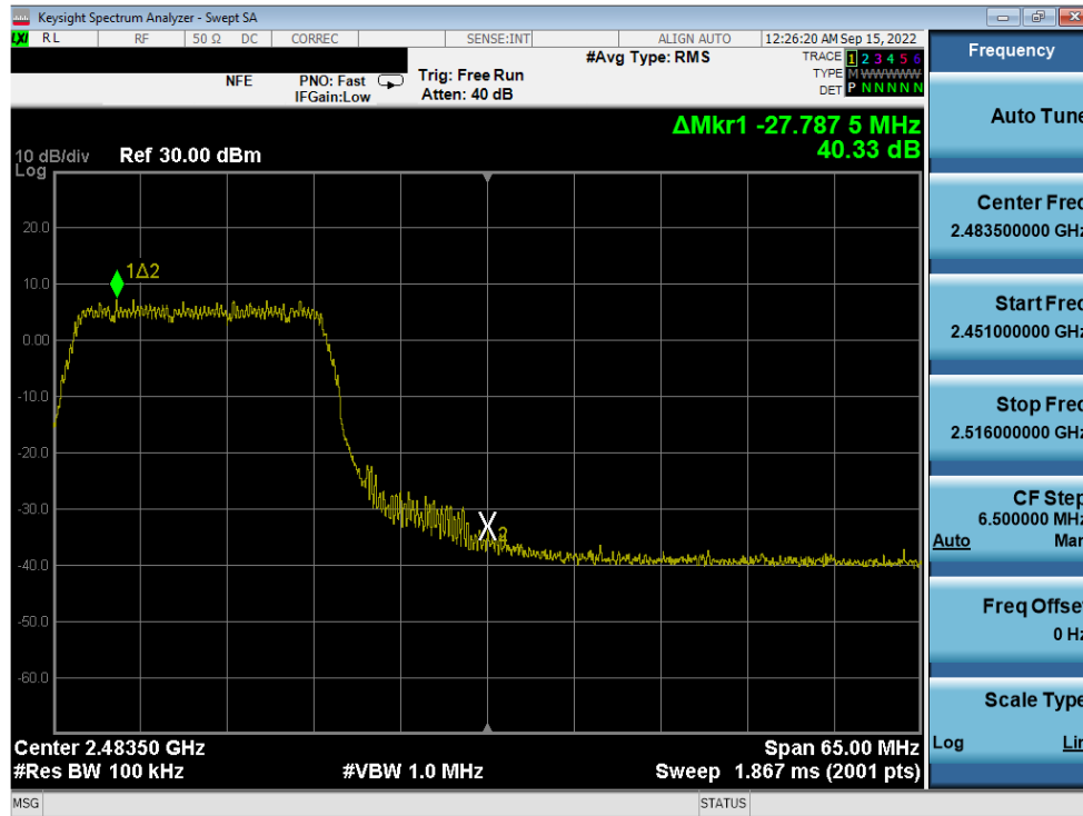
Plot 7-61. Band Edge Plot (802.11n MCS7 – Ch. 11)
