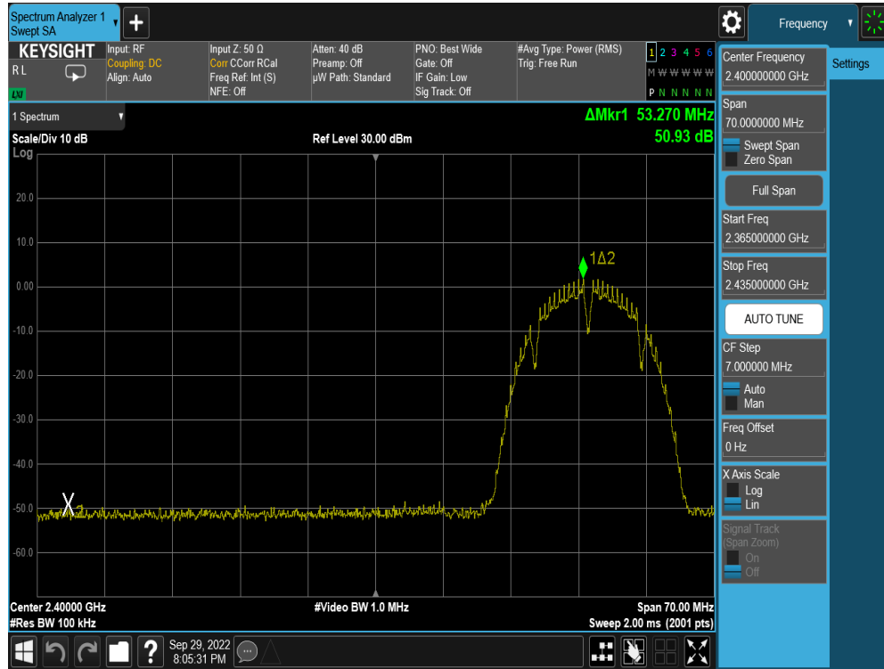
Plot 7-27. Band Edge Plot (802.11b – Ch. 3)
