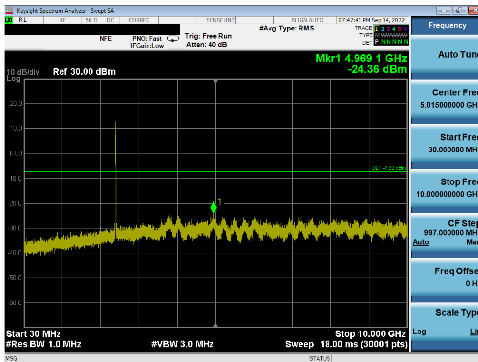
Plot 7-64. Conducted Spurious Plot (802.11b – Ch. 1)
