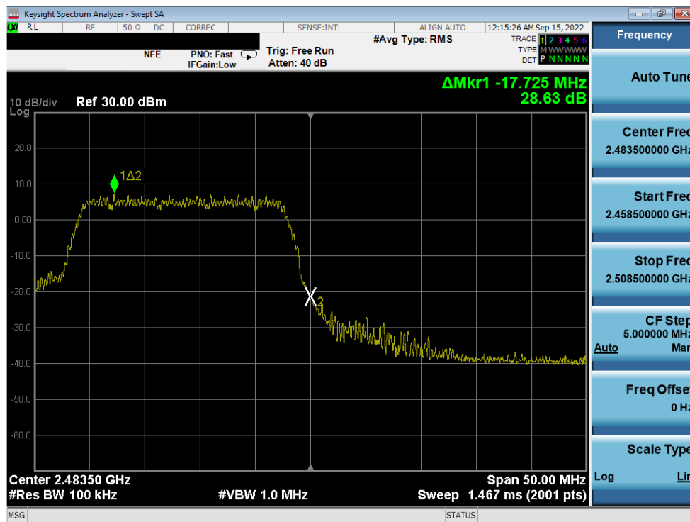
Plot 7-63. Band Edge Plot (802.11n MCS7 – Ch. 13)
