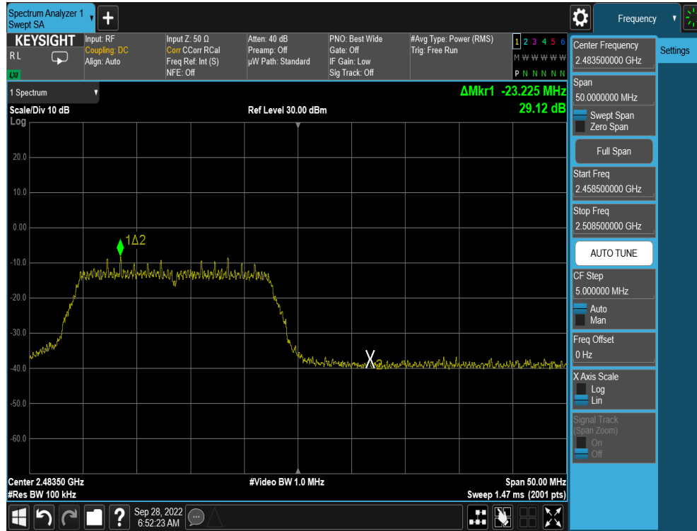
Plot 7-55. Band Edge Plot (802.11n MCS0– Ch. 13)
