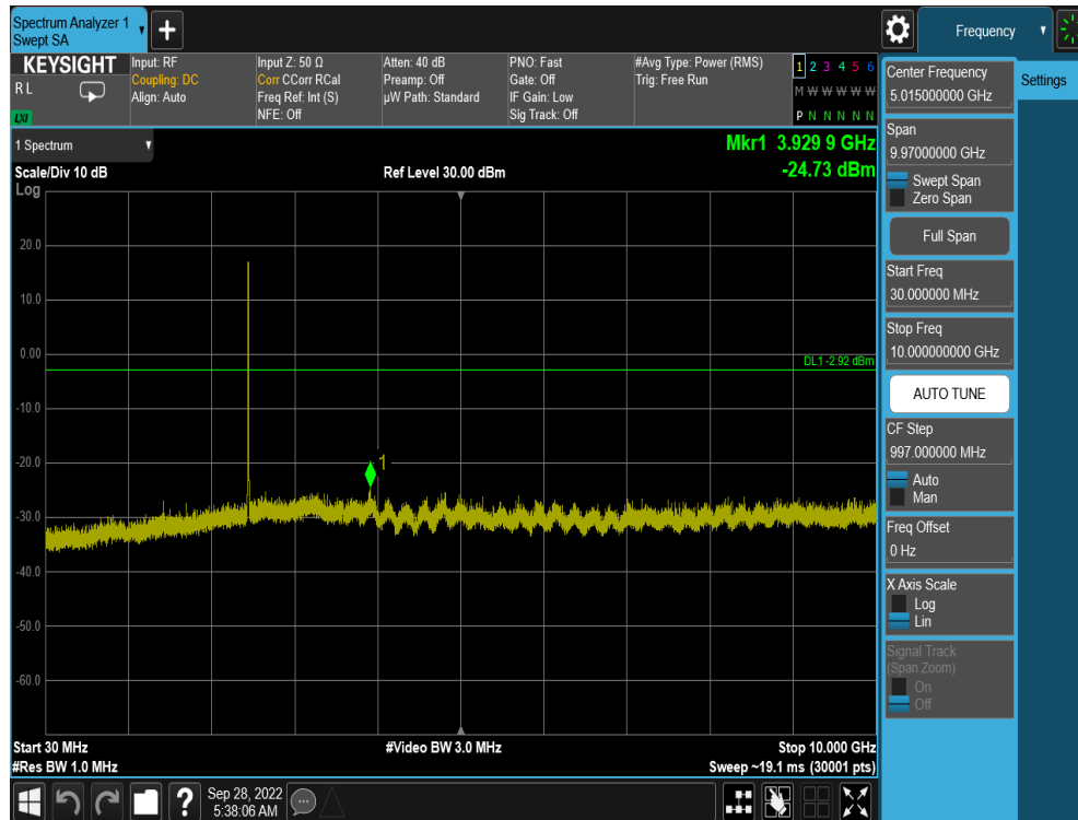
Plot 7-68. Conducted Spurious Plot (802.11b – Ch. 11)
