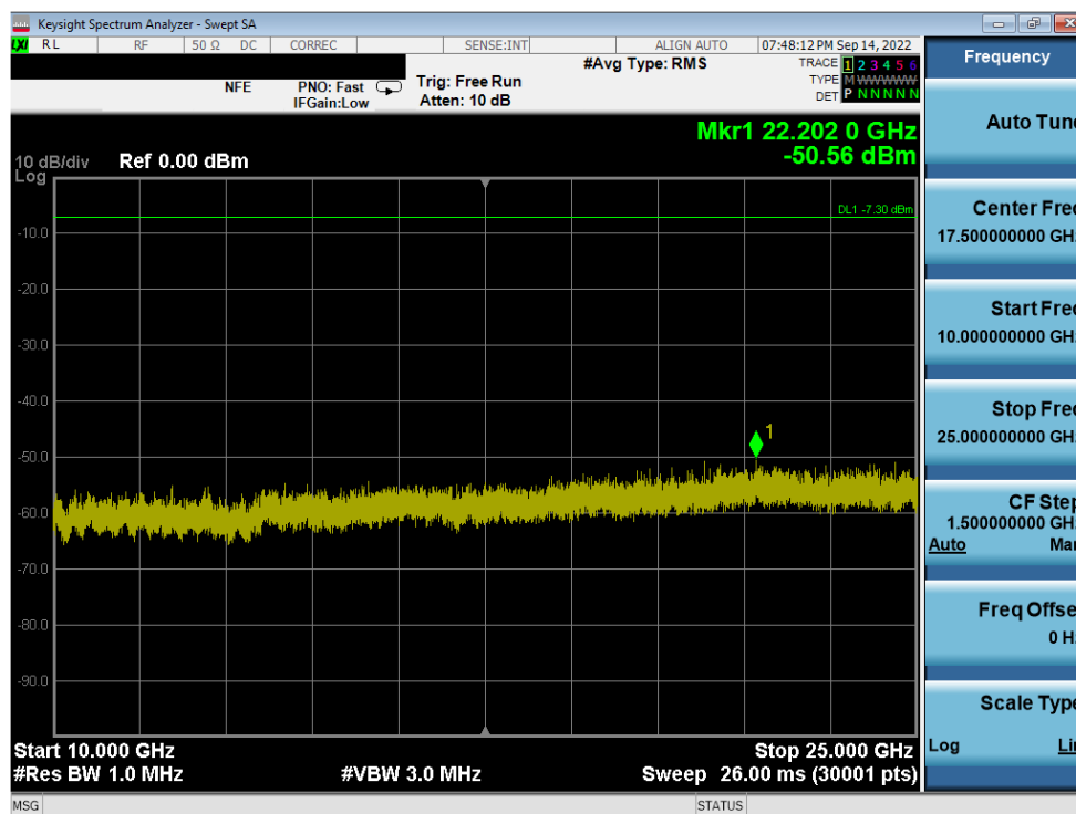
Plot 7-65. Conducted Spurious Plot (802.11b – Ch. 1)
