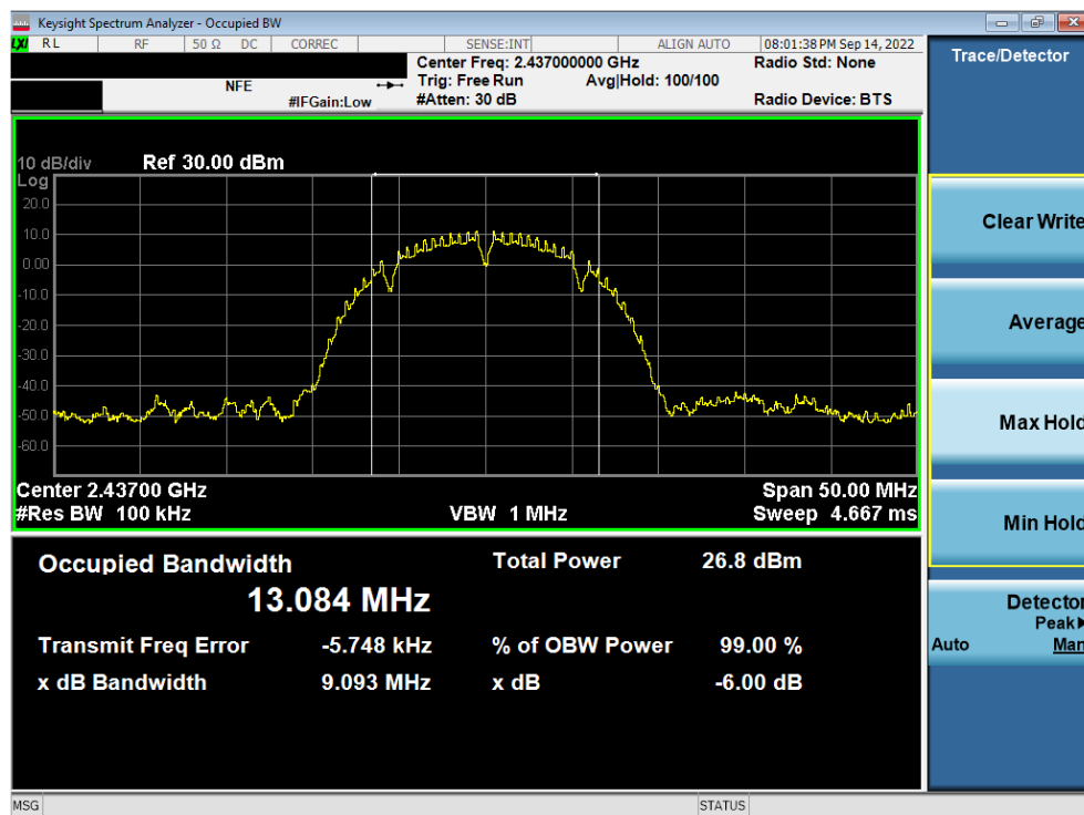
Plot 7-2. 6dB BW and 99% OBW Plot (802.11b – Ch. 6)
