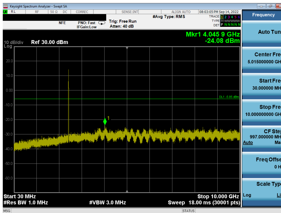
Plot 7-66. Conducted Spurious Plot (802.11b – Ch. 6)
