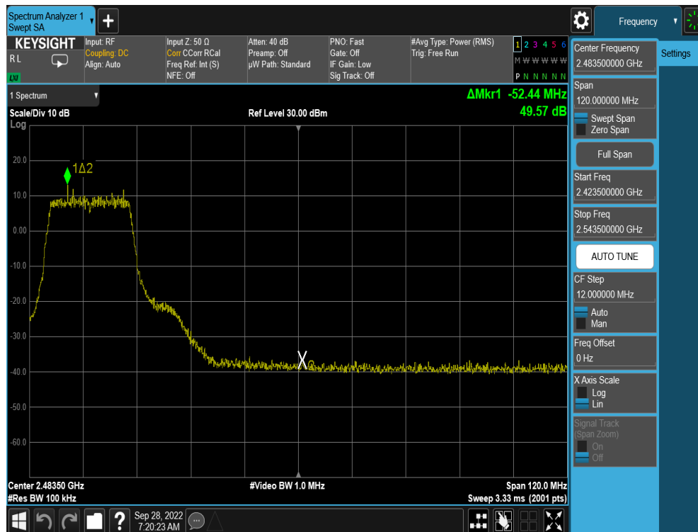
Plot 7-48. Band Edge Plot (802.11n MCS0 – Ch. 6)
