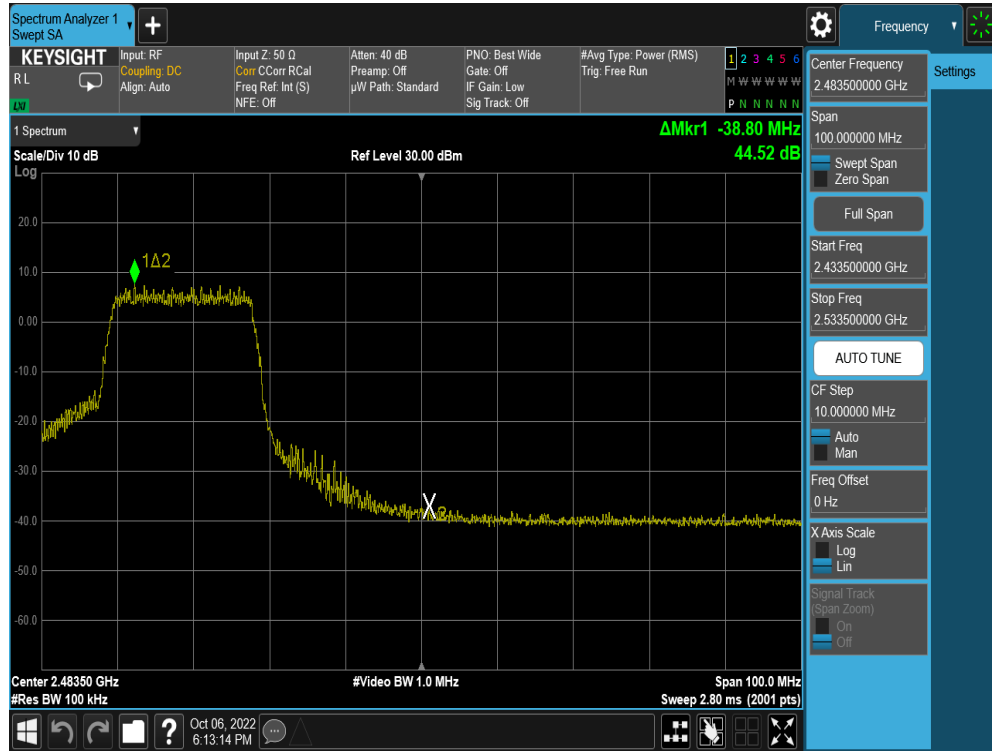
Plot 7-59. Band Edge Plot (802.11n MCS7 – Ch. 9)
