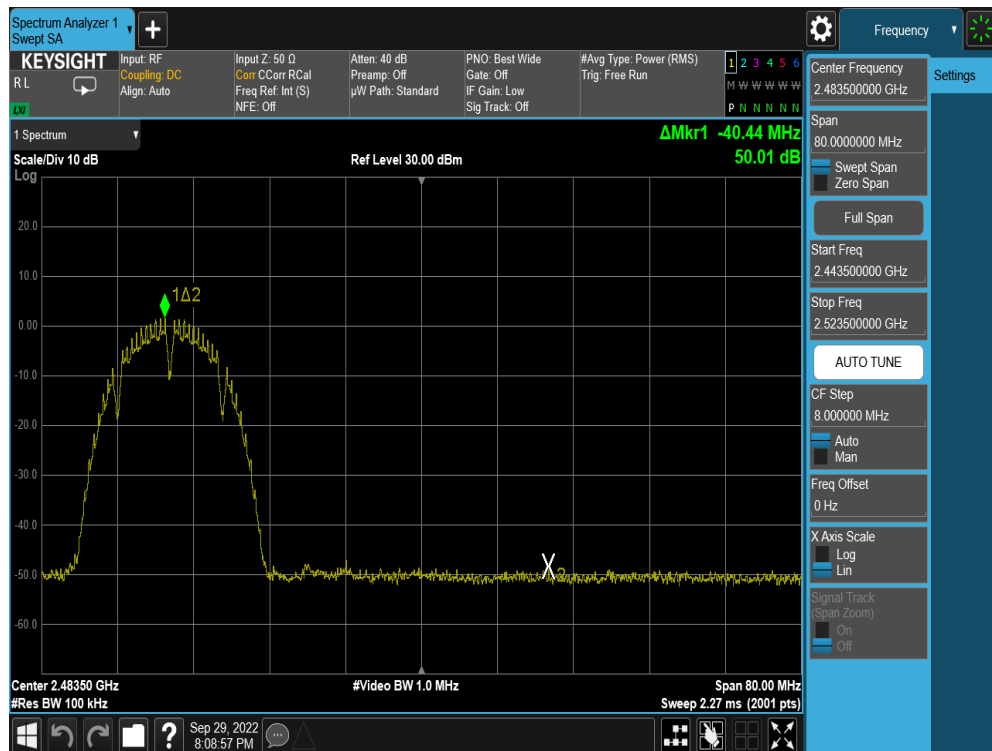
Plot 7-28. Band Edge Plot (802.11b – Ch. 10)
