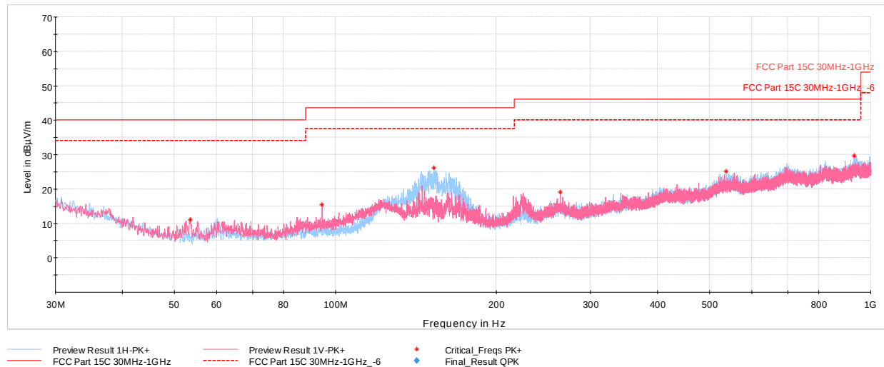
Plot 7-41. Radiated Spurious Emissions Below 1GHz (GFSK ePA – Ch.0, with AC Power Cable)
