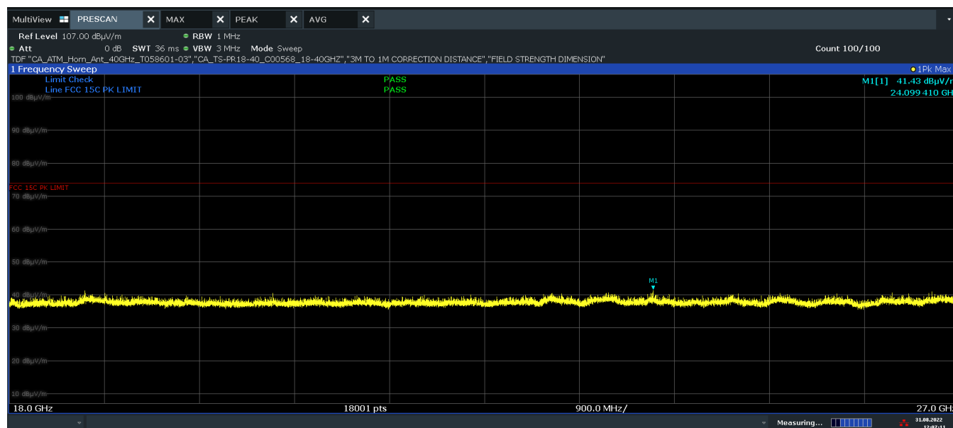
Plot 7-33. Radiated Spurious Emissions Above 18GHz (BT GFSK ePA – Ch. 0, Ant. Pol H)
