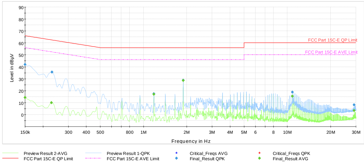
Plot 7-44. AC Line-Conducted Test Plot (N, GFSK ePA – Ch.0, with AC Power Cable)
