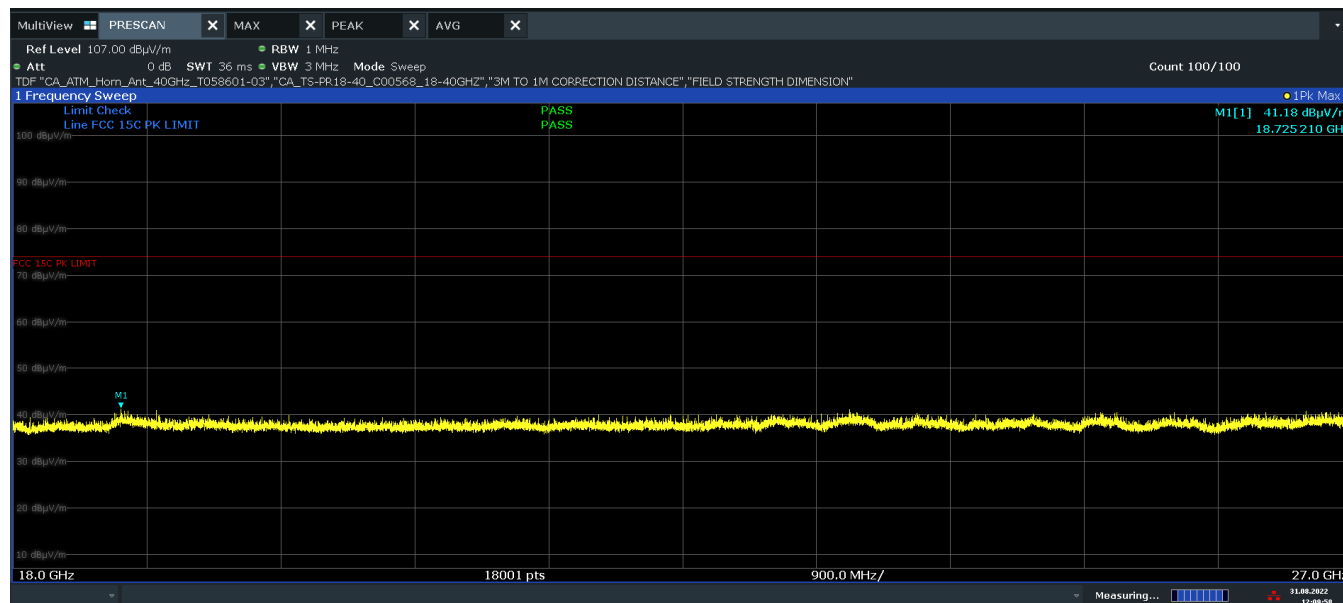
Plot 7-32. Radiated Spurious Emissions Above 18GHz (BT GFSK ePA – Ch. 0, Ant. Pol V)
