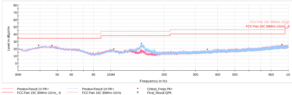
Plot 7-42. Radiated Spurious Emissions Below 1GHz Simultaneous Transmission with AC Power Cable
