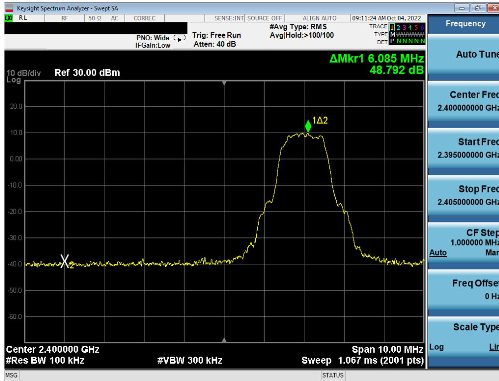
Plot 7-11. Band Edge Plot (Bluetooth with Hopping Disabled, 8DPSK, ePA – Ch. 0)
