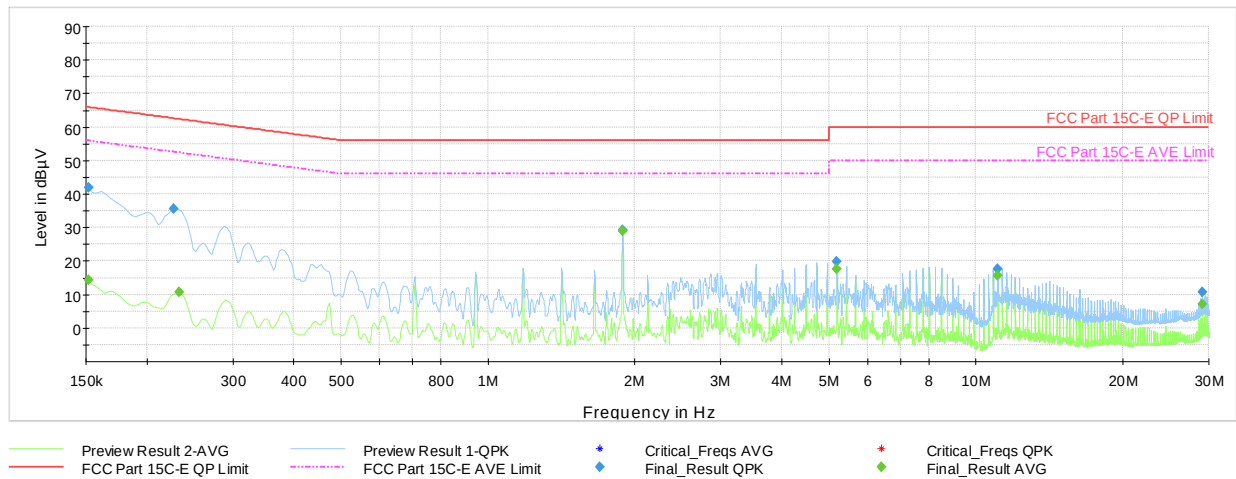
Plot 7-43. AC Line-Conducted Test Plot (L1, GFSK ePA – Ch.0, with AC Power Cable)
