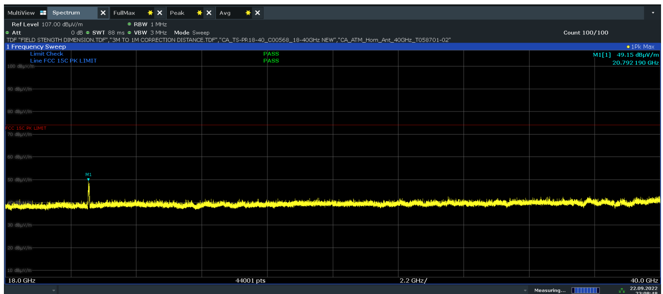
Plot 7-36. Radiated Spurious Emissions Simultaneous Transmission Above 18GHz Ant. Pol. V
