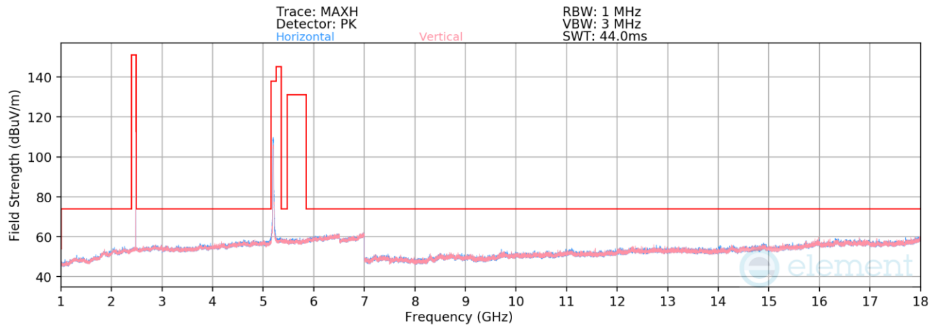
Plot 7-34. Radiated Spurious Emissions Simultaneous Transmission above 1GHz
