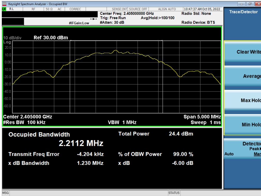
Plot 7-1. 6dB BW & 99% OBW Plot (802.15.4, Ch. 11)
