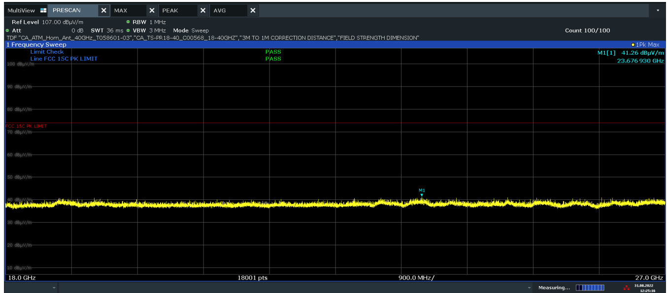
Plot 7-32. Radiated Spurious Emissions Above 18GHz (4Mbps, HDR4, ePA – Ch. 1, Ant. Pol V)
