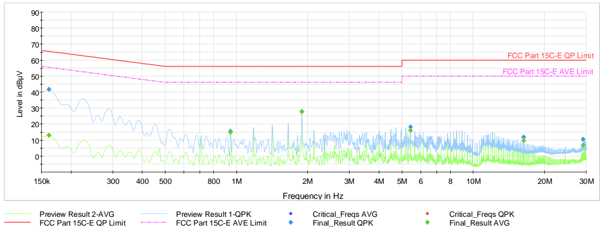
Plot 7-41. AC Line Conducted Plot with Bluetooth HDR (L1, 4Mbps ePA - Ch.1 with AC Power Cable)
