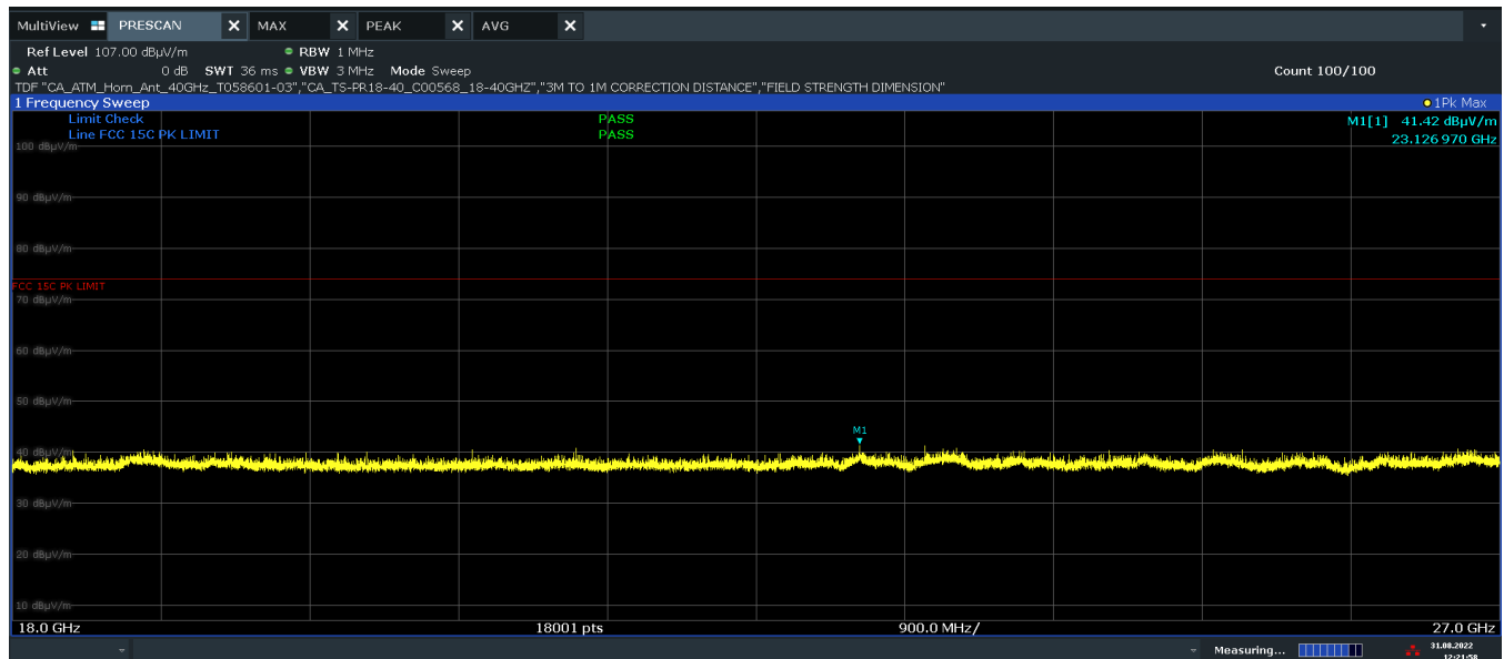
Plot 7-33. Radiated Spurious Emissions Above 18GHz (4Mbps, HDR4, ePA – Ch. 1, Ant. Pol H)
