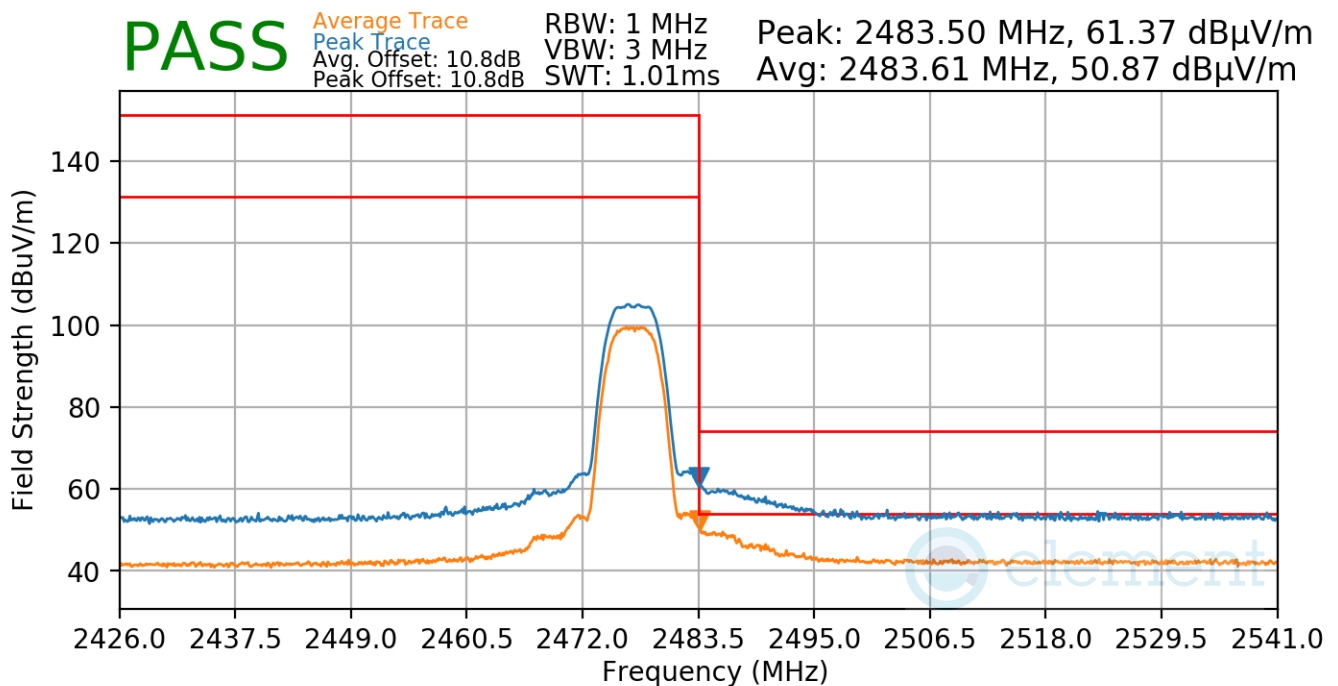
Plot 7-38. Radiated Restricted Upper Band Edge Measurement
