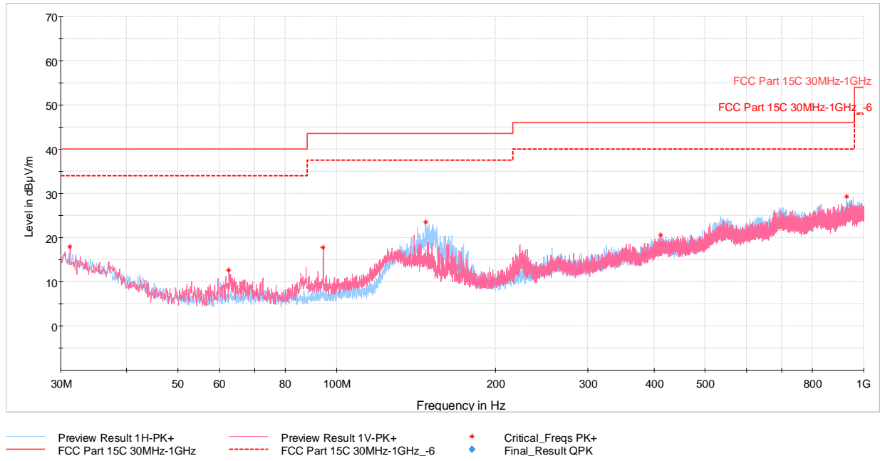
Plot 7-40. Radiated Spurious Emissions Below 1GHz (4Mbps, ePA – Ch.1 with AC Power Cable)
