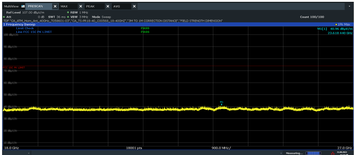
Plot 7-33. Radiated Spurious Emissions Above 18GHz V Polarity (1Mbps ePA – Ch. 19)
