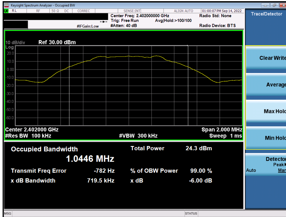
Plot 7-1. 6dB BW & 99% OBW Plot (Bluetooth (LE), 1Mbps, ePA – Ch. 0)
