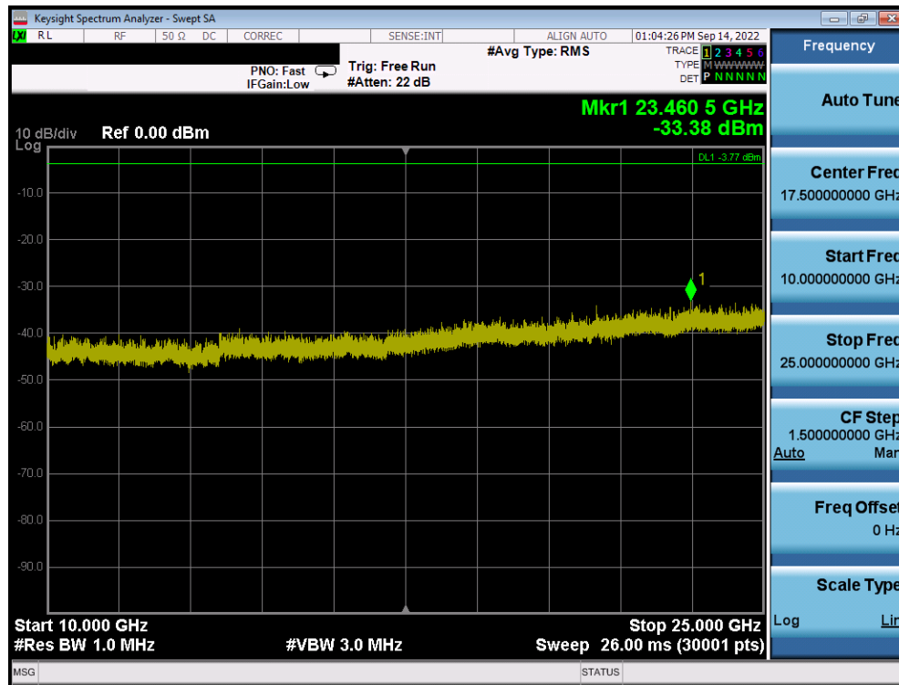
Plot 7-24. Conducted Spurious Plot (Bluetooth (LE), 1Mbps, ePA – Ch. 0)
