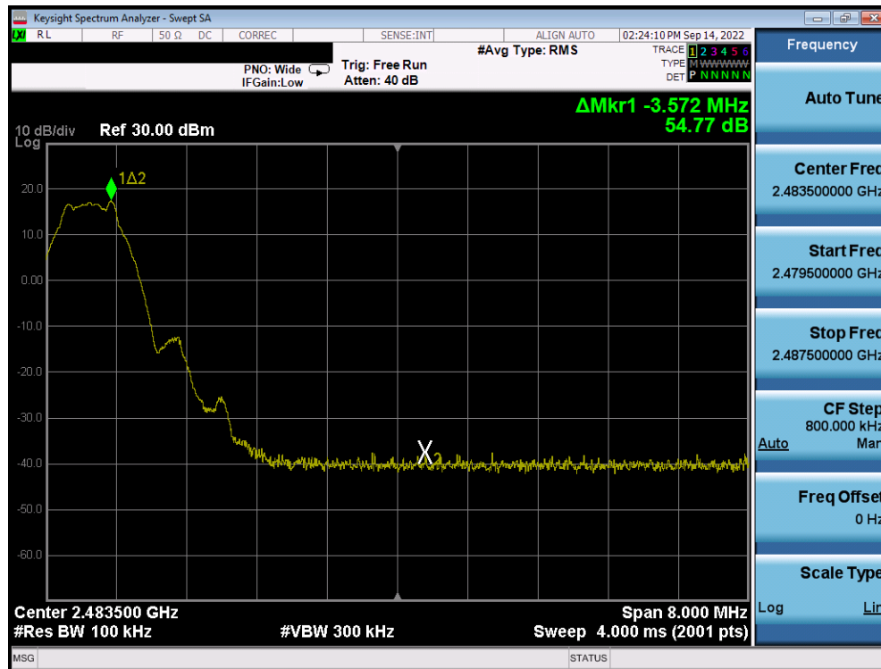
Plot 7-20. Band Edge Plot (Bluetooth (LE), 1Mbps, ePA – Ch. 39)
