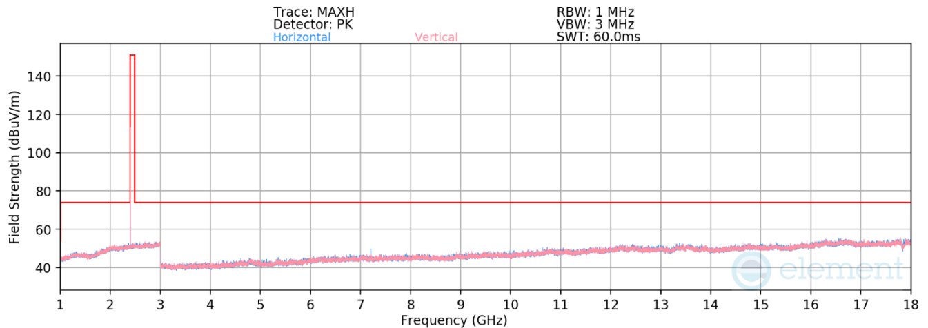
Plot 7-29. Radiated Spurious Emissions 1-18GHz (1Mbps, ePA – Ch. 0)
