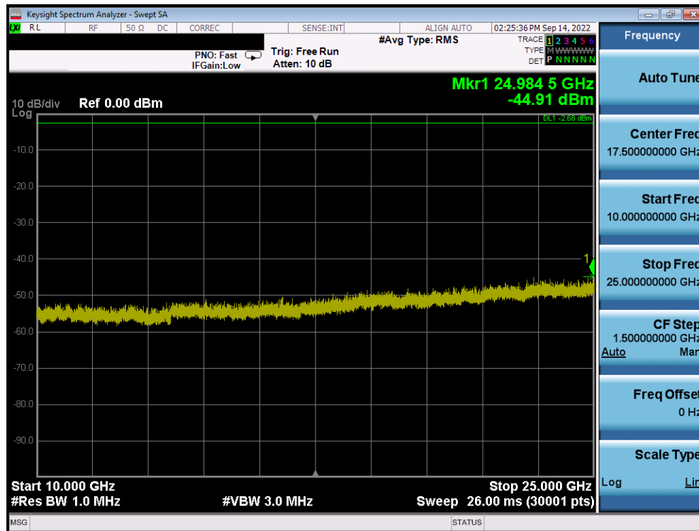
Plot 7-28. Conducted Spurious Plot (Bluetooth (LE), 1Mbps, ePA – Ch. 39)
