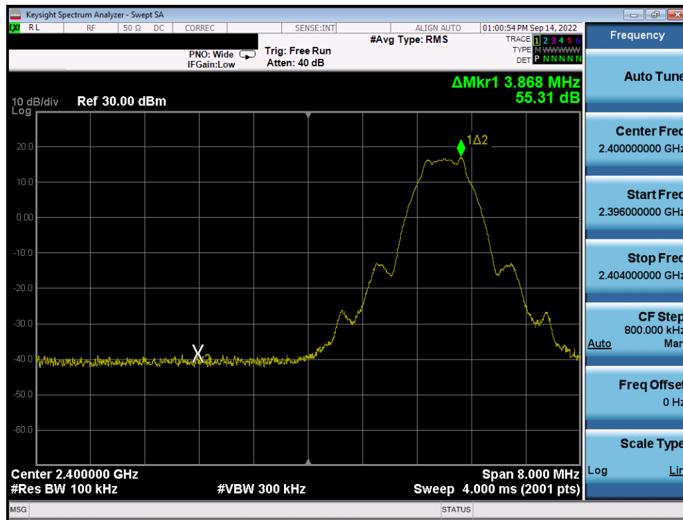
Plot 7-19. Band Edge Plot (Bluetooth (LE), 1Mbps, ePA – Ch. 0)
