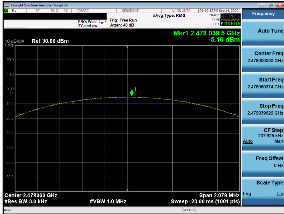
Plot 7-15. Power Spectral Density Plot (Bluetooth (LE), 2Mbps, ePA – Ch. 38)
