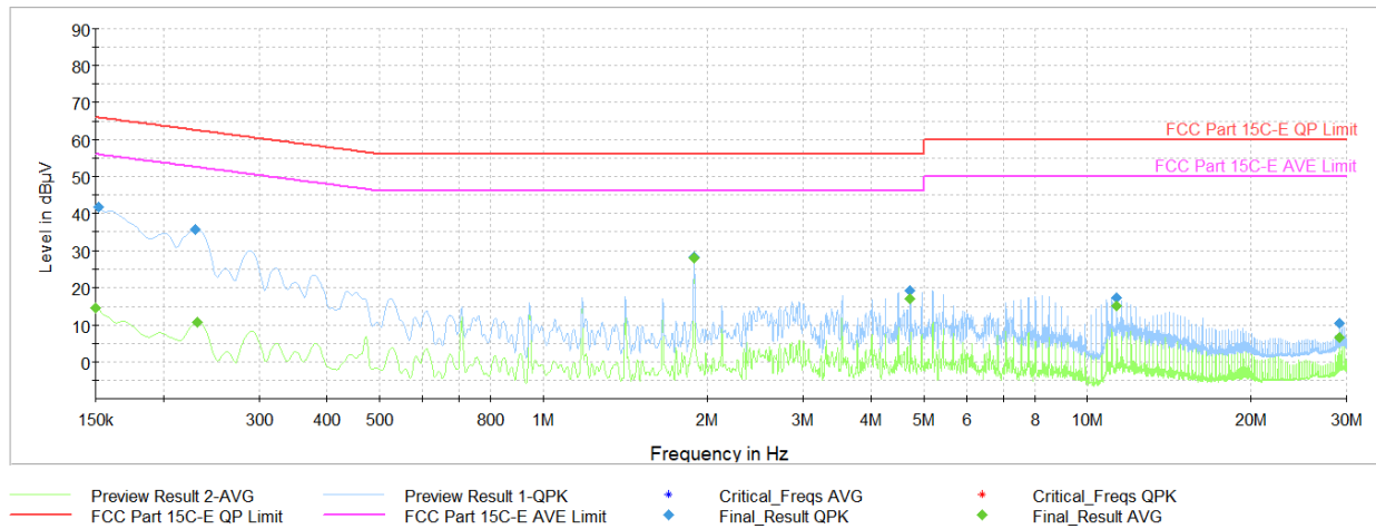
Plot 7-39. AC Line Conducted Plot with Bluetooth LE (L1, 1Mbps ePA – Ch.19 with AC Power Cable)
