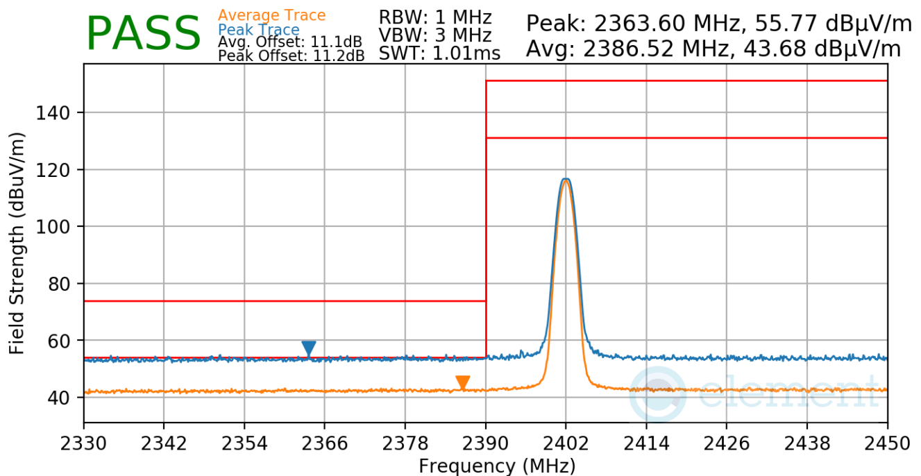
Plot 7-34. Radiated Restricted Lower Band Edge Measurement (Average & Peak)
