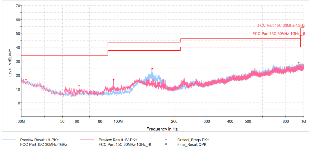
Plot 7-38. Radiated Spurious Emissions Below 1GHz (1Mbps, ePA – Ch.19, Pol. H & V, with AC Power Cable)
