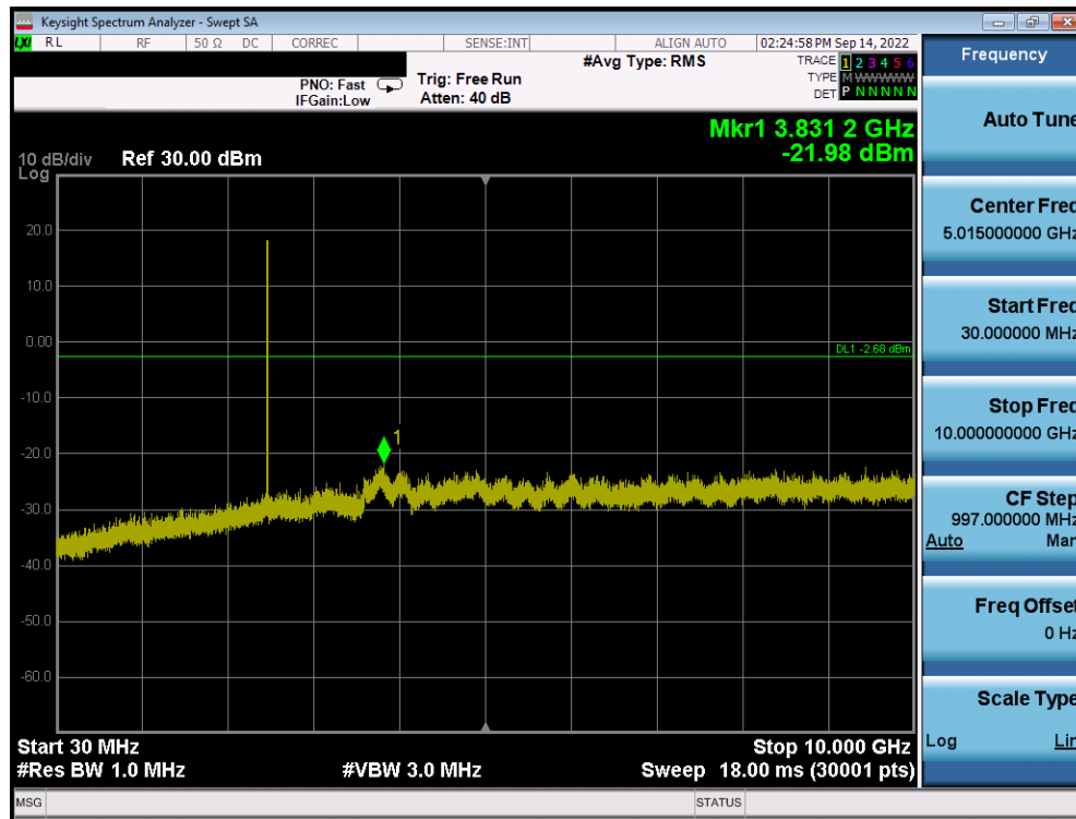
Plot 7-27. Conducted Spurious Plot (Bluetooth (LE), 1Mbps, ePA – Ch. 39)
