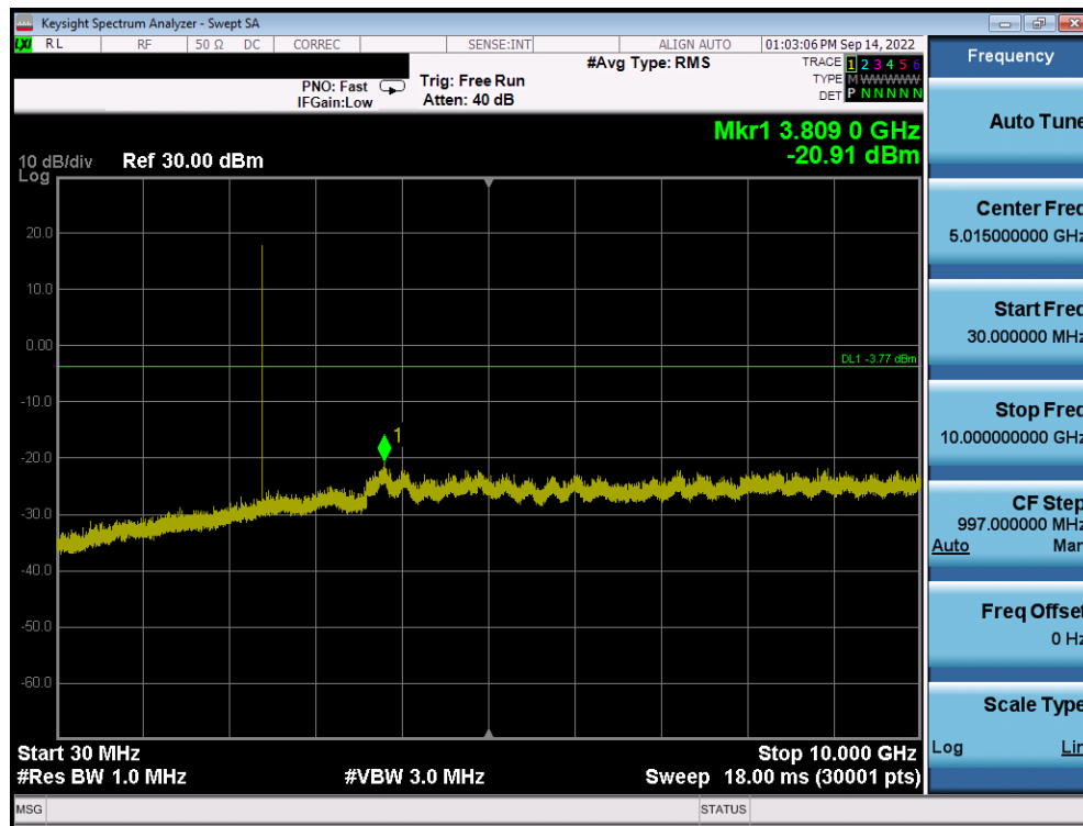
Plot 7-23. Conducted Spurious Plot (Bluetooth (LE), 1Mbps, ePA – Ch. 0)
