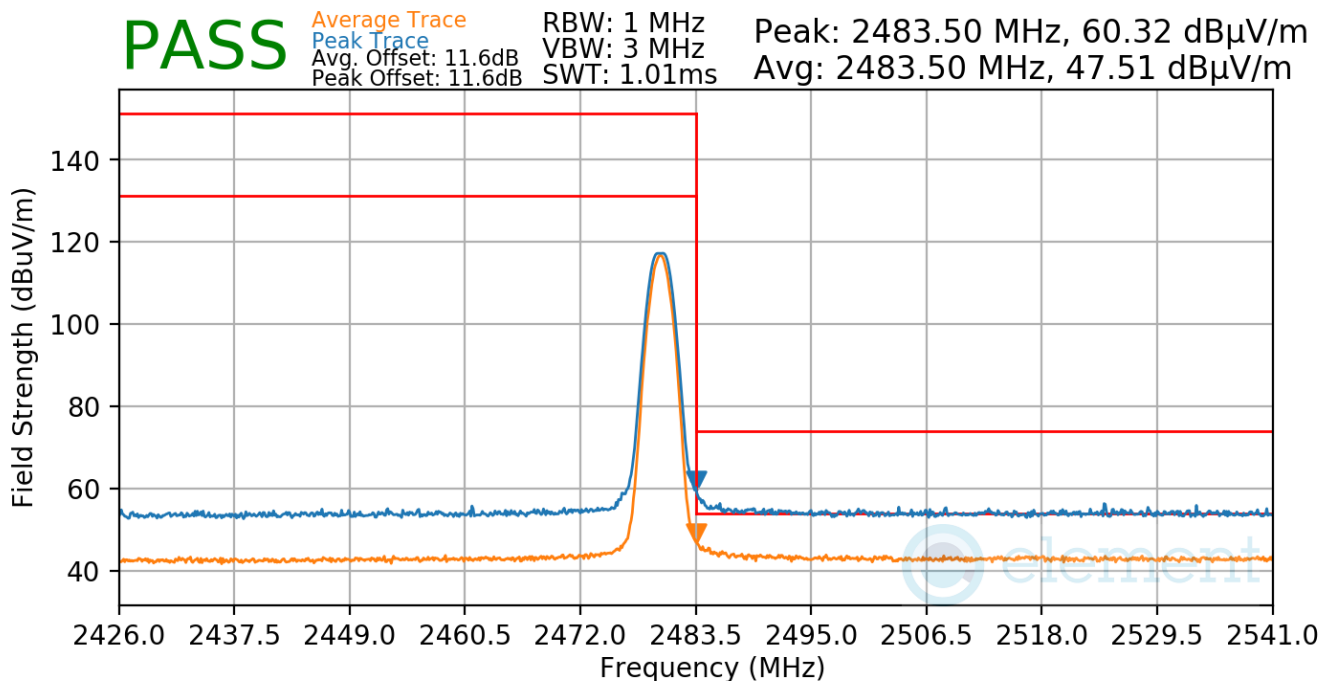
Plot 7-35. Radiated Restricted Upper Band Edge Measurement (Average & Peak)
