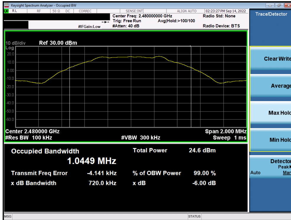
Plot 7-3. 6dB BW & 99% OBW Plot (Bluetooth (LE), 1Mbps, ePA – Ch. 39)
