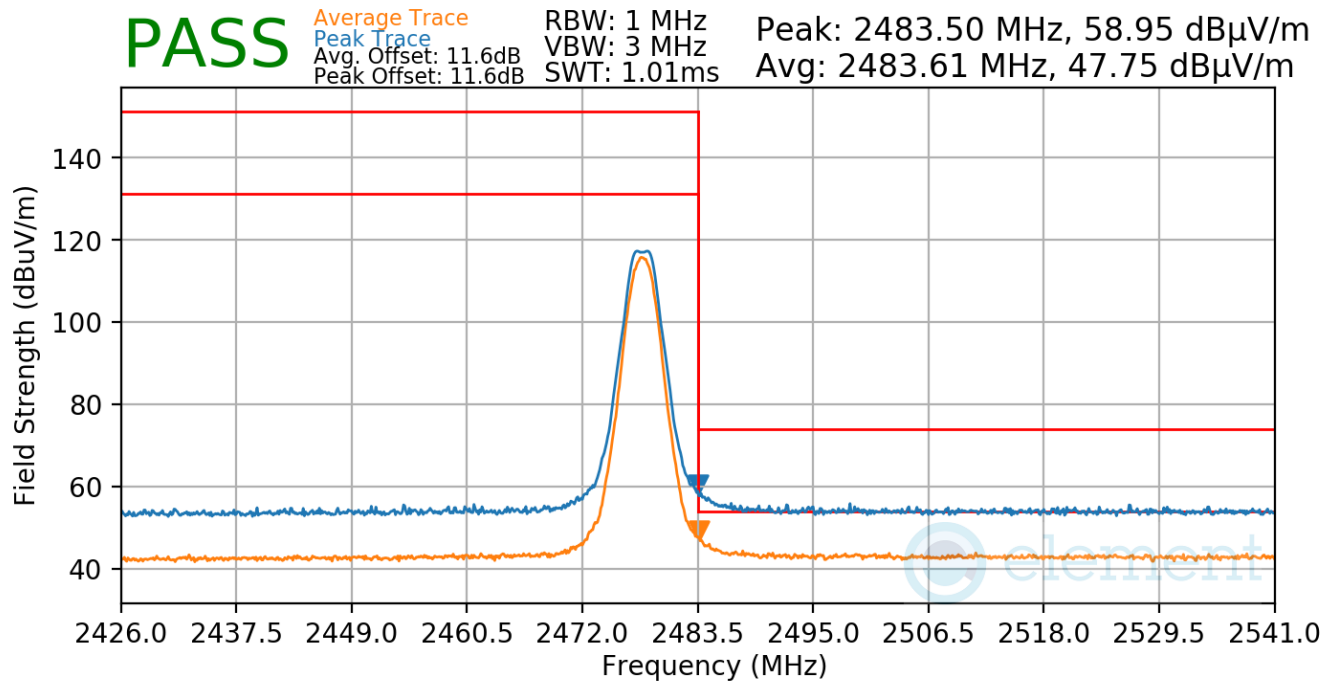
Plot 7-37. Radiated Restricted Upper Band Edge Measurement (Average & Peak)
