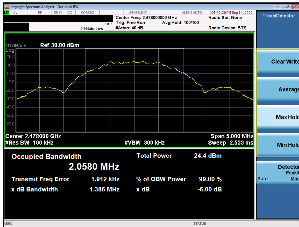
Plot 7-6. 6dB BW & 99% OBW Plot (Bluetooth (LE), 2Mbps, ePA – Ch. 38)
