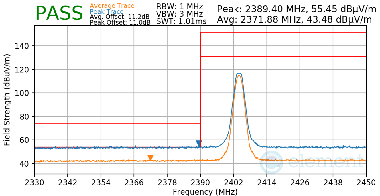
Plot 7-36. Radiated Restricted Lower Band Edge Measurement (Average & Peak)
