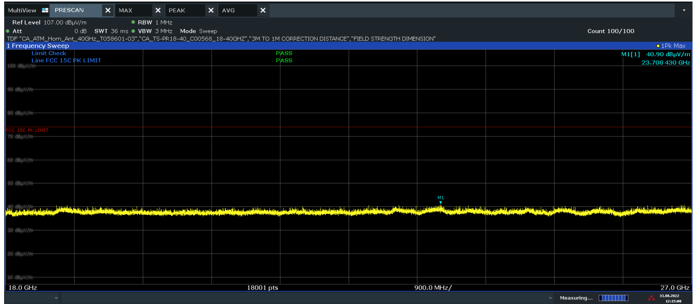
Plot 7-32. Radiated Spurious Emissions Above 18GHz H Polarity (1Mbps ePA – Ch. 19)
