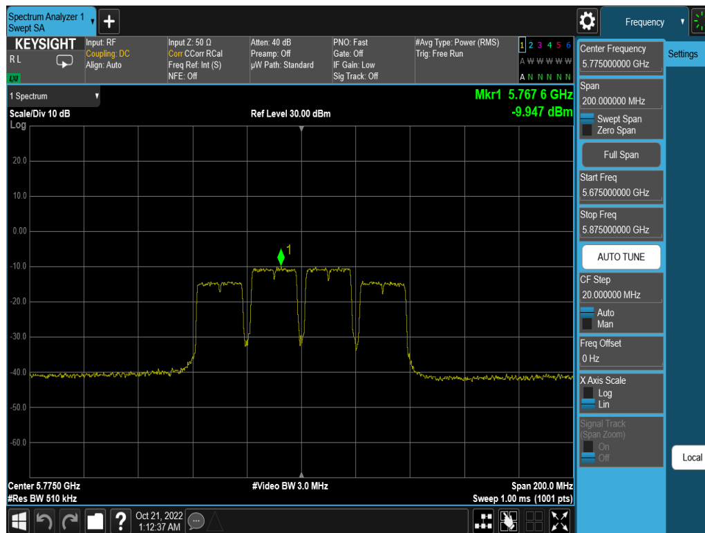
Plot 7-28. PSD (80MHz BW 802.11ac – Ch. 155, MCS0)
