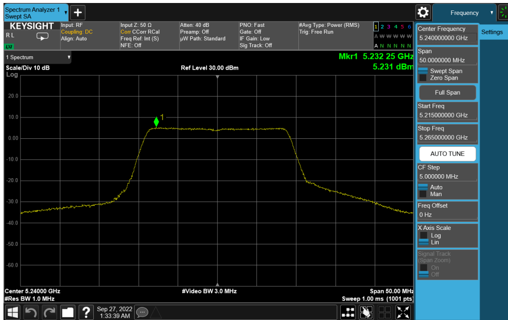
Plot 7-17. PSD (20MHz BW 802.11n – Ch. 48, MCS0)
