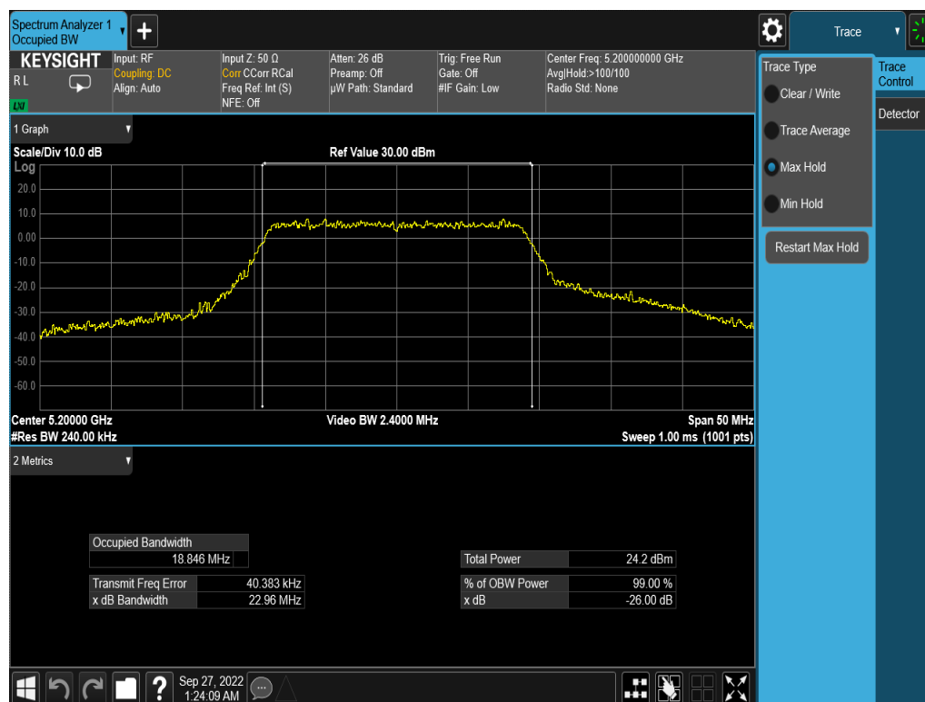
Plot 7-2. 26dB BW & 99% (20MHz BW 802.11n – Ch. 40, MCS0)
