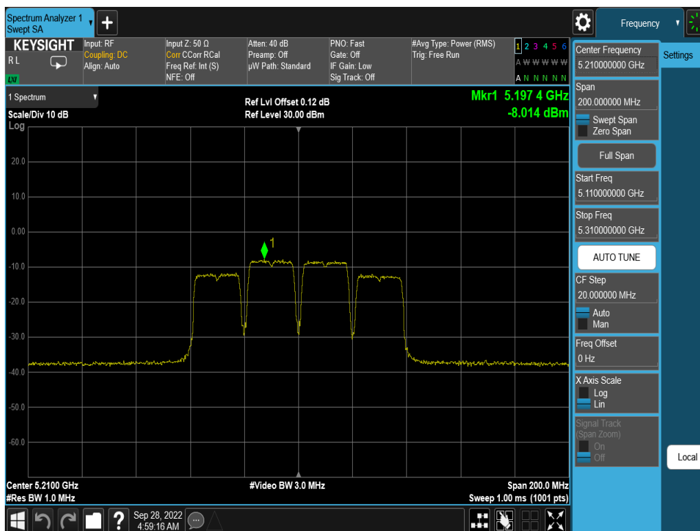
Plot 7-32. ISD PSD (80MHz BW 11ac – Ch.42, MCS0)
