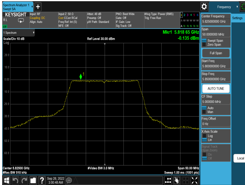
Plot 7-27. PSD (20MHz BW 802.11n – Ch. 165, MCS0)
