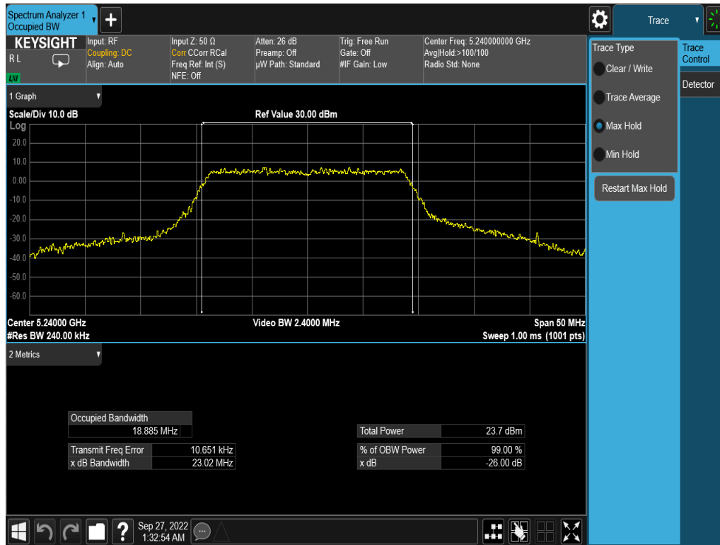
Plot 7-3. 26dB BW & 99% (20MHz BW 802.11n – Ch. 48, MCS0)
