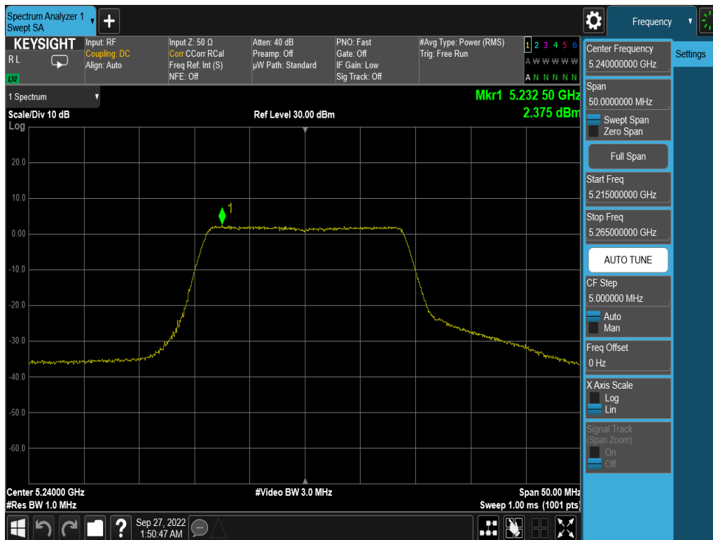
Plot 7-31. ISD PSD (20MHz BW 11n – Ch.48, MCS0)
