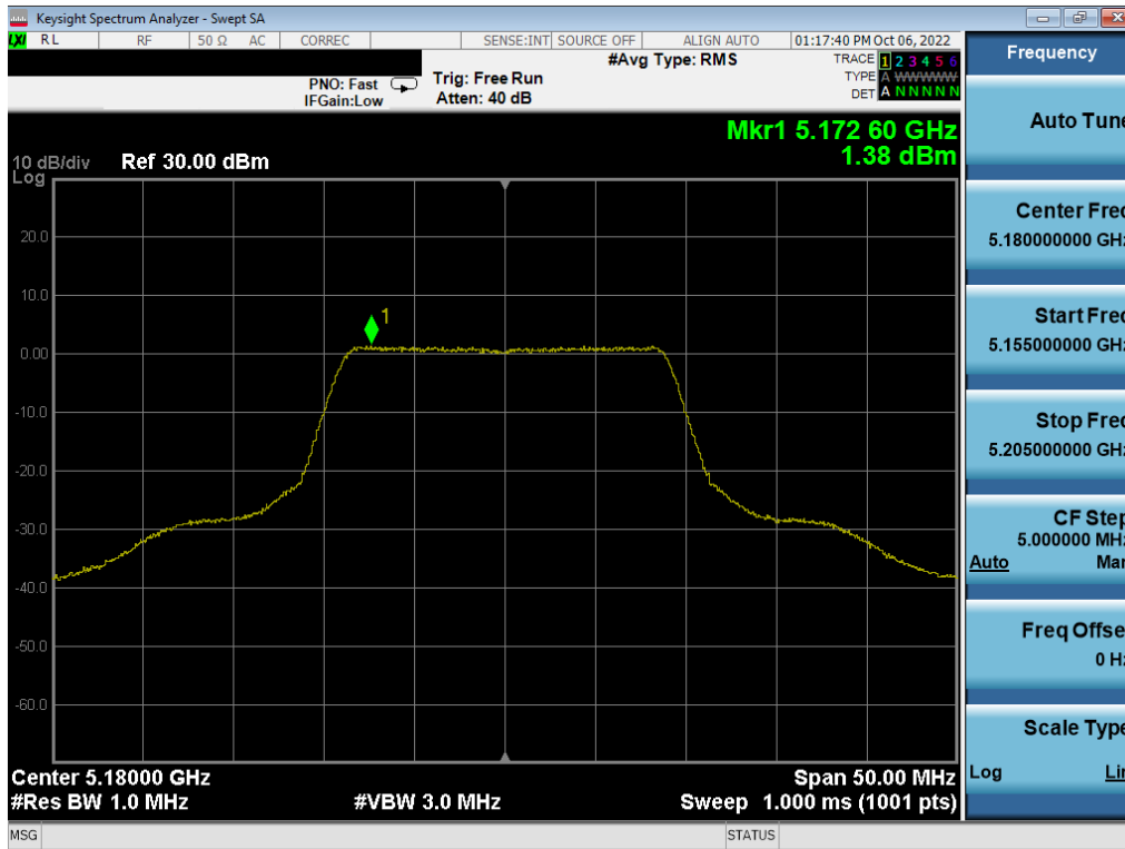
Plot 7-15. PSD (20MHz BW 802.11n – Ch. 36, MCS0)
