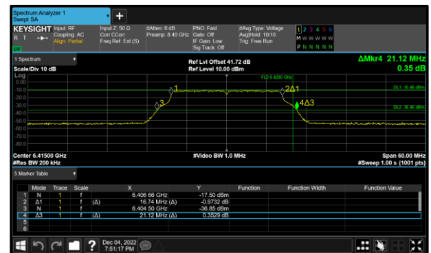
Figure 2 - 802.11a Maximum 99% OBW
