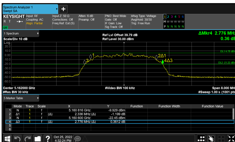
Figure 28 - Core 1 (B) 5162 MHz (CH12) 26 dB and 99% Bandwidth
