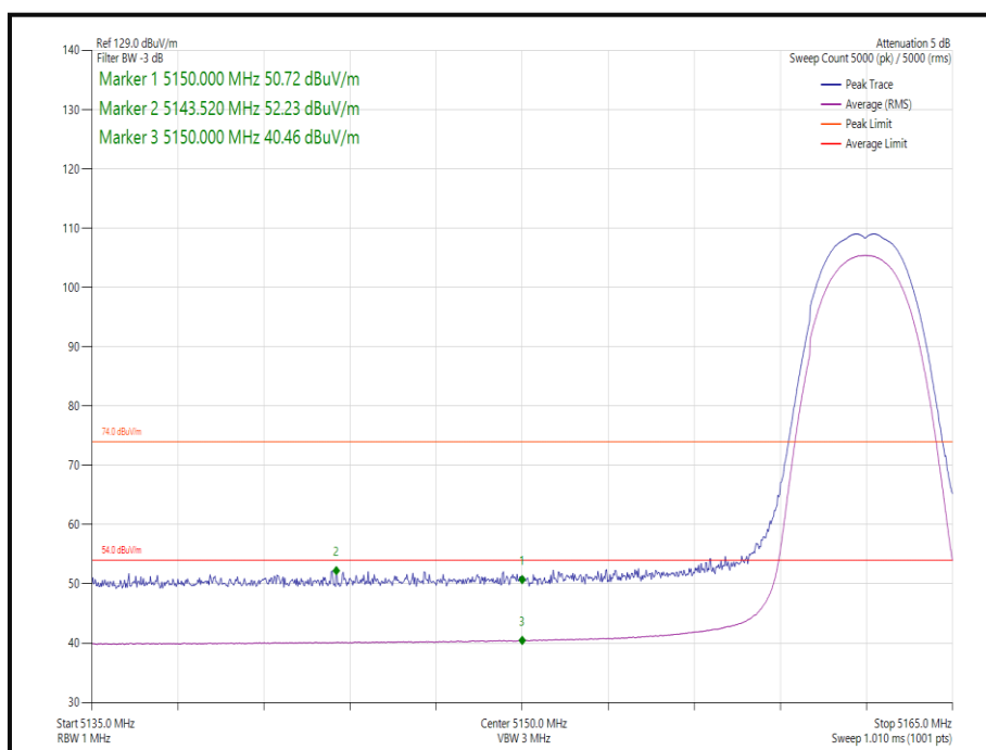
Figure 17 - Static - \pi/4 DQPSK/4-DH5 - 5162 MHz - Band Edge Frequency 5150 MHz
