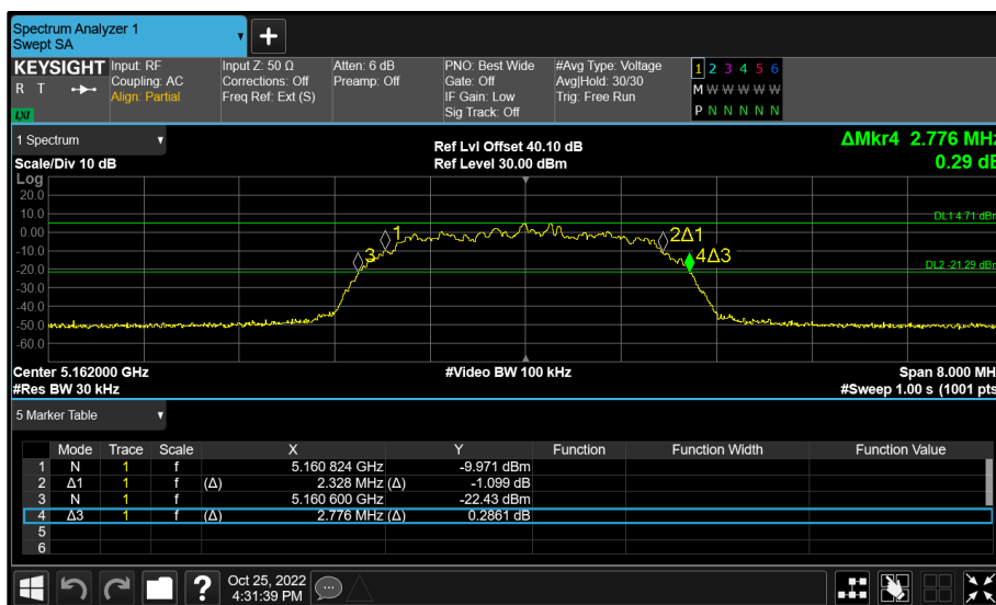
Figure 27 - Core 0 (A) 5162 MHz (CH12) 26 dB and 99% Bandwidth
