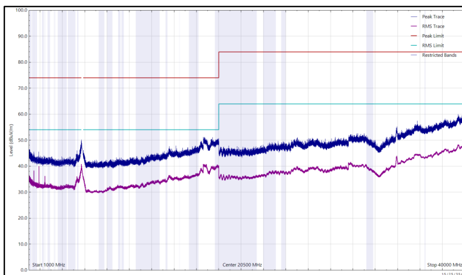
Figure 386 - U-NII-3 - 5745 MHz (CH149), VHT20, CDD, Core 0 + Core 1,1 GHz to 40 GHz, Vertical
