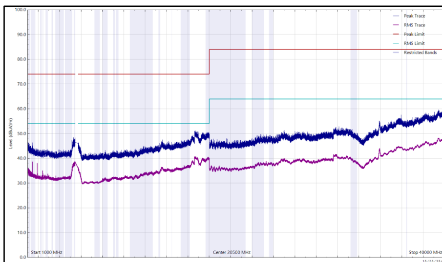
Figure 382 - U-NII-2C - 5500 MHz (CH100), VHT20, CDD, Core 0 + Core 1,1 GHz to 40 GHz, Vertical
