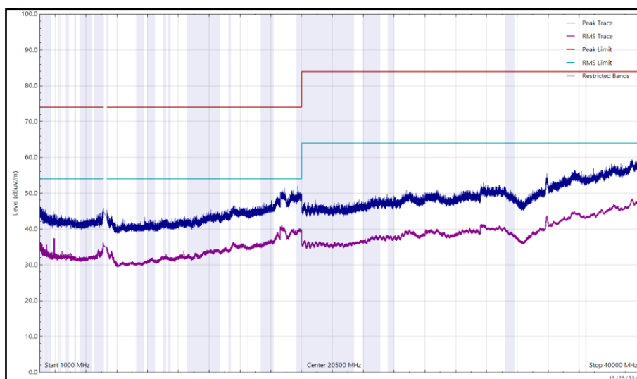
Figure 392 - U-NII-1 - 5180 MHz (CH36), HE20, RU26-0, CDD, Core 0 + Core 1,1 GHz to 40 GHz, Horizontal
