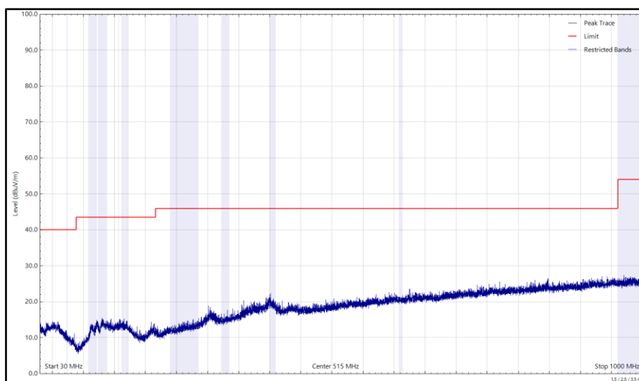
Figure 391 - U-NII-1 - 5180 MHz (CH36), HE20, RU26-0, CDD, Core 0 + Core 1,30 MHz to 1 GHz, Horizontal (Peak)
