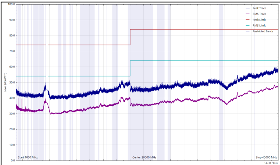
Figure 402 - U-NII-2C - 5500 MHz (CH100), HE20, RU52-37, CDD, Core 0 + Core 1, 1 GHz to 40 GHz, Vertical
