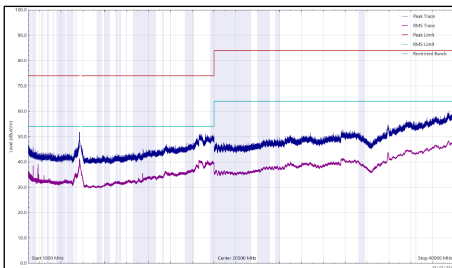
Figure 406 - U-NII-3 - 5745 MHz (CH149), HE20, RU26-0, CDD, Core 0 + Core 1,1 GHz to 40 GHz, Vertical
