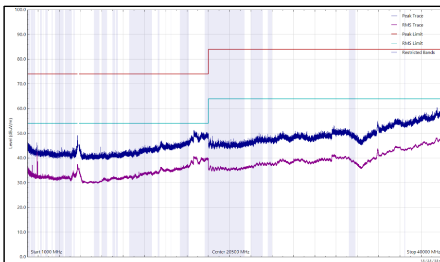
Figure 405 - U-NII-3 - 5745 MHz (CH149), HE20, RU26-0, CDD, Core 0 + Core 1,1 GHz to 40 GHz, Horizontal
