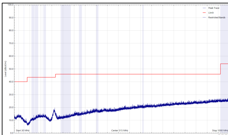
Figure 373 - U-NII-3 - 5825 MHz (CH165), 802.11a, Core 1, 30 MHz to 1 GHz, Vertical (Peak)
