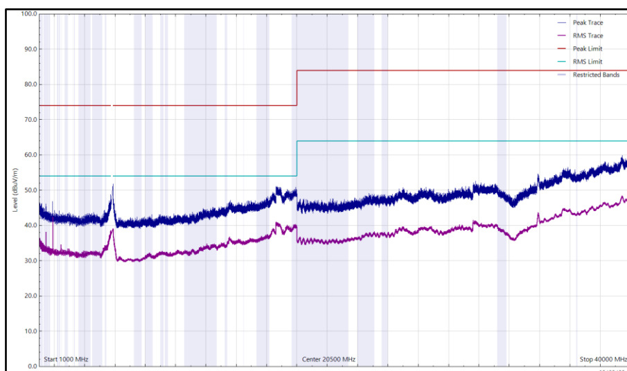
Figure 374 - U-NII-3 - 5825 MHz (CH165), 802.11a, Core 1, 1 GHz to 40 GHz, Vertical
