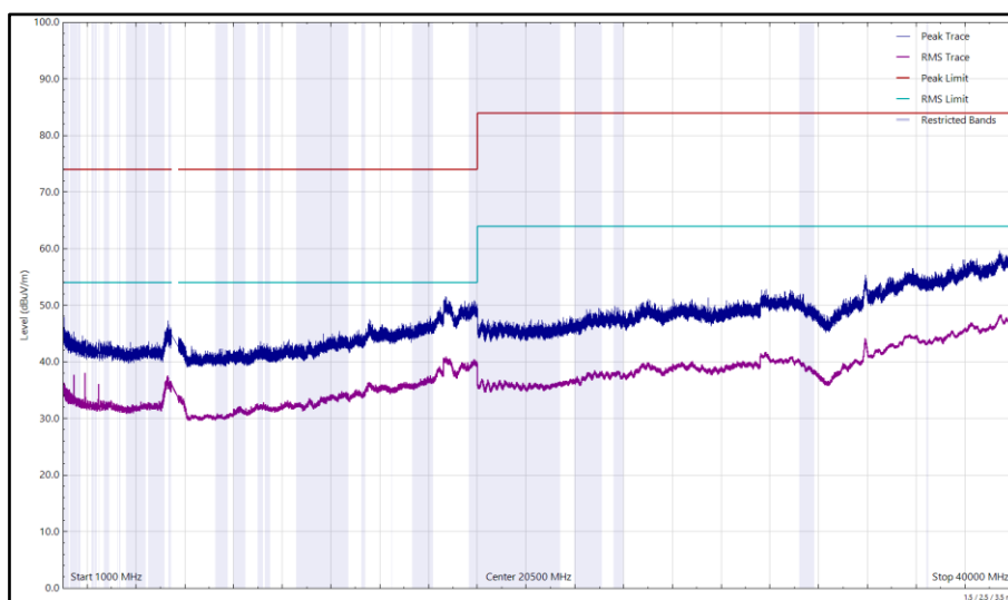
Figure 381 - U-NII-2C - 5500 MHz (CH100), VHT20, CDD, Core 0 + Core 1,1 GHz to 40 GHz, Horizontal
