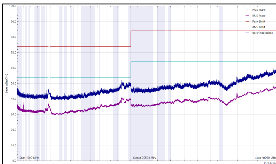
Figure 385 - U-NII-3 - 5745 MHz (CH149), VHT20, CDD, Core 0 + Core 1,1 GHz to 40 GHz, Horizontal
