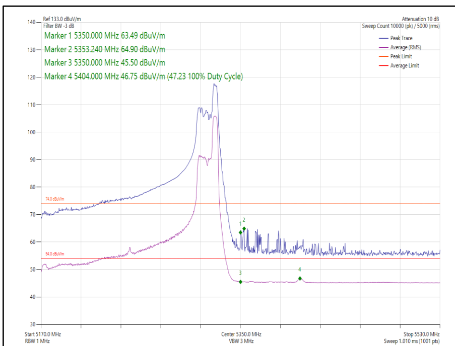
Figure 90 - 802.11ax HE160, Core 1, 52-52 - 5250 MHz, Band Edge Frequency 5350 MHz
