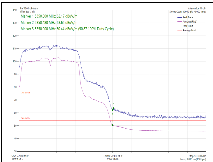
Figure 47 - 802.11n HT40 SDM, Cores 0-1 - 5310 MHz, Band Edge Frequency 5350 MHz
