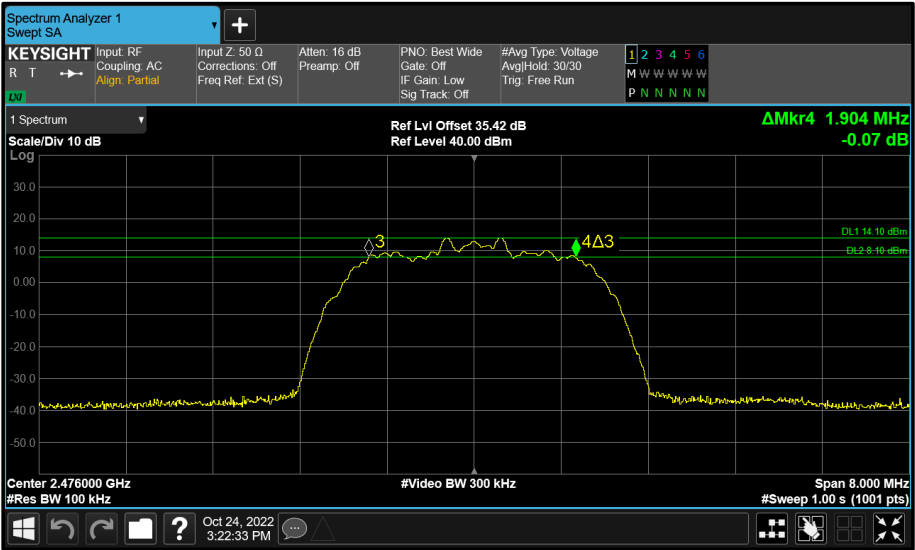
Figure 38 - Core 1 (B) 2476 MHz (CH74) 6 dB Bandwidth
