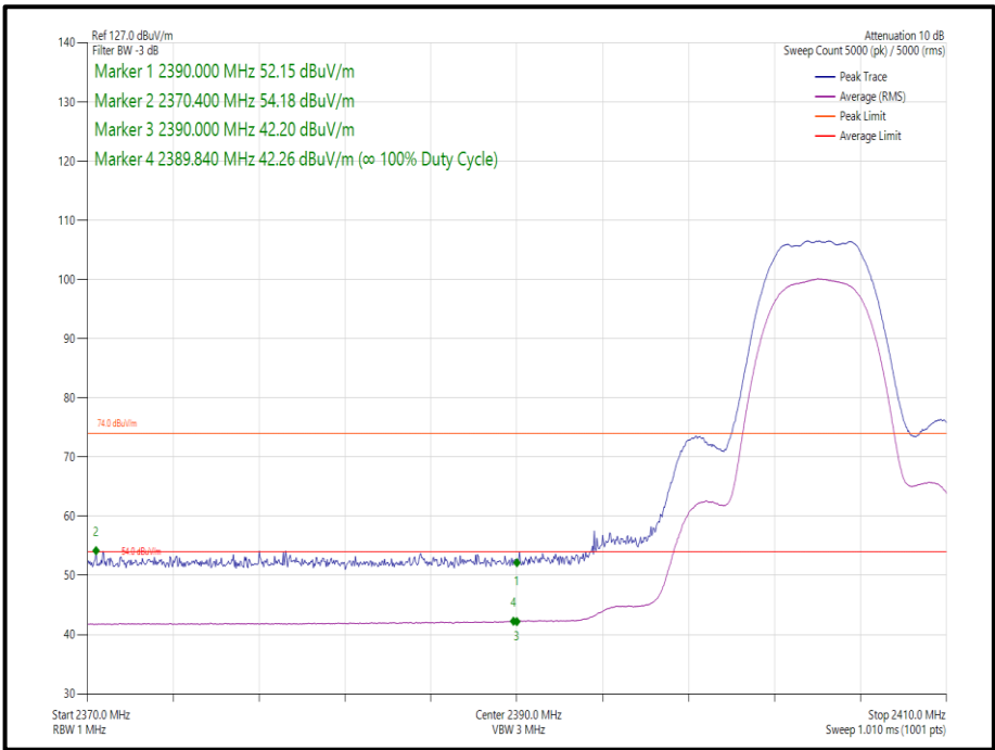
Figure 23 Core 2 - Static - GFSK/8-DH5 - 2404 MHz - Band Edge Frequency 2390.0 MHz
