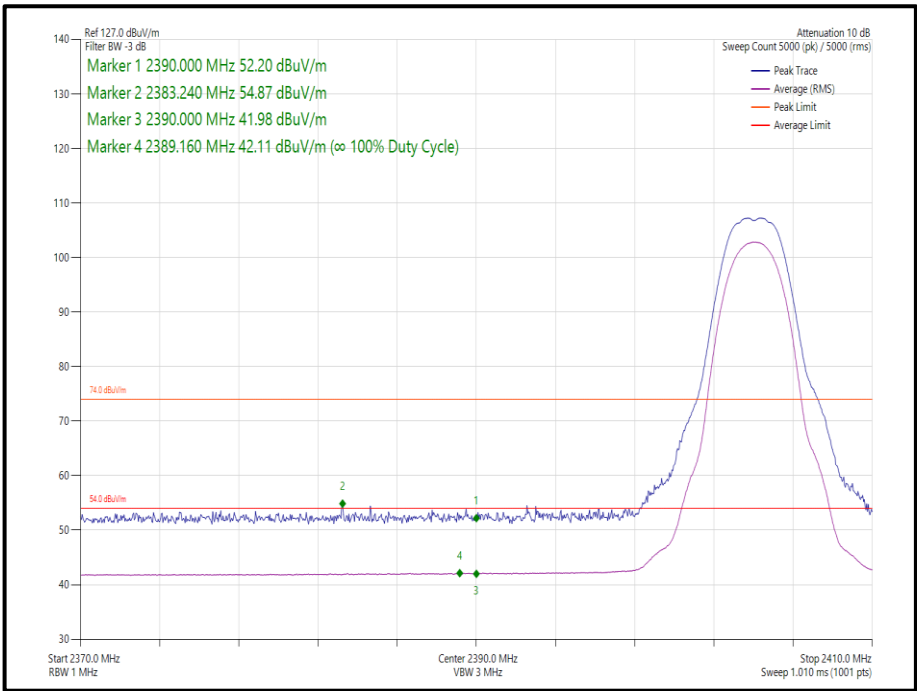
Figure 21 Core 2 - Static - GFSK/4-DH5 - 2404 MHz - Band Edge Frequency 2390.0 MHz
