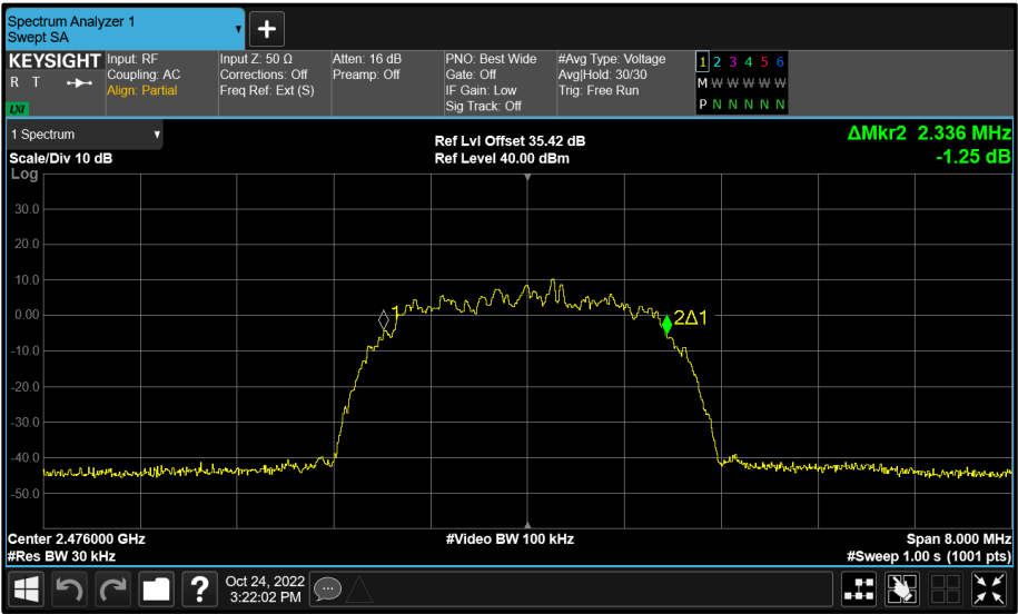
Figure 37 - Core 1 (B) 2476 MHz (CH74) 99% Bandwidth
