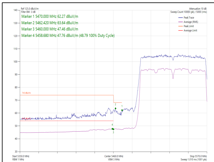
Figure 288 - 802.11ac VHT80 Core 0 - 5530 MHz, Band Edge Frequency 5470 MHz
