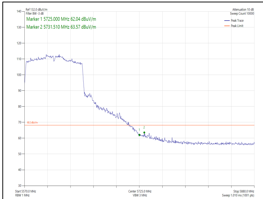
Figure 291 - 802.11ac VHT80 Core 0 - 5610 MHz, Band Edge Frequency 5725 MHz
