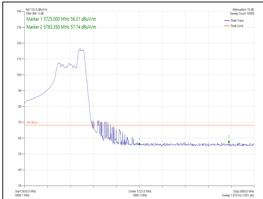
Figure 257 - 802.11ax HE40, Core 0, 52-44 - 5670 MHz, Band Edge Frequency 5725 MHz
