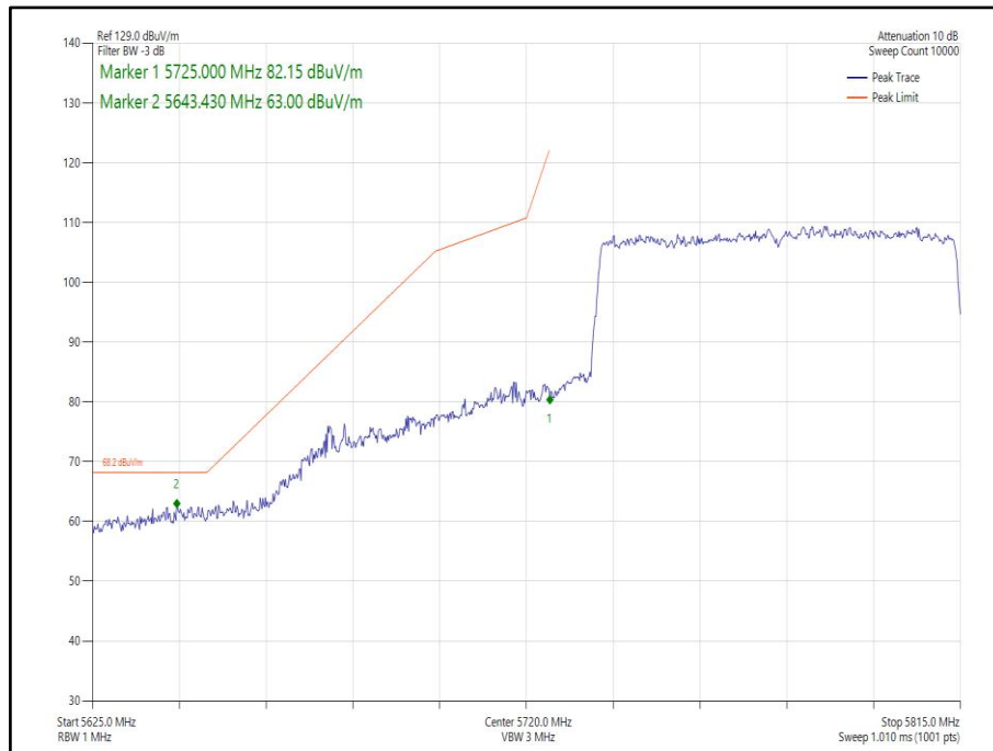
Figure 295 - 802.11ax HE80 Core 0 SU - 5775 MHz, Band Edge Frequency 5725 MHz
