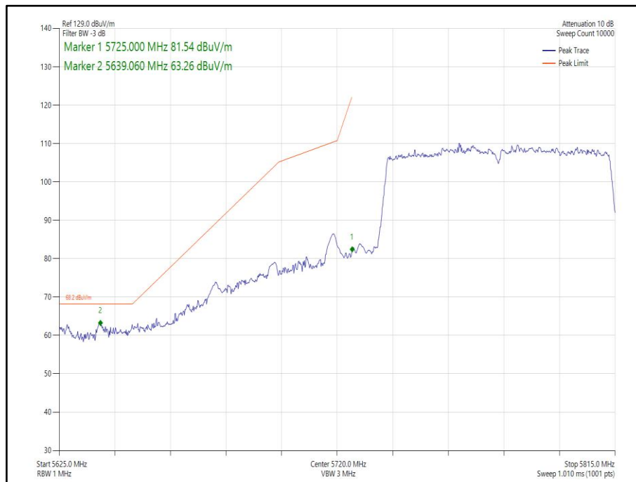
Figure 294 - 802.11ac VHT80 Core 0 - 5775 MHz, Band Edge Frequency 5725 MHz
