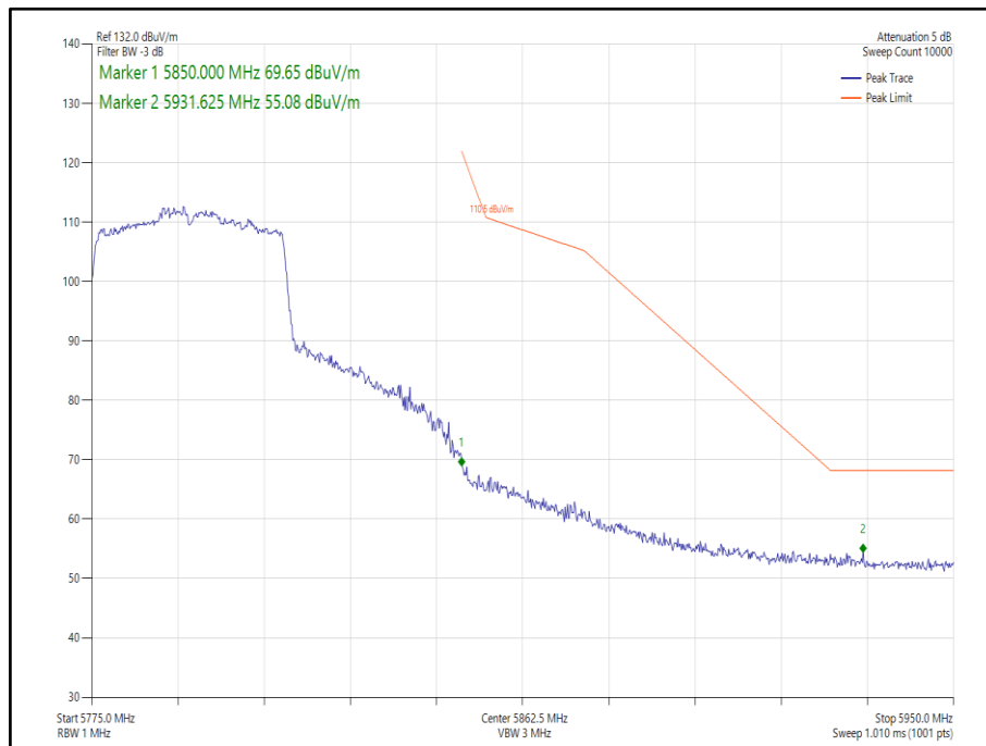
Figure 262 - 802.11ax HE40, Core 0, SU - 5795 MHz, Band Edge Frequency 5850 MHz
