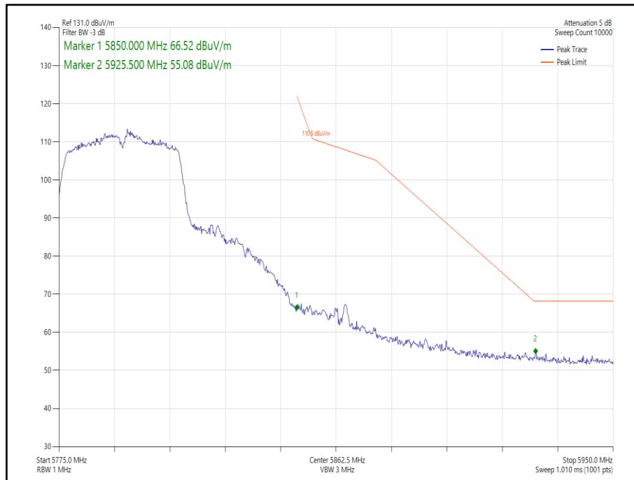
Figure 261 - 802.11n HT40, Core 0, - 5795 MHz, Band Edge Frequency 5850 MHz
