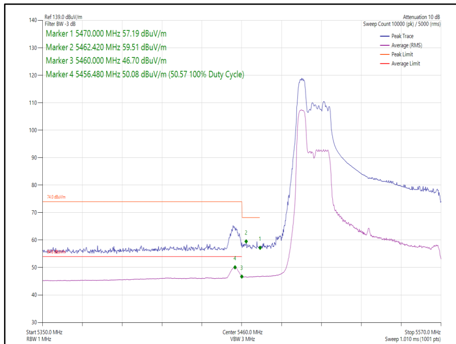
Figure 290 - 802.11ax HE80 Core 0 52-37- 5530 MHz, Band Edge Frequency 5470 MHz
