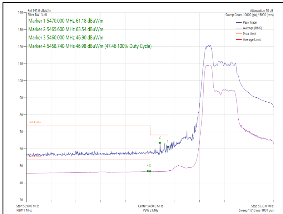
Figure 254 - 802.11ax HE40, Core 0, 52-37 - 5510 MHz, Band Edge Frequency 5470 MHz
