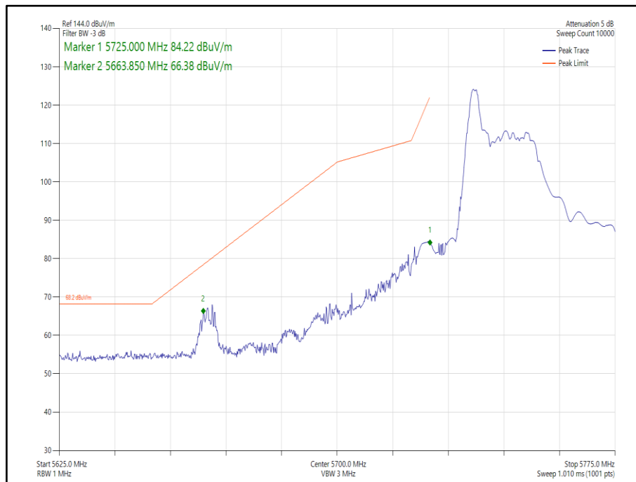
Figure 260 - 802.11ax HE40, Core 0, 26-0 - 5755 MHz, Band Edge Frequency 5725 MHz
