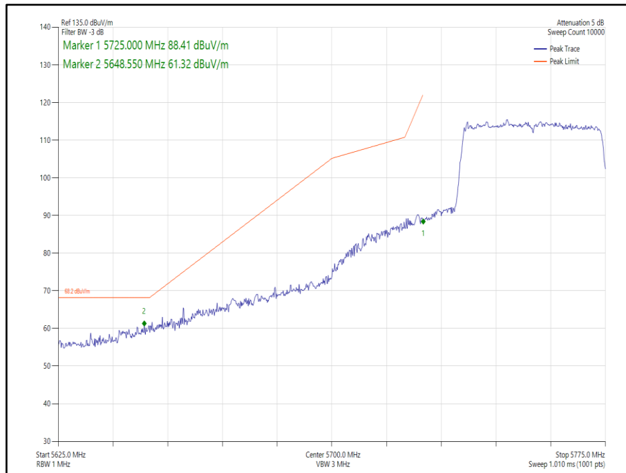
Figure 259 - 802.11ax HE40, Core 0, SU - 5755 MHz, Band Edge Frequency 5725 MHz
