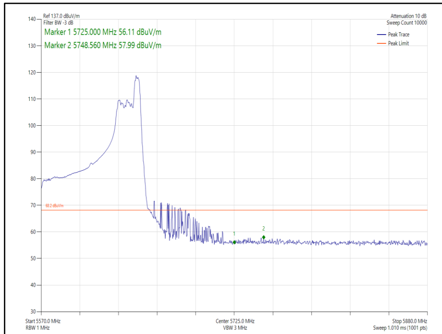
Figure 293 - - 802.11ax HE80 Core 0 52-52 - 5610 MHz, Band Edge Frequency 5725 MHz
