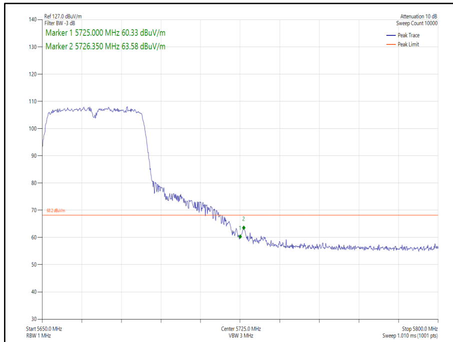
Figure 255 - 802.11n HT40, Core 0, - 5670 MHz, Band Edge Frequency 5725 MHz
