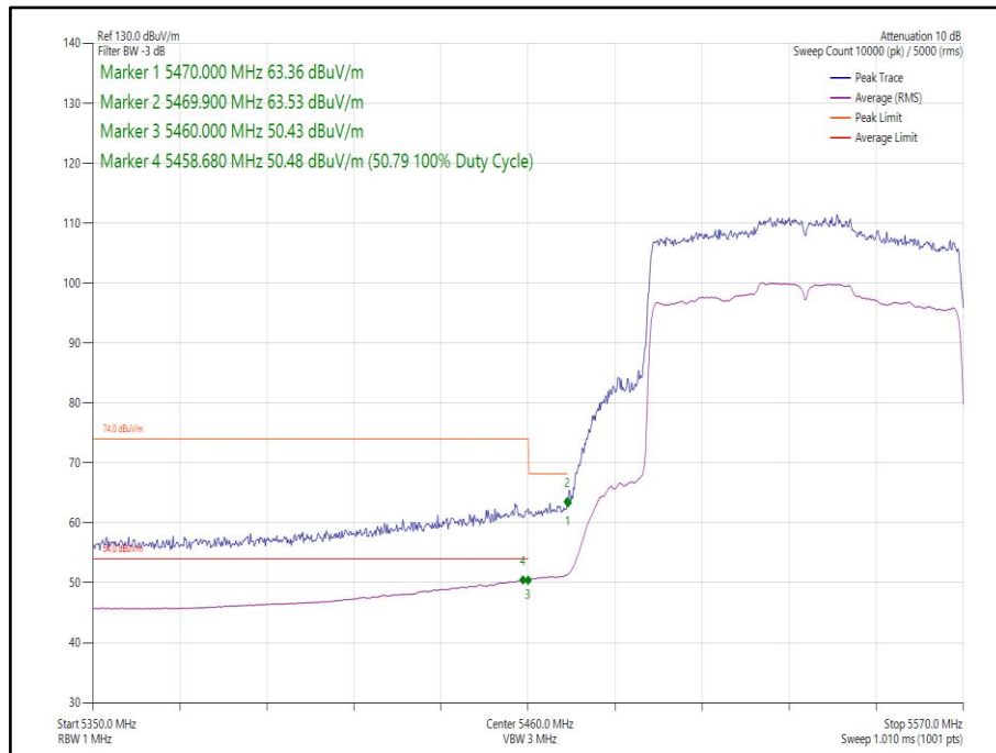
Figure 289 - 802.11ax HE80 Core 0 SU - 5530 MHz, Band Edge Frequency 5470 MHz
