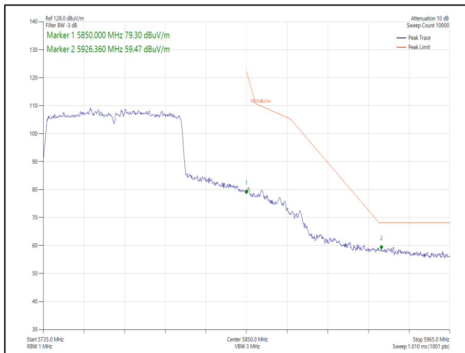
Figure 297 - 802.11ac VHT80 Core 0 - 5775 MHz, Band Edge Frequency 5850 MHz
