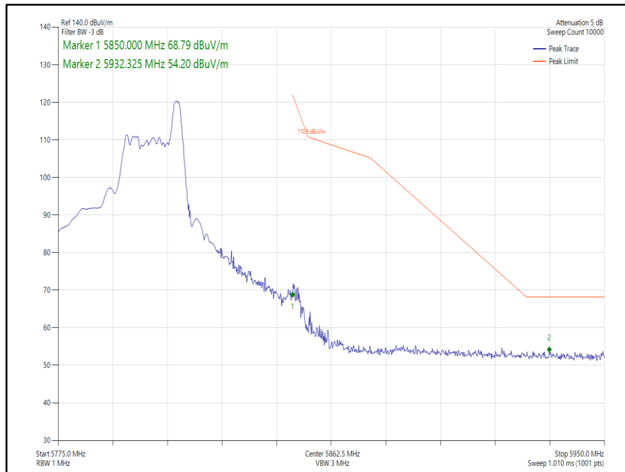
Figure 263 - 802.11ax HE40, Core 0, 26-17 - 5795 MHz, Band Edge Frequency 5850 MHz
