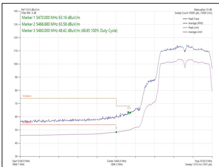
Figure 252 - 802.11n HT40, Core 0 - 5510 MHz, Band Edge Frequency 5470 MHz
