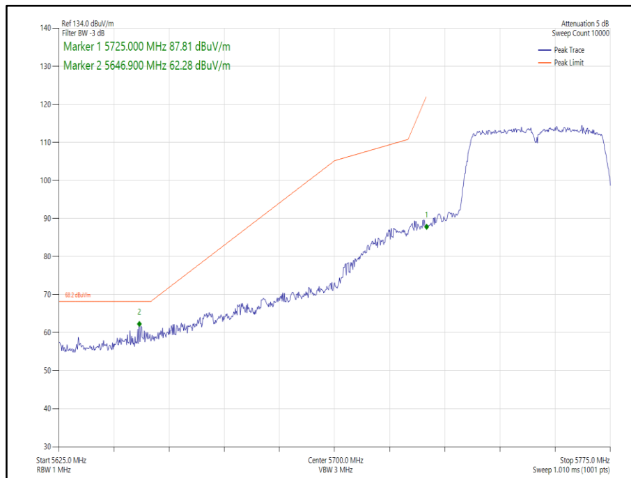
Figure 258 - 802.11n HT40, Core 0, - 5755 MHz, Band Edge Frequency 5725 MHz
