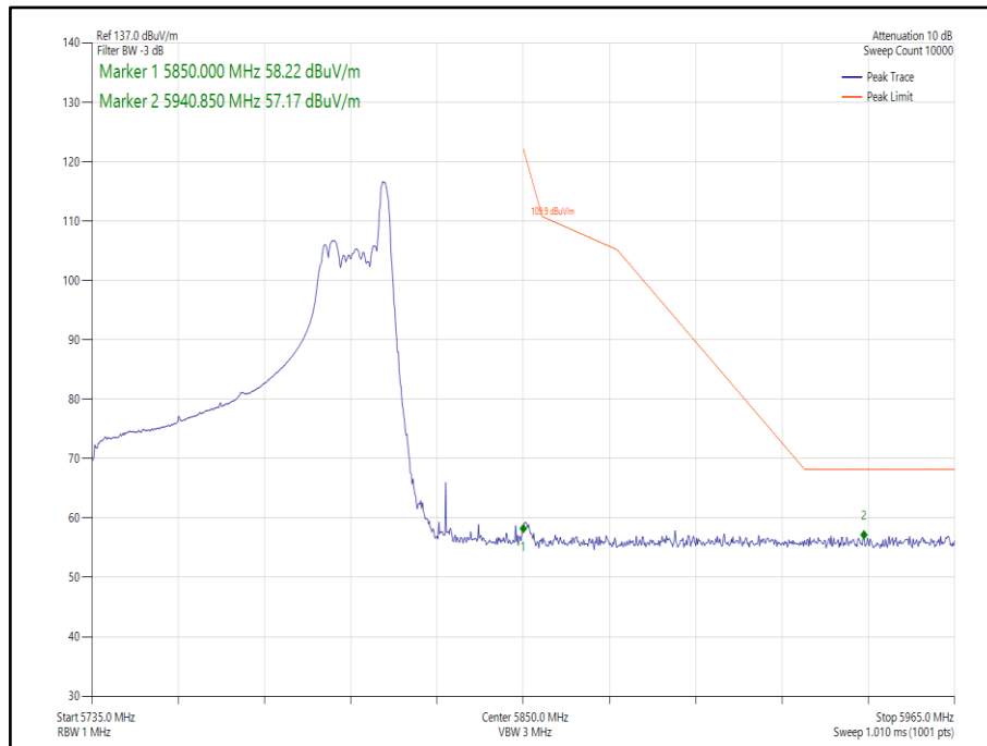
Figure 299 - 802.11ax HE80 Core 0 26-36 - 5775 MHz, Band Edge Frequency 5850 MHz
