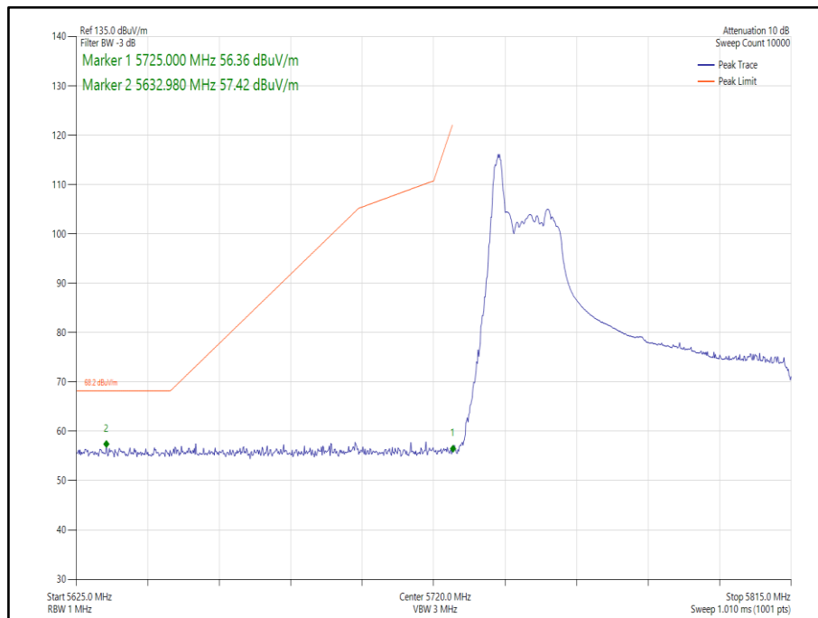
Figure 296 - 802.11ax HE80 Core 0 26-0 - 5775 MHz, Band Edge Frequency 5725 MHz
