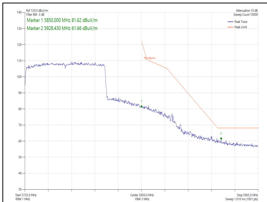
Figure 298 - 802.11ax HE80 Core 0 SU - 5775 MHz, Band Edge Frequency 5850 MHz
