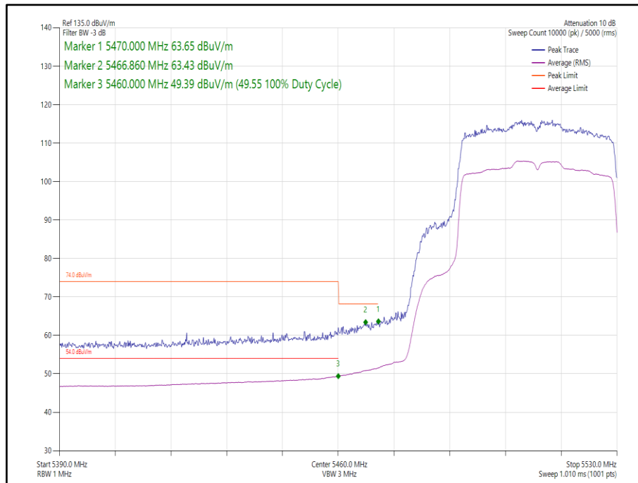
Figure 253 - 802.11ax HE40, Core 0, SU - 5510 MHz, Band Edge Frequency 5470 MHz
