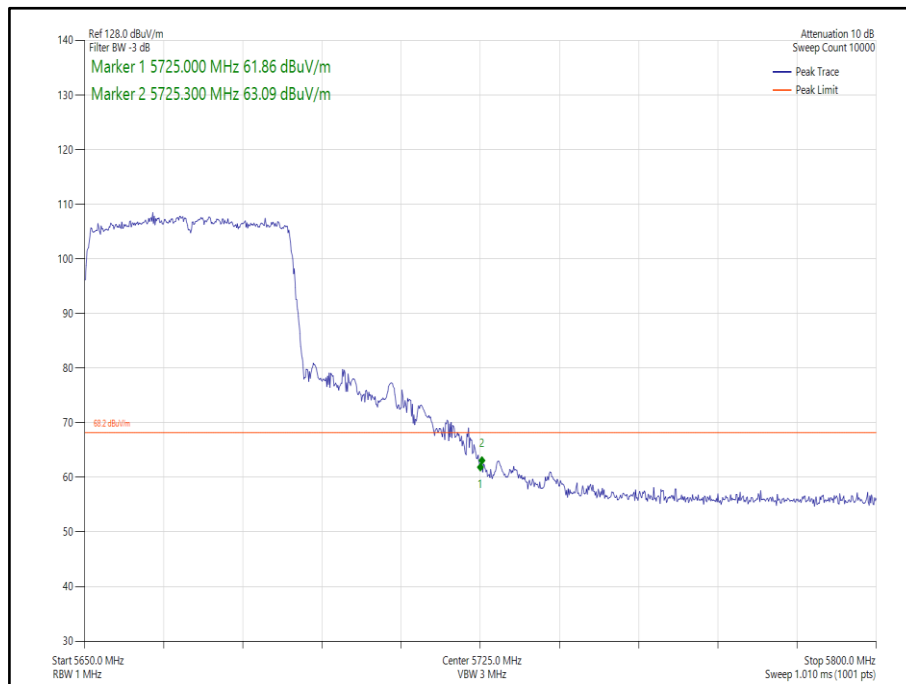
Figure 256 - 802.11ax HE40, Core 0, SU - 5670 MHz, Band Edge Frequency 5725 MHz
