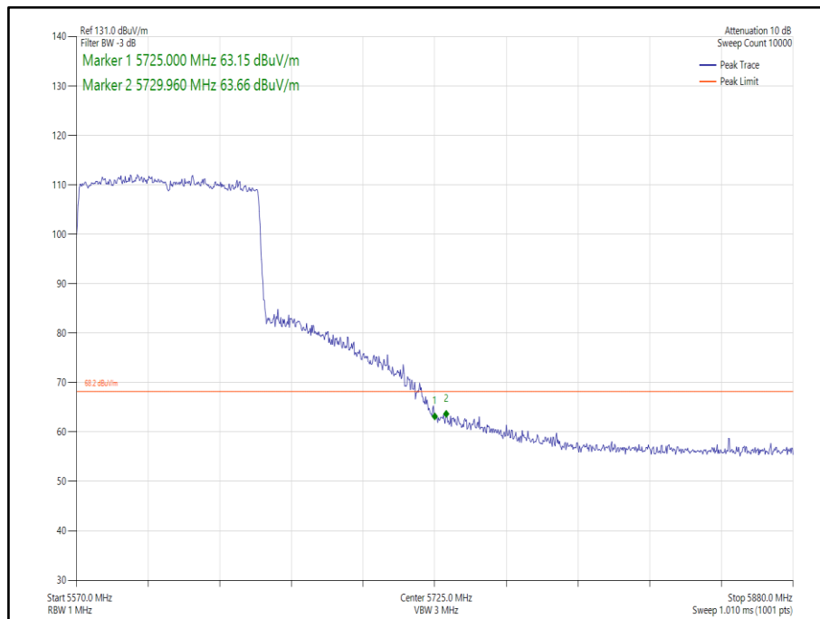
Figure 292 - - 802.11ax HE80 Core 0 SU - 5610 MHz, Band Edge Frequency 5725 MHz
