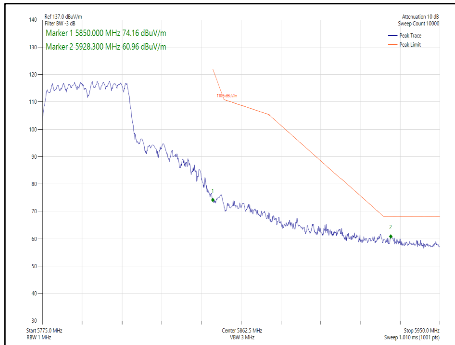
Figure 282 - 802.11n HT40 CDD, Cores 0-1 - 795 MHz, Band Edge Frequency 5850 MHz
