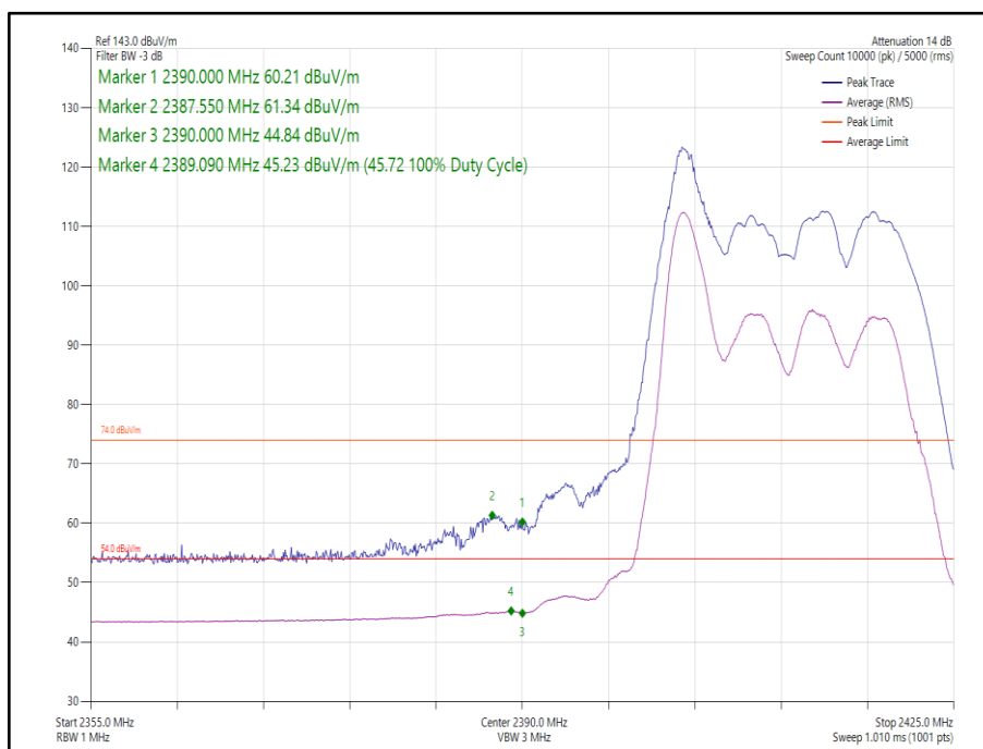
Figure 25 - 802.11ax HE20, Core 0-1, 26-0 - 2412 MHz, Band Edge Frequency 2390 MHz
