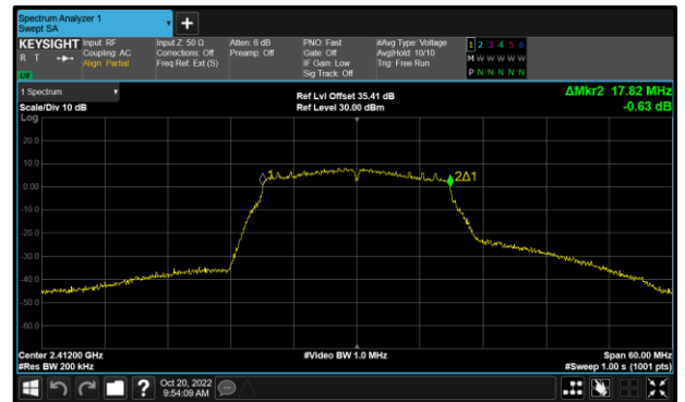
Figure 44 - 802.11n HT20 Maximum 99% OBW
