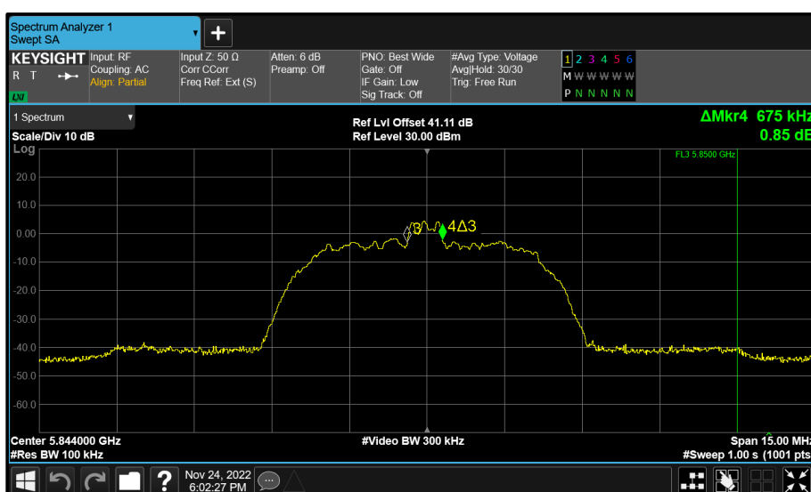
Figure 200 - Core 1 (B) 5844 MHz (CH119) 6 dB Bandwidth
