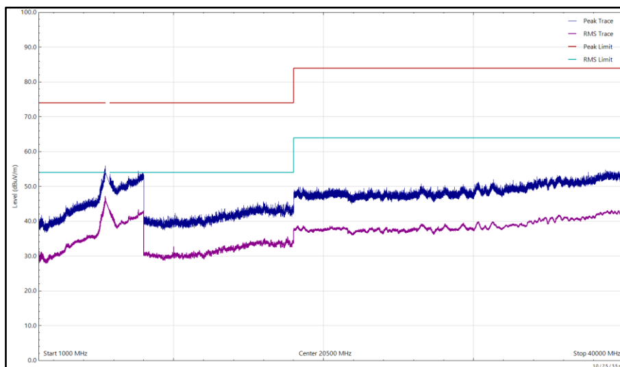
Figure 368 - U-NII-2C - 5500 MHz (CH100), 802.11a, Core 0, 1 GHz to 40 GHz, Vertical
