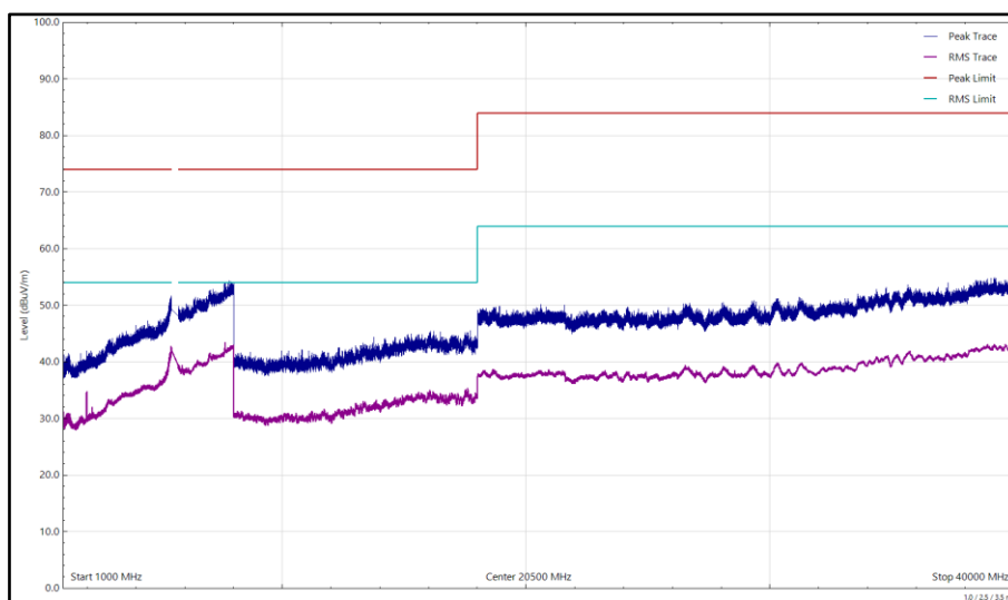
Figure 367 - U-NII-2C - 5500 MHz (CH100), 802.11a, Core 0, 1 GHz to 40 GHz, Horizontal
