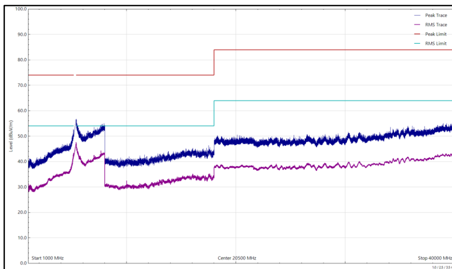
Figure 360 - U-NII-2A - 5320 MHz (CH64), 802.11a, Core 0, 1 GHz to 40 GHz, Vertical
