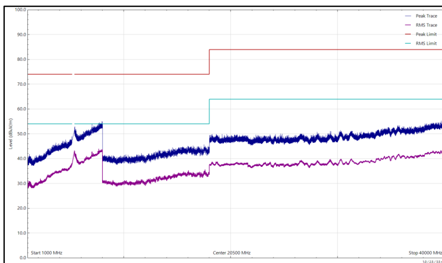
Figure 359 - U-NII-2A - 5320 MHz (CH64), 802.11a, Core 0, 1 GHz to 40 GHz, Horizontal
