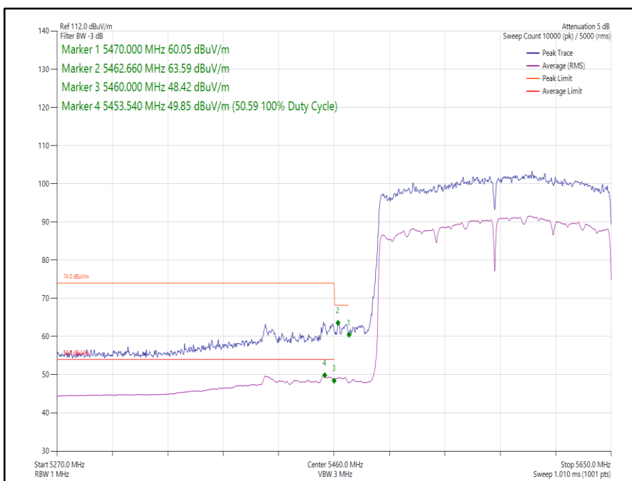
Figure 325 - 802.11ax HE160 Core 1 SU - 5570 MHz Band Edge Frequency 5470 MHz
