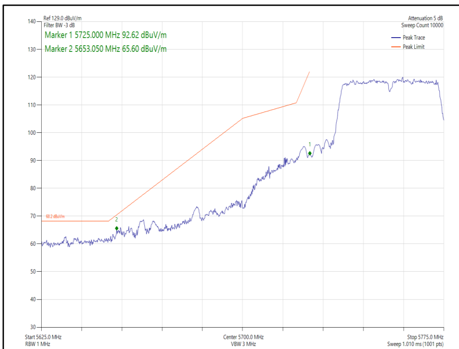
Figure 277 - 802.11n HT40 SDM, Cores 0-1 - 5755 MHz Band Edge Frequency 5725 MHz
