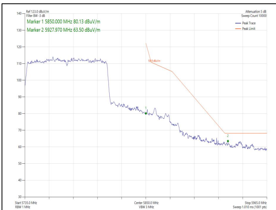
Figure 297 - 802.11ac VHT80 Core 1 - 5775 MHz Band Edge Frequency 5850 MHz
