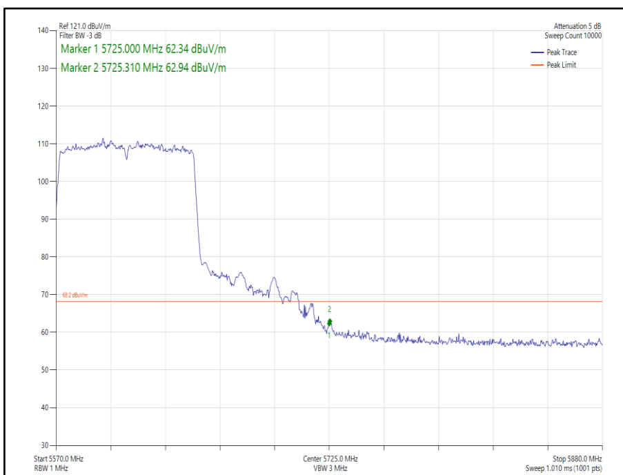
Figure 291 - 802.11ac VHT80 Core 1 - 5610 MHz Band Edge Frequency 5725 MHz
