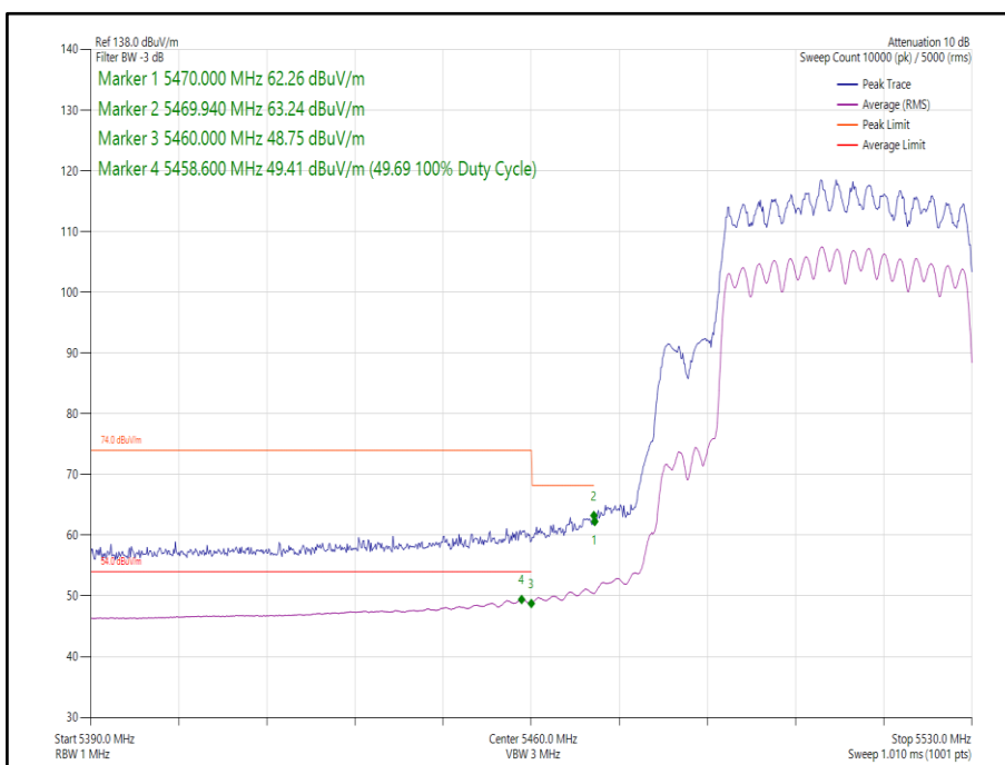
Figure 266 - 802.11ax HE40 CDD, Cores 0-1, SU - 5510 MHz Band Edge Frequency 5470 MHz
