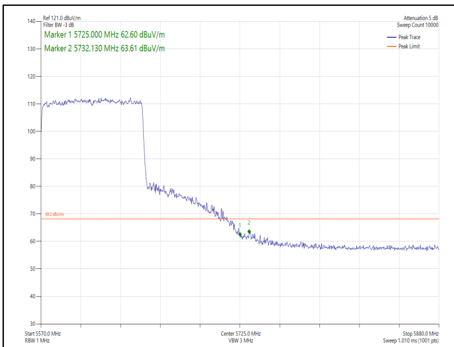
Figure 292 - - 802.11ax HE80 Core 1 SU - 5610 MHz Band Edge Frequency 5725 MHz
