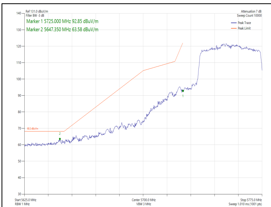
Figure 280 - 802.11ax HE40 SDM, Cores 0-1, SU - 5755 MHz Band Edge Frequency 5725 MHz
