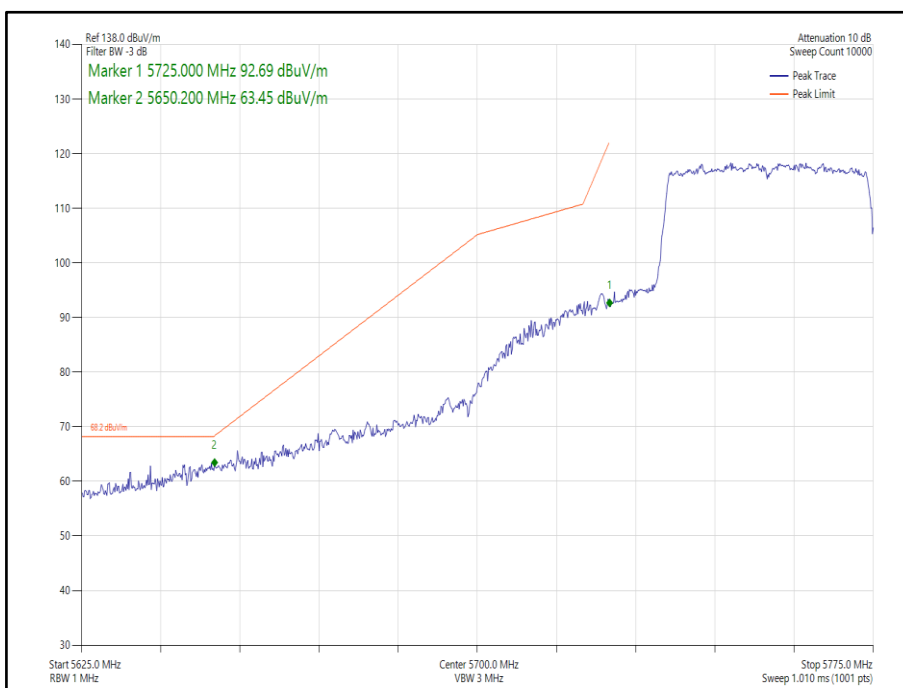
Figure 259 - 802.11ax HE40, Core 1, SU - 5755 MHz Band Edge Frequency 5725 MHz
