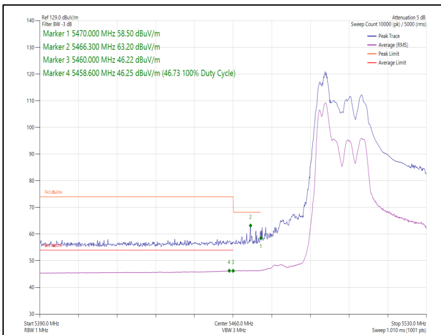
Figure 269 - 802.11ax HE40 SDM, Cores 0-1, 52-37 - 5510 MHz Band Edge Frequency 5470 MHz
