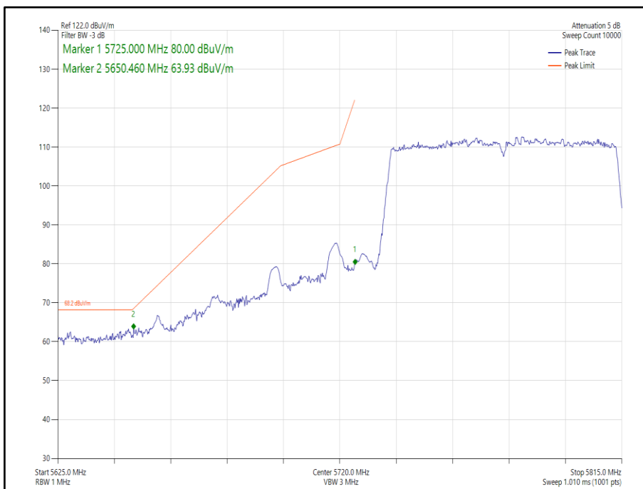
Figure 294 - 802.11ac VHT80 Core 1 - 5775 MHz Band Edge Frequency 5725 MHz
