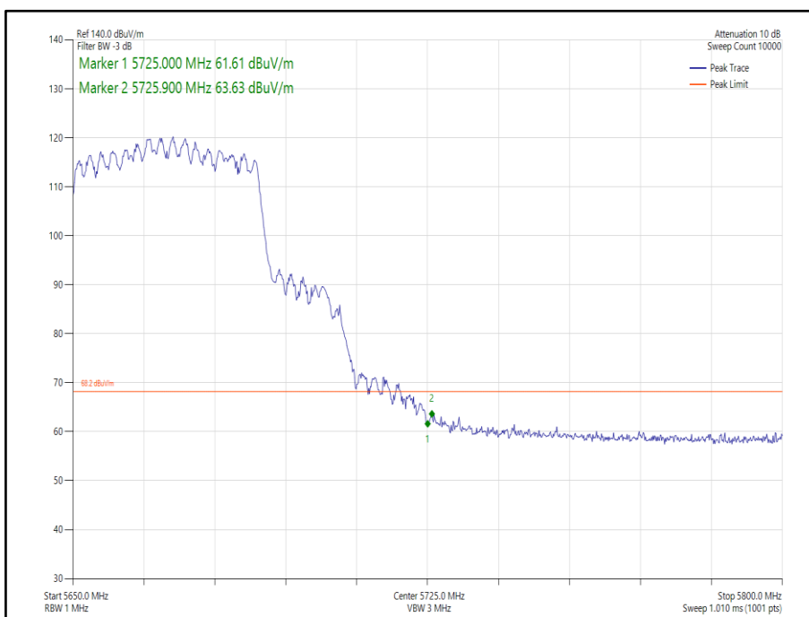
Figure 272 - 802.11ax HE40 CDD, Cores 0-1, SU - 5670 MHz Band Edge Frequency 5725 MHz
