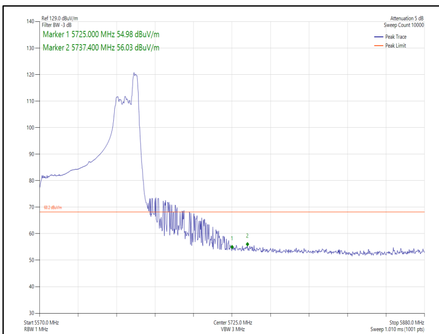
Figure 293 - - 802.11ax HE80 Core 1 52-52 - 5610 MHz Band Edge Frequency 5725 MHz
