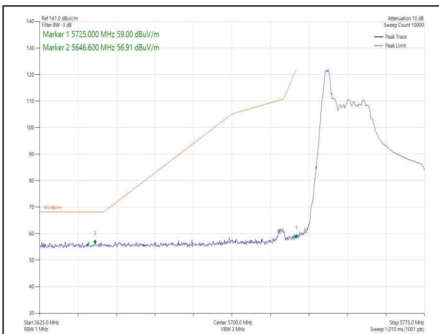
Figure 260 - 802.11ax HE40, Core 1, 26-0 - 5755 MHz Band Edge Frequency 5725 MHz
