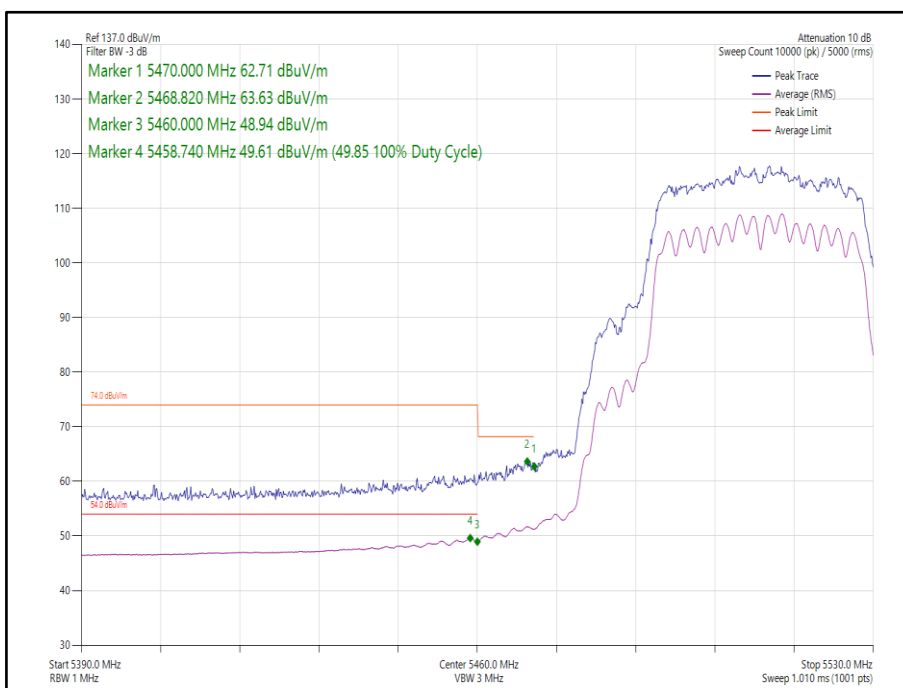
Figure 264 - 802.11n HT40 CDD, Cores 0-1 - 5510 MHz Band Edge Frequency 5470 MHz
