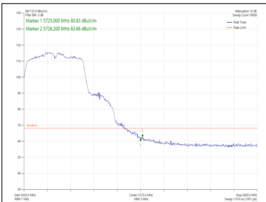
Figure 255 - 802.11n HT40, Core 1 - 5670 MHz Band Edge Frequency 5725 MHz
