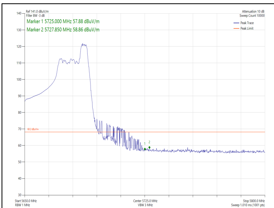
Figure 257 - 802.11ax HE40, Core 1, 52-44 - 5670 MHz Band Edge Frequency 5725 MHz
