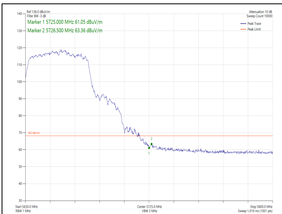
Figure 270 - 802.11n HT40 CDD, Cores 0-1 - 5670 MHz Band Edge Frequency 5725 MHz
