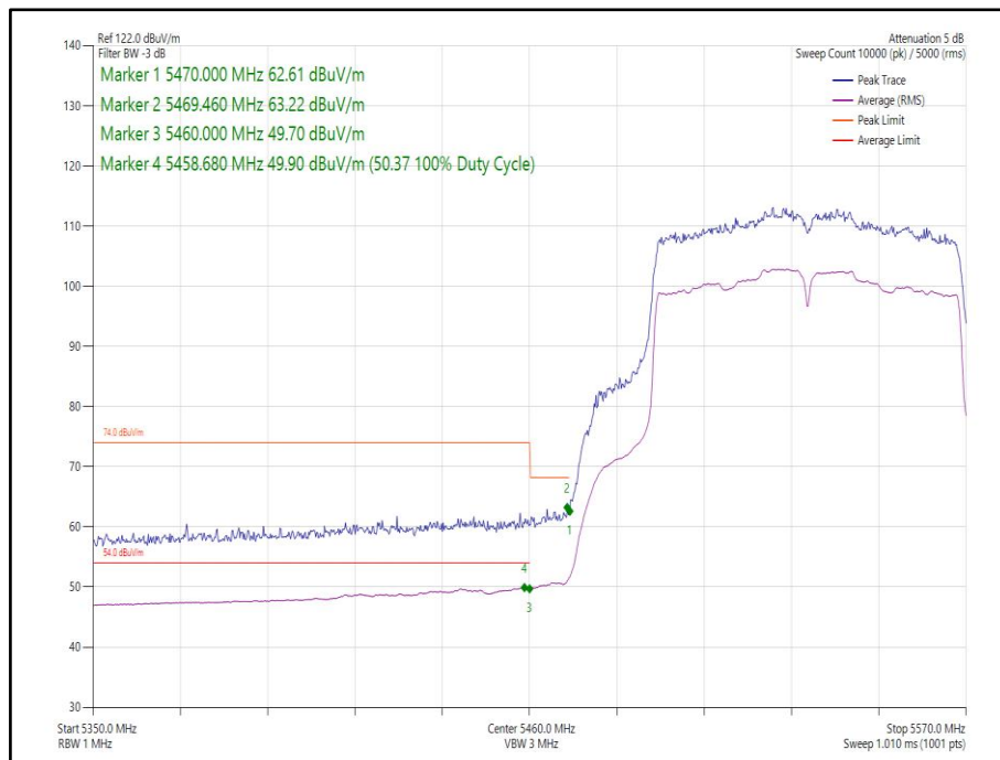
Figure 288 - 802.11ac VHT80 Core 1 - 5530 MHz Band Edge Frequency 5470 MHz
