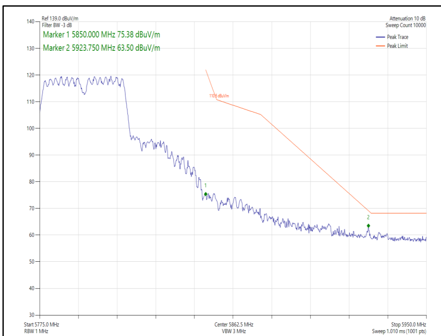
Figure 282 - 802.11n HT40 CDD, Cores 0-1 - 5795 MHz Band Edge Frequency 5850 MHz
