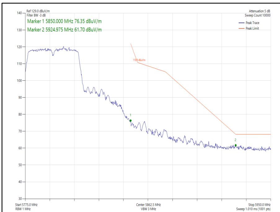
Figure 283 - 802.11n HT40 SDM, Cores 0-1 - 5795 MHz Band Edge Frequency 5850 MHz
