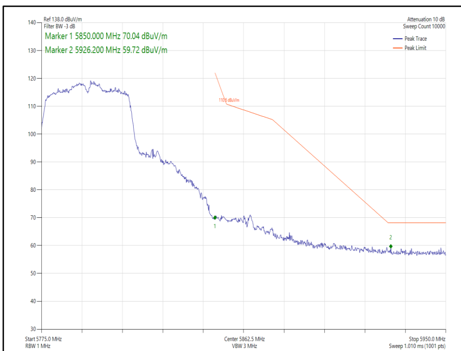
Figure 261 - 802.11n HT40, Core 1 - 5795 MHz Band Edge Frequency 5850 MHz
