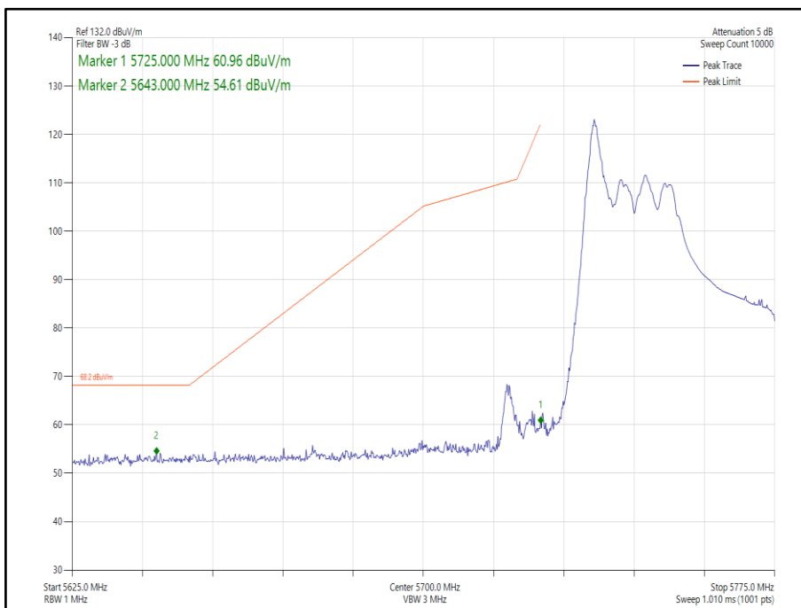
Figure 281 - 802.11ax HE40 SDM, Cores 0-1, 26-0 - 5755 MHz Band Edge Frequency 5725 MHz
