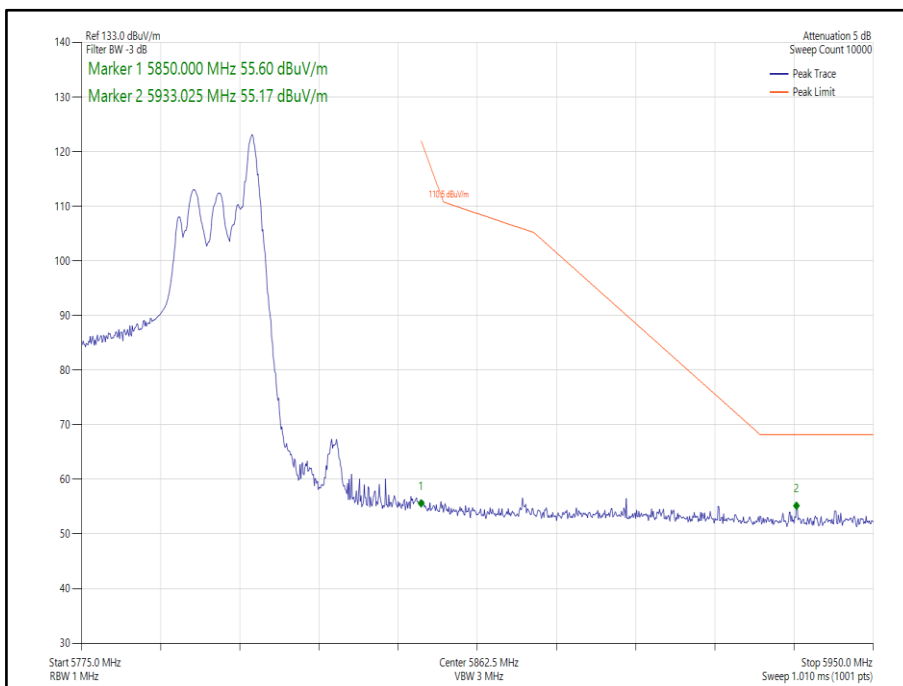
Figure 287 - 802.11ax HE40 SDM, Cores 0-1, 26-17 - 5795 MHz Band Edge Frequency 5850 MHz
