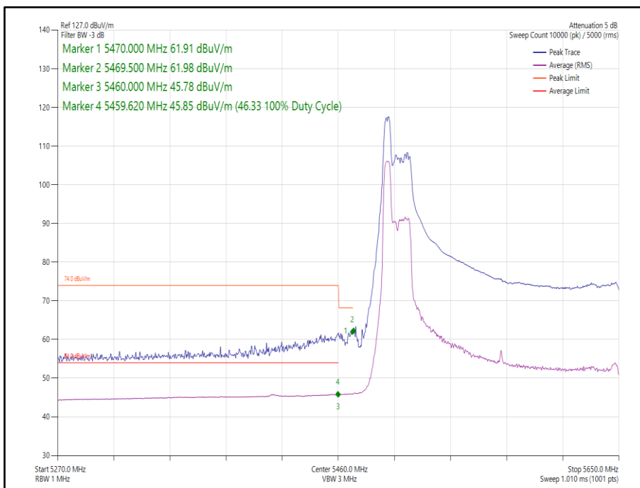
Figure 326 - 802.11ax HE160 Core 1 52-37- 5570 MHz Band Edge Frequency 5470 MHz
