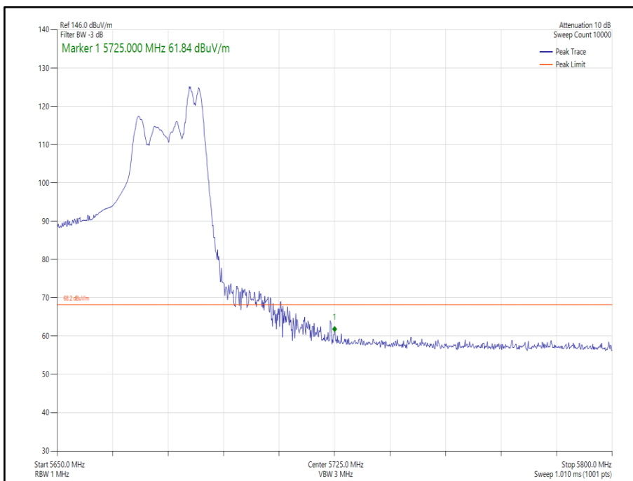
Figure 273 - 802.11ax HE40 CDD, Cores 0-1, 52-44 - 5670 MHz Band Edge Frequency 5725 MHz
