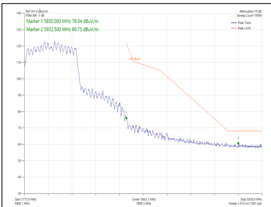
Figure 284 - 802.11ax HE40 CDD, Cores 0-1, SU - 5795 MHz Band Edge Frequency 5850 MHz
