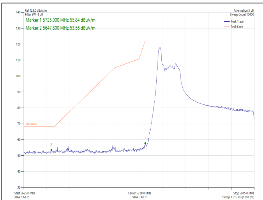
Figure 296 - 802.11ax HE80 Core 1 26-0 - 5775 MHz Band Edge Frequency 5725 MHz
