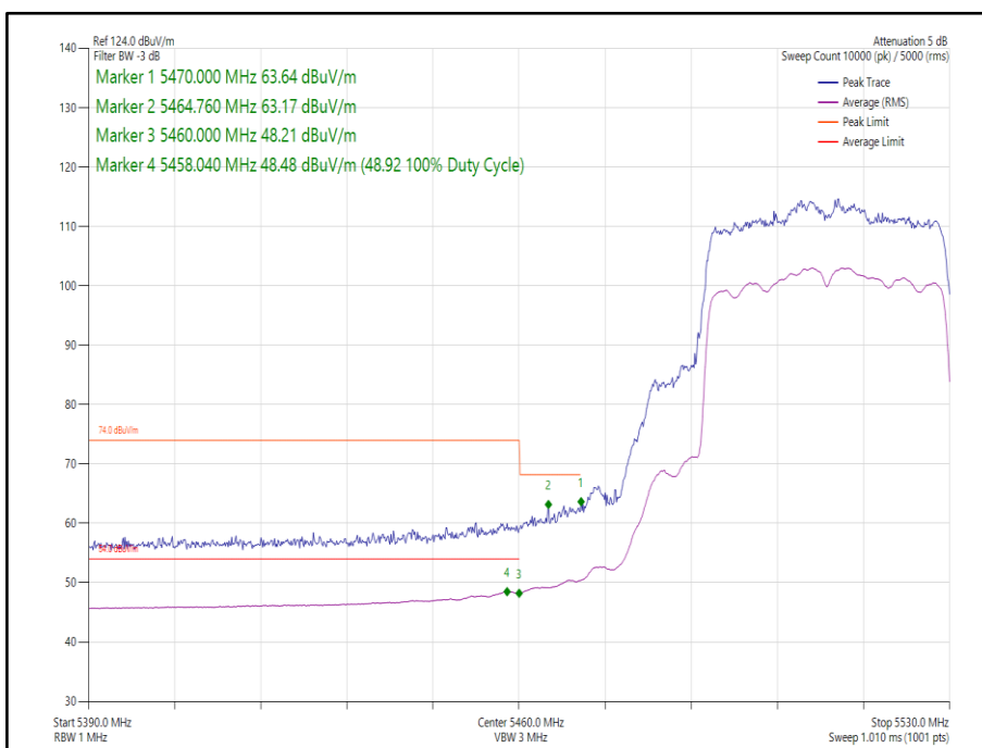
Figure 268 - 802.11ax HE40 SDM, Cores 0-1, SU - 5510 MHz Band Edge Frequency 5470 MHz
