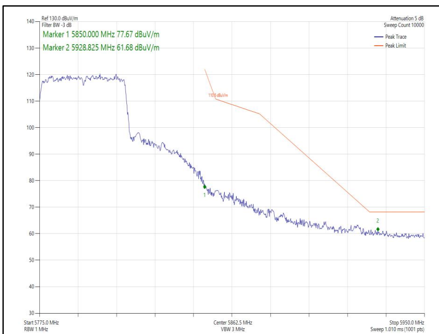
Figure 286 - 802.11ax HE40 SDM, Cores 0-1, SU - 5795 MHz Band Edge Frequency 5850 MHz
