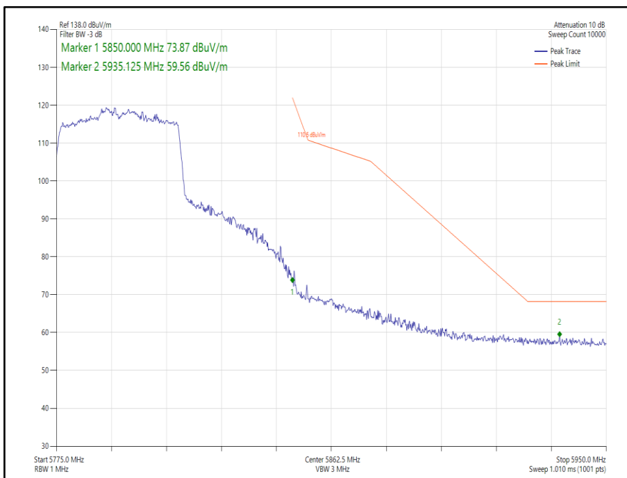
Figure 262 - 802.11ax HE40, Core 1, SU - 5795 MHz Band Edge Frequency 5850 MHz
