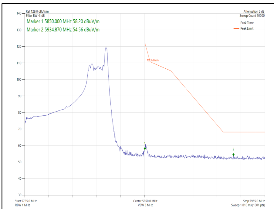
Figure 299 - 802.11ax HE80 Core 1 26-36 - 5775 MHz Band Edge Frequency 5850 MHz
