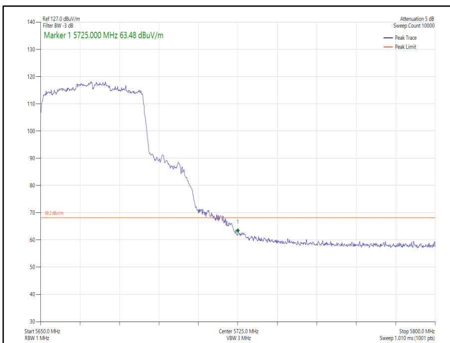
Figure 274 - 802.11ax HE40 SDM, Cores 0-1, SU - 5670 MHz Band Edge Frequency 5725 MHz
