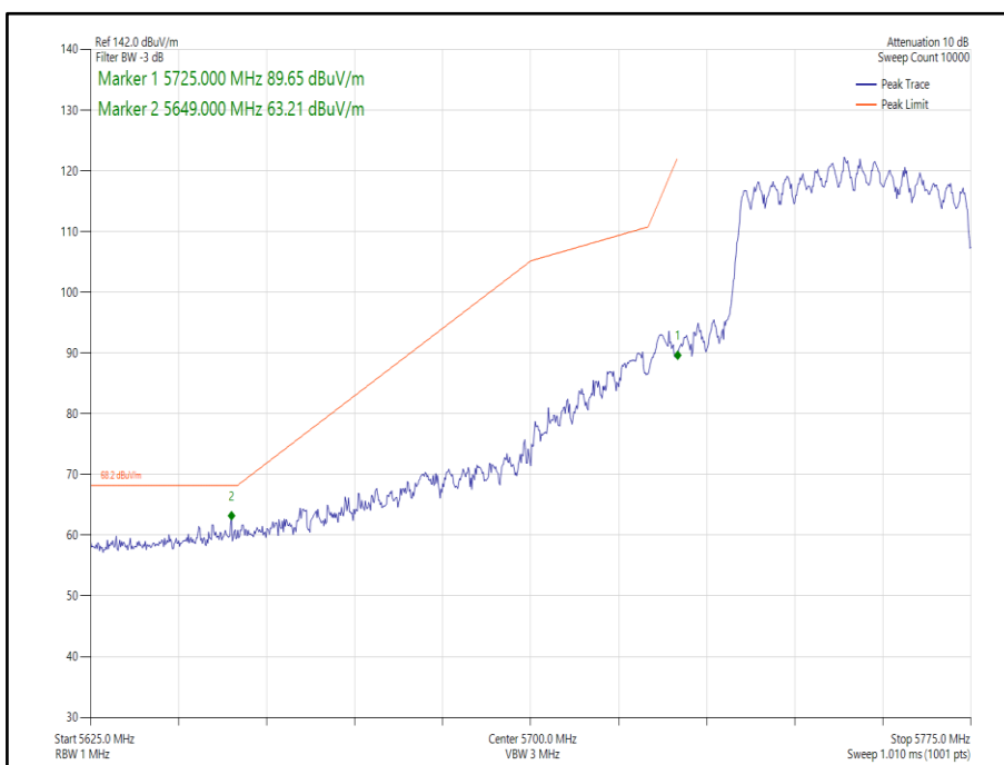
Figure 278 - 802.11ax HE40 CDD, Cores 0-1, SU - 5755 MHz Band Edge Frequency 5725 MHz
