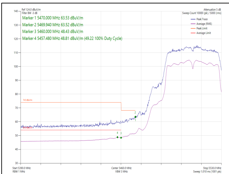
Figure 265 - 802.11n HT40 SDM, Cores 0-1 - 5510 MHz Band Edge Frequency 5470 MHz
