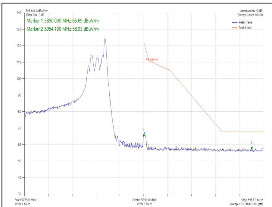
Figure 321 - 802.11ax HE80 CDD, Cores 0-1, 2d 6-36 - 5775 MHz Band Edge Frequency 5850 MHz
