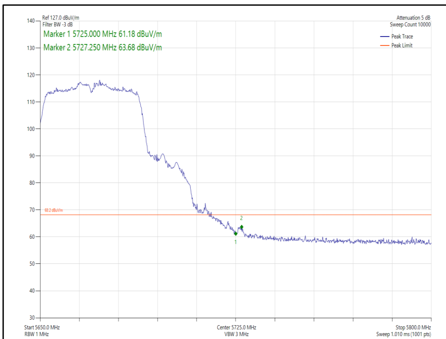
Figure 271 - 802.11n HT40 SDM, Cores 0-1 - 5670 MHz Band Edge Frequency 5725 MHz
