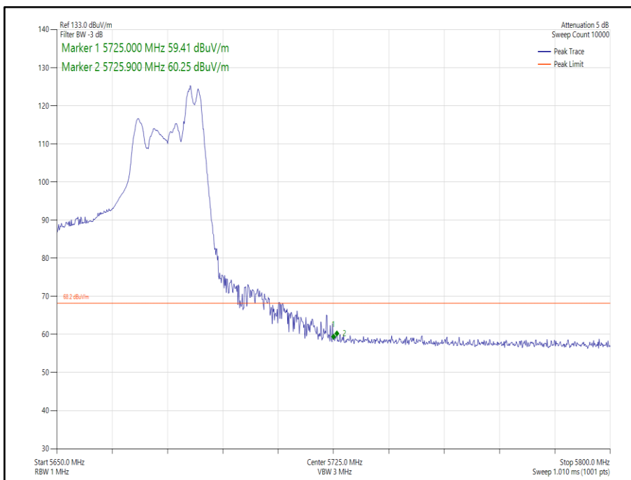
Figure 275 - 802.11ax HE40 SDM, Cores 0-1, 52-44 - 5670 MHz Band Edge Frequency 5725 MHz
