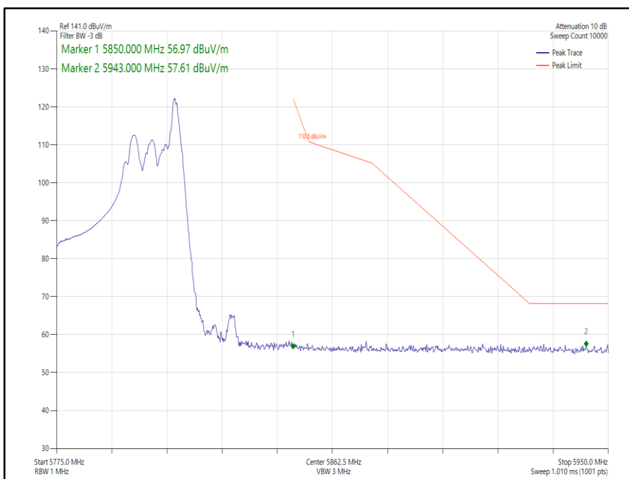
Figure 285 - 802.11ax HE40 CDD, Cores 0-1, 26-17 - 5795 MHz Band Edge Frequency 5850 MHz
