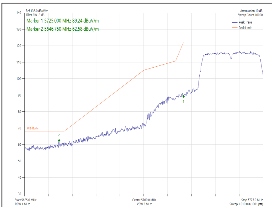
Figure 258 - 802.11n HT40, Core 1 - 5755 MHz Band Edge Frequency 5725 MHz
