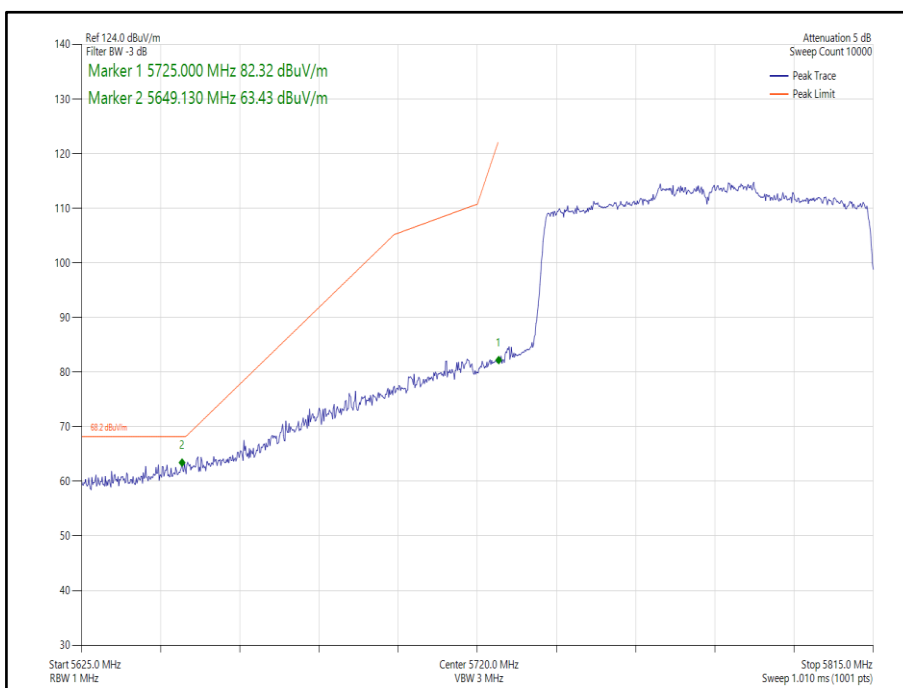
Figure 295 - 802.11ax HE80 Core 1 SU - 5775 MHz Band Edge Frequency 5725 MHz
