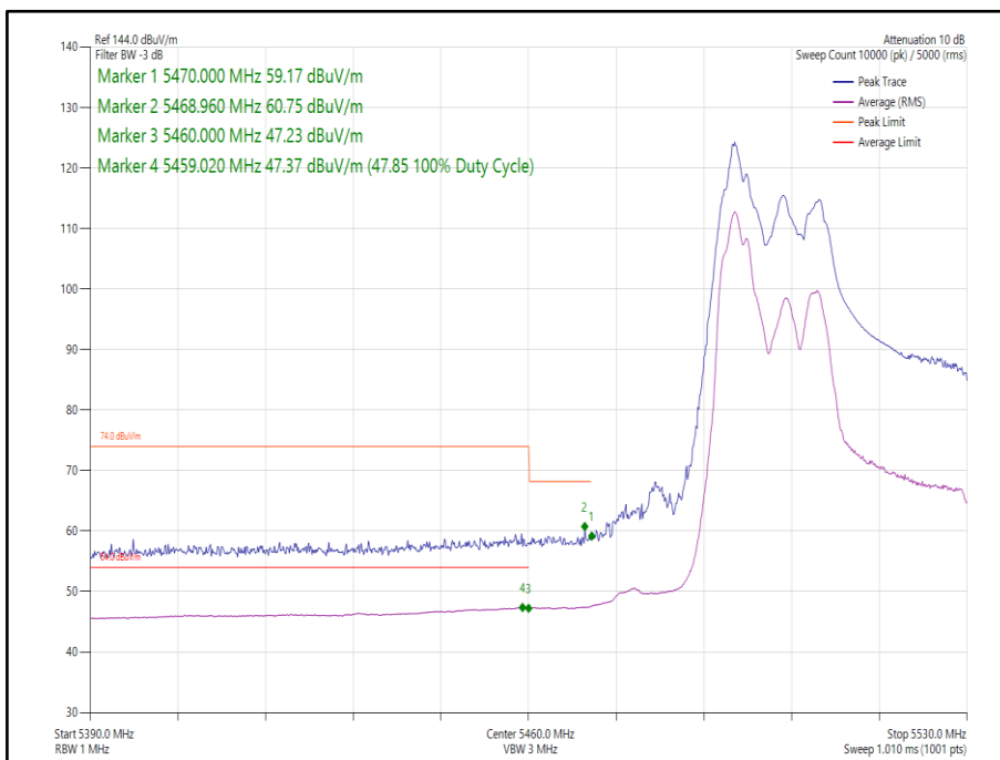
Figure 267 - 802.11ax HE40 CDD, Cores 0-1, 52-37 - 5510 MHz Band Edge Frequency 5470 MHz
