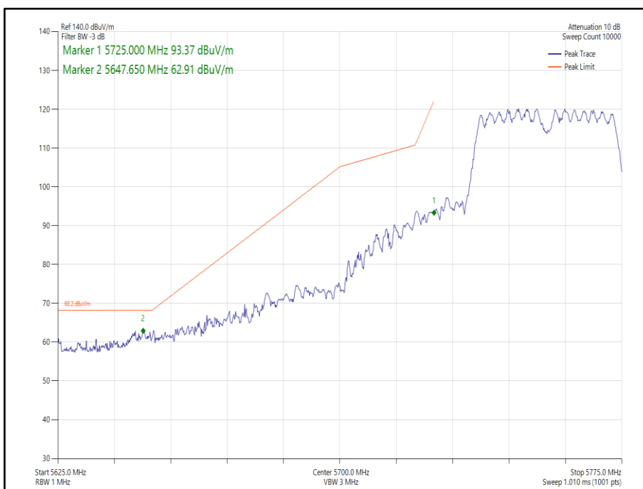
Figure 276 - 802.11n HT40 CDD, Cores 0-1 - 5755 MHz Band Edge Frequency 5725 MHz
