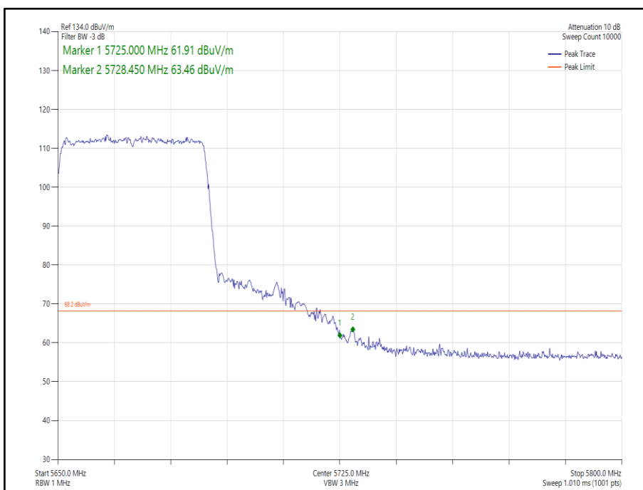
Figure 256 - 802.11ax HE40, Core 1, SU - 5670 MHz Band Edge Frequency 5725 MHz
