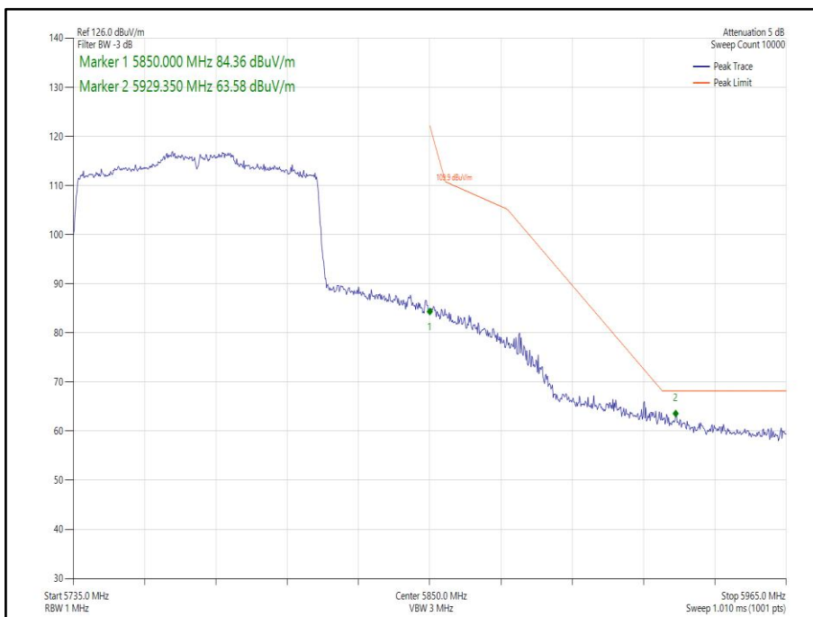
Figure 298 - 802.11ax HE80 Core 1 SU - 5775 MHz Band Edge Frequency 5850 MHz
