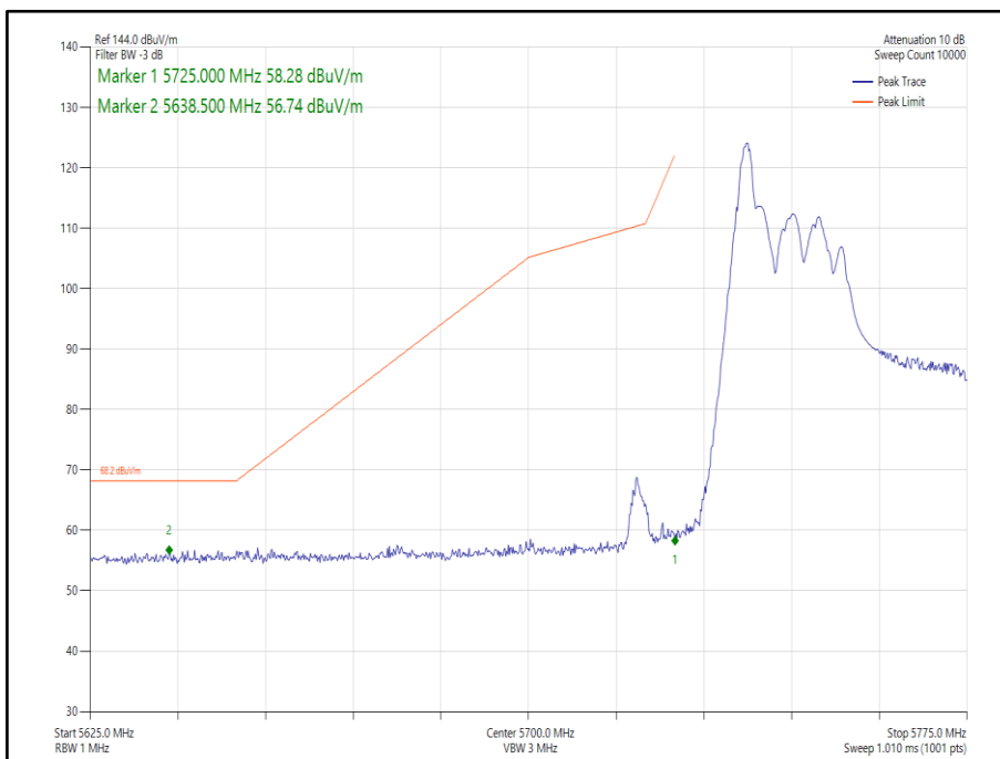
Figure 279 - 802.11ax HE40 CDD, Cores 0-1, 26-0 - 5755 MHz Band Edge Frequency 5725 MHz
