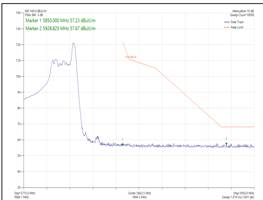
Figure 263 - 802.11ax HE40, Core 1, 26-17 - 5795 MHz Band Edge Frequency 5850 MHz
