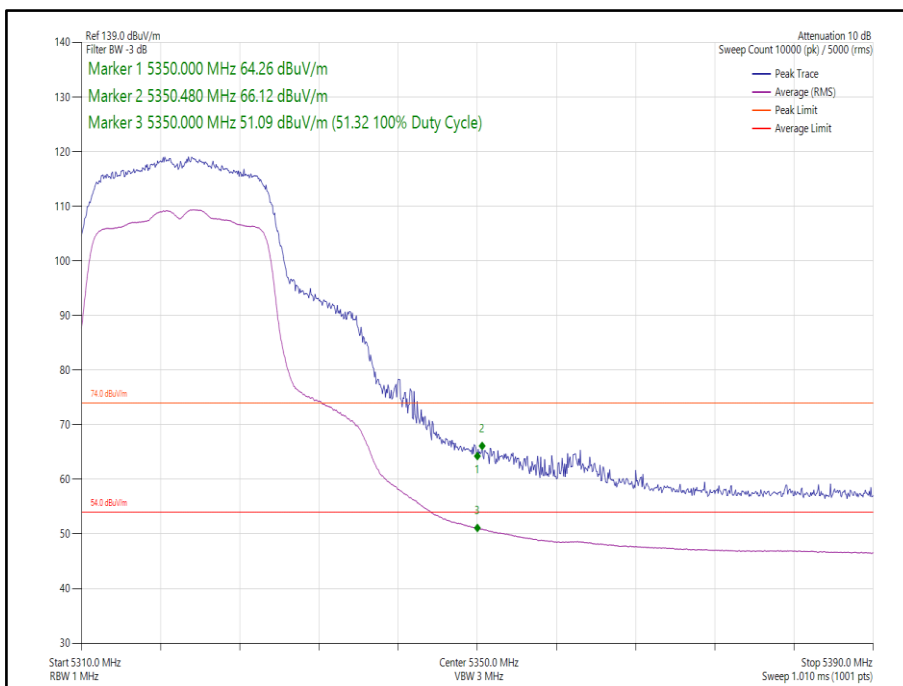
Figure 6 - 802.11n HT20, Core 0 - 5320 MHz, Band Edge Frequency 5350 MHz
