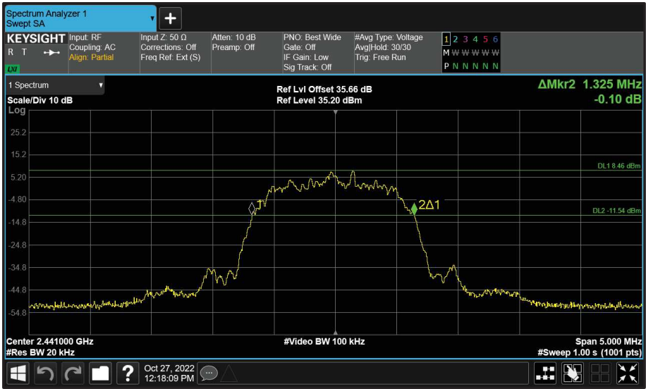
Figure 63 - Core 0 (A) 2441 MHz (CH39) 20 dB Bandwidth
