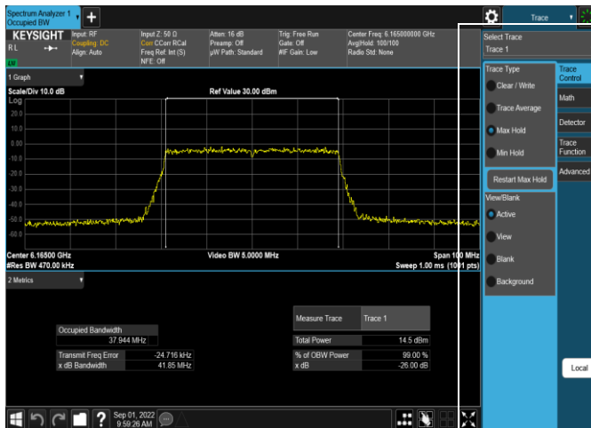
Plot 7-72. 26dB & 99% Bandwidth Plot Antenna 4a (40MHz 802.11ax RU484 (UNII Band 5) – Ch. 43)
