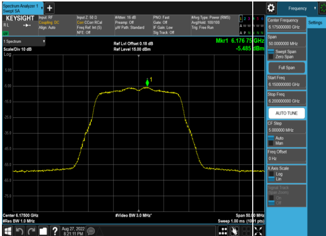
Plot 7-205. Power Spectral Density Plot Antenna 4a (20MHz 802.11a (UNII Band 5) – Ch. 45, MCS4)
