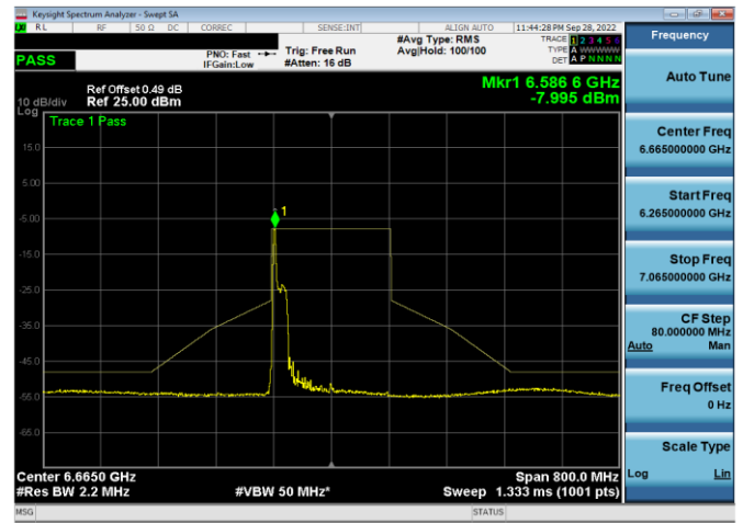
Plot 7-601. In-Band Emission Plot SDM Antenna 5b (160MHz 802.11x RU26 (UNII Band 7) – Ch. 143)
