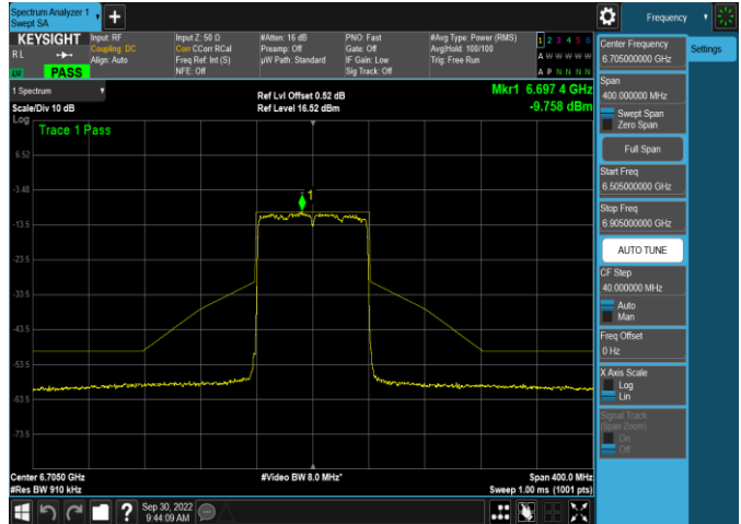
Plot 7-600. In-Band Emission Plot SDM Antenna 4a (80MHz 802.11x RU996 (UNII Band 7) – Ch. 151)
