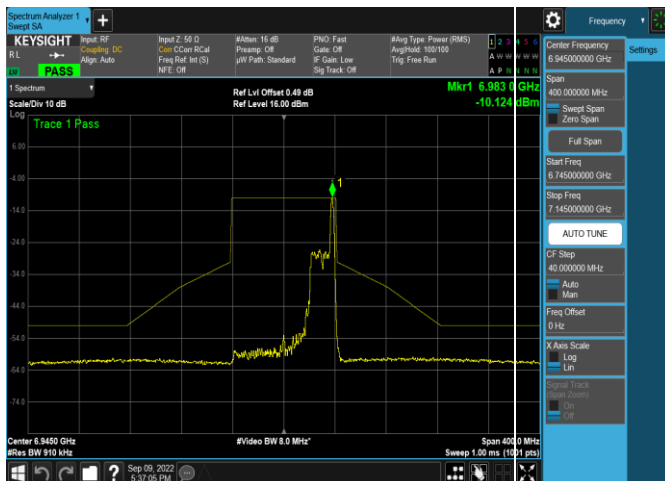
Plot 7-629. In-Band Emission Plot SDM Antenna 5b (80MHz 802.11ax RU26 (UNII Band 8) – Ch. 199)
