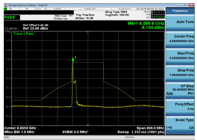
Plot 7-602. In-Band Emission Plot SDM Antenna 4a (160MHz 802.11x RU26 (UNII Band 7) – Ch. 143)
