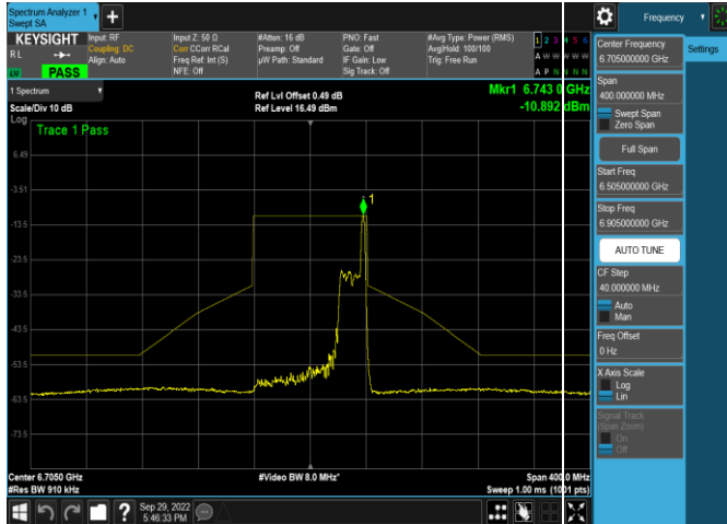
Plot 7-597. In-Band Emission Plot SDM Antenna 5b (80MHz 802.11x RU26 (UNII Band 7) – Ch. 151)
