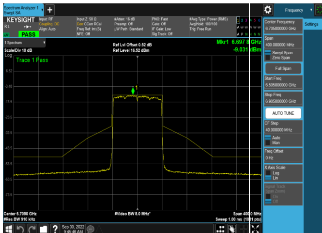
Plot 7-599. In-Band Emission Plot SDM Antenna 5b (80MHz 802.11x RU996 (UNII Band 7) – Ch. 151)
