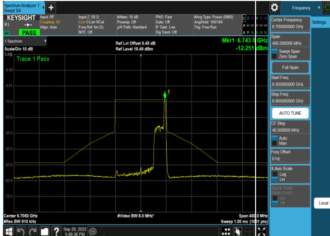
Plot 7-598. In-Band Emission Plot SDM Antenna 4a (80MHz 802.11x RU26 (UNII Band 7) – Ch. 151)
