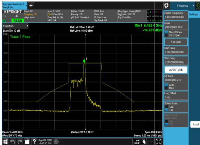
Plot 7-556. In-Band Emission Plot SDM Antenna 4a (40MHz 802.11ax RU26 (UNII Band 6) – Ch. 107)
