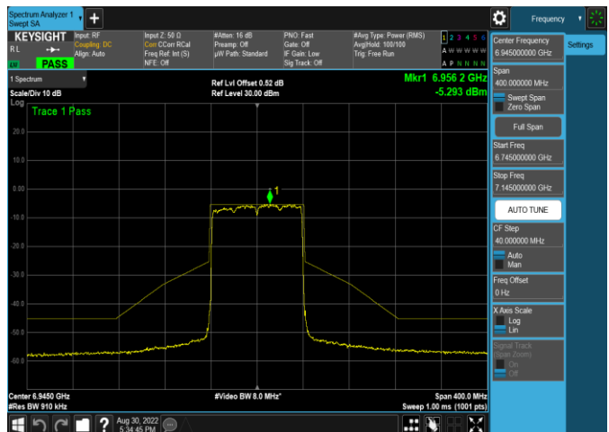
Plot 7-444. In-Band Emission Plot Antenna 5b (80MHz 802.11ax RU96 (UNII Band 8) – Ch. 199)
