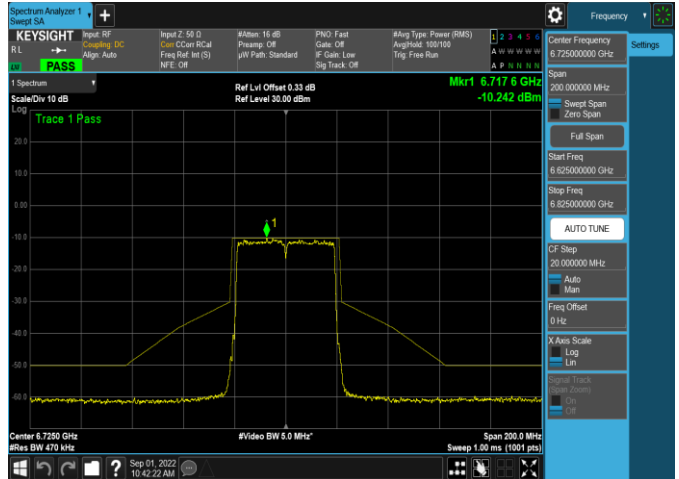
Plot 7-488. In-Band Emission Plot Antenna 4a (40MHz 802.11ax RU84 (UNII Band 7) – Ch. 155)
