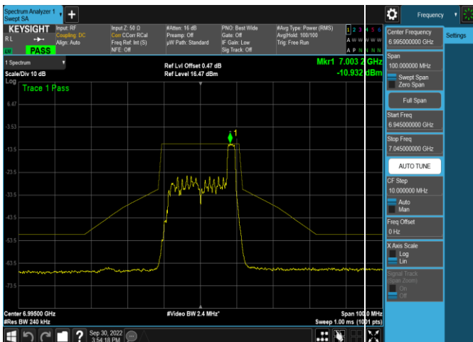
Plot 7-435. In-Band Emission Plot Antenna 5b (20MHz 802.11ax RU26 (UNII Band 8) – Ch. 209)
