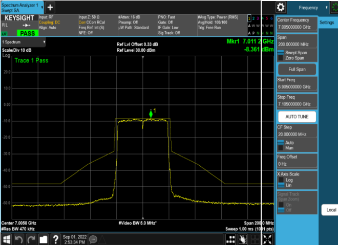
Plot 7-440. In-Band Emission Plot Antenna 5b (40MHz 802.11ax RU48 (UNII Band 8) – Ch. 211)
