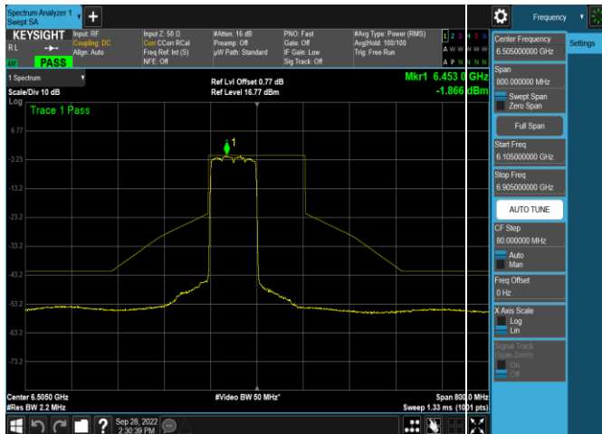
Plot 7-480. In-Band Emission Plot Antenna 4a (160MHz 802.11ax RU996x2 (UNII Band 6) – Ch. 111)
