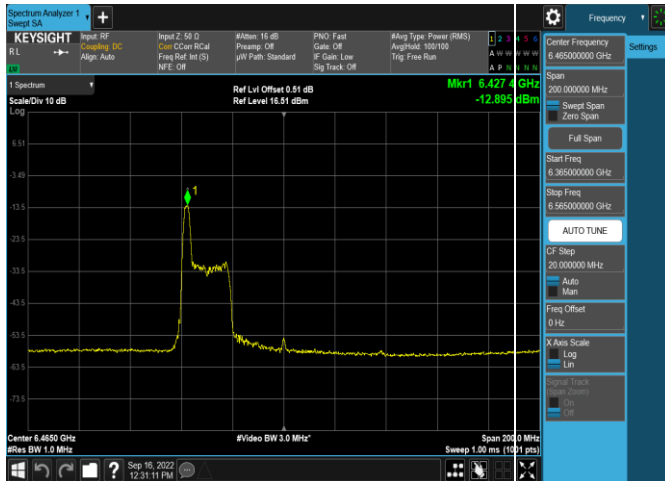
Plot 7-305. Power Spectral Density Plot SDM Antenna 5b (80MHz 802.11ax RU26 (UNII Band 6) – Ch. 103)
