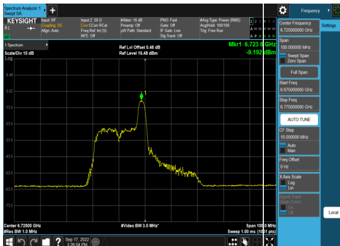
Plot 7-331. Power Spectral Density Plot SDM Antenna 5b (40MHz 802.11ax RU26 (UNII Band 7) – Ch. 155)
