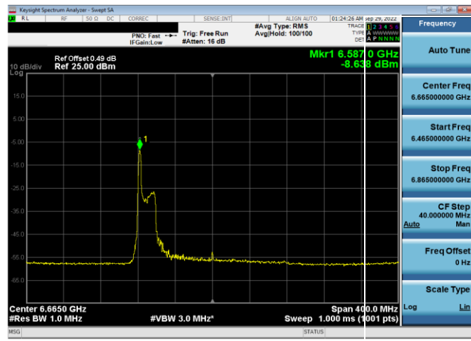
Plot 7-237. Power Spectral Density Plot Antenna 4a (160MHz 802.11ax RU26 (UNII Band 7) – Ch. 143)
