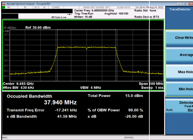
Plot 7-28. 26dB & 99% Bandwidth Plot Antenna 5b (40MHz 802.11ax (UNII Band 6) – Ch. 107, MCS4)
