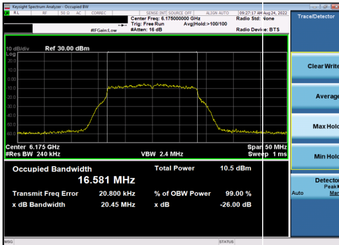
Plot 7-21. 26dB & 99% Bandwidth Plot Antenna 5b (20MHz 802.11a (UNII Band 5) – Ch. 45, MCS4)
