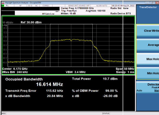
Plot 7-1. 26dB & 99% Bandwidth Plot Antenna 5b (20MHz 802.11a (UNII Band 5) – Ch. 45, MCS2)
