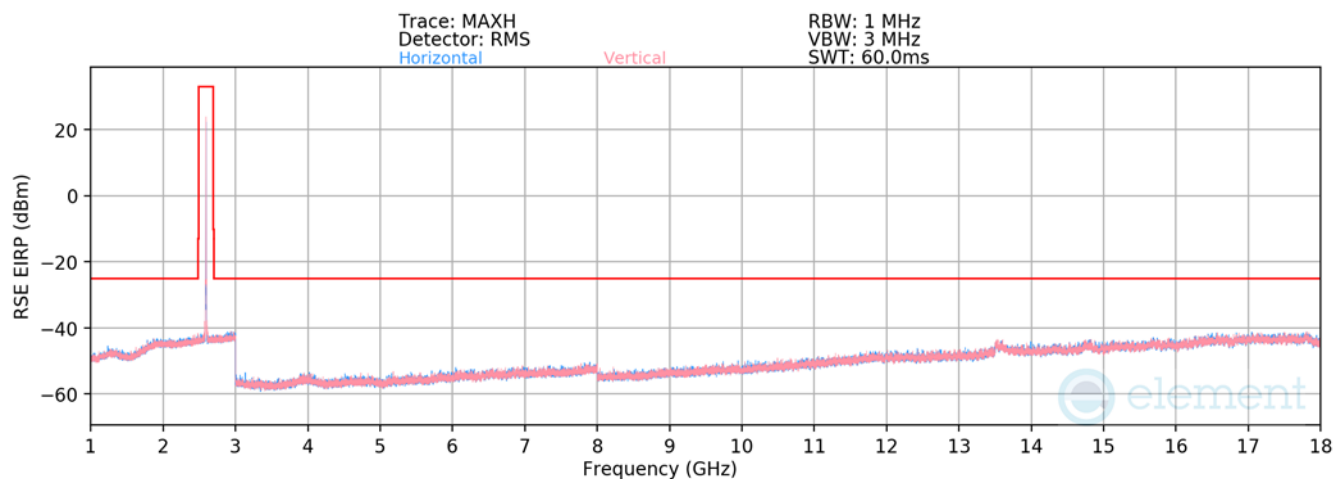
Plot 7-314. Antenna 1 Radiated Spurious Plot 1GHz – 18GHz (LTE Band 7)
