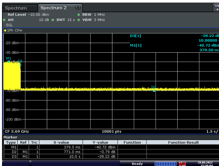
Plot 7-99. Run#1 End User Device Discontinues Operations within 10s
