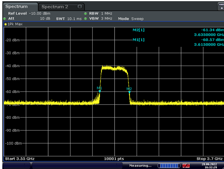
Plot 7-100. Run#2 End User Device Frequency of Operations
