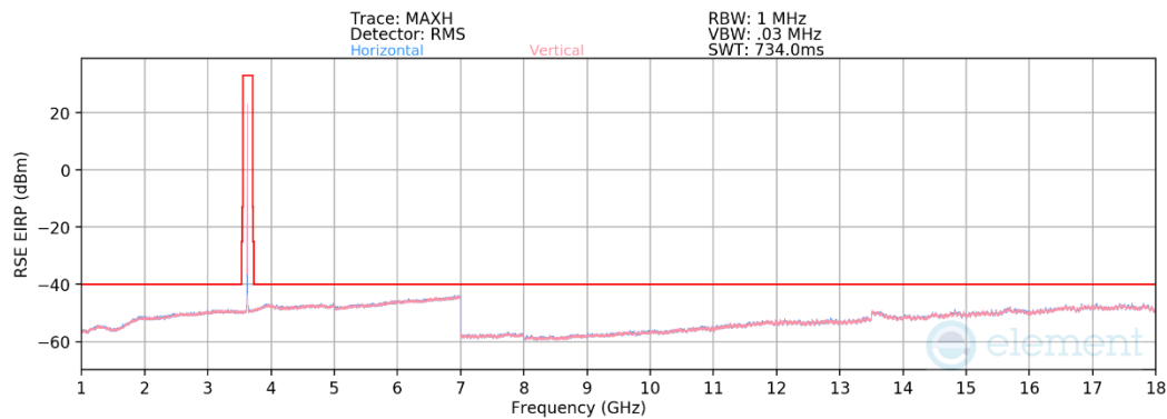
Plot 7-88. Radiated Spurious Plot 1 – 18GHz (LTE Band 48)
