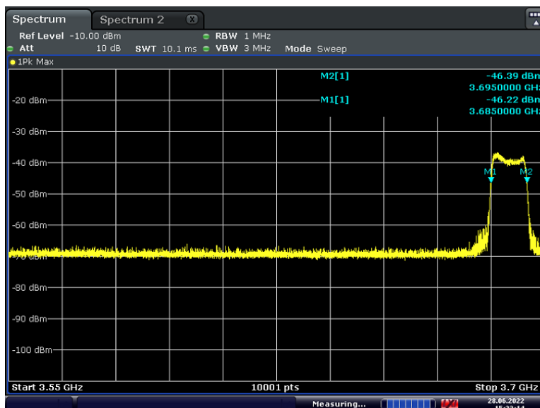
Plot 7-98. Run#1 End User Device Frequency of Operations
