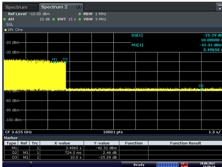
Plot 7-101. Run#2 End User Device Discontinues Operations within 10s
