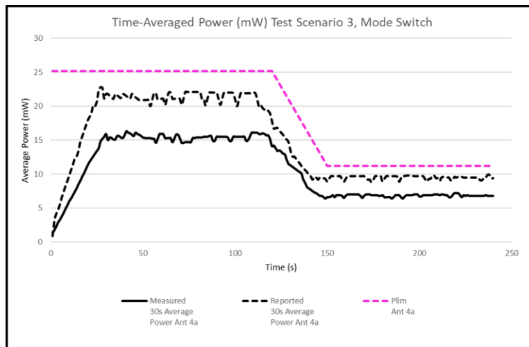
Figure J-8 30s Average Power vs. Time during Mode Switch
