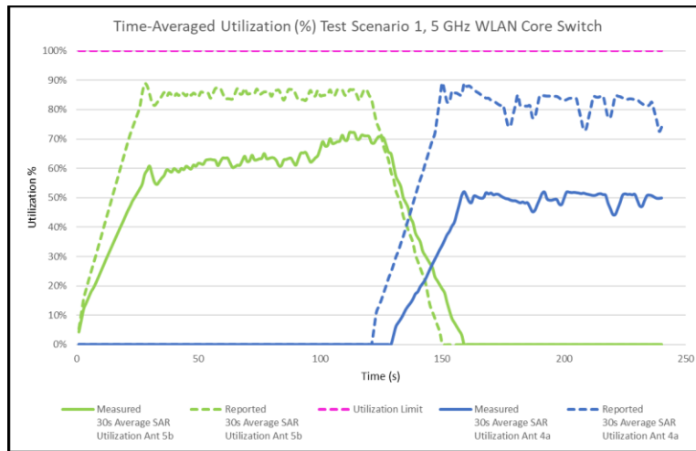
Figure J-3 30s Average SAR Utilization vs. Time, 5 GHz
